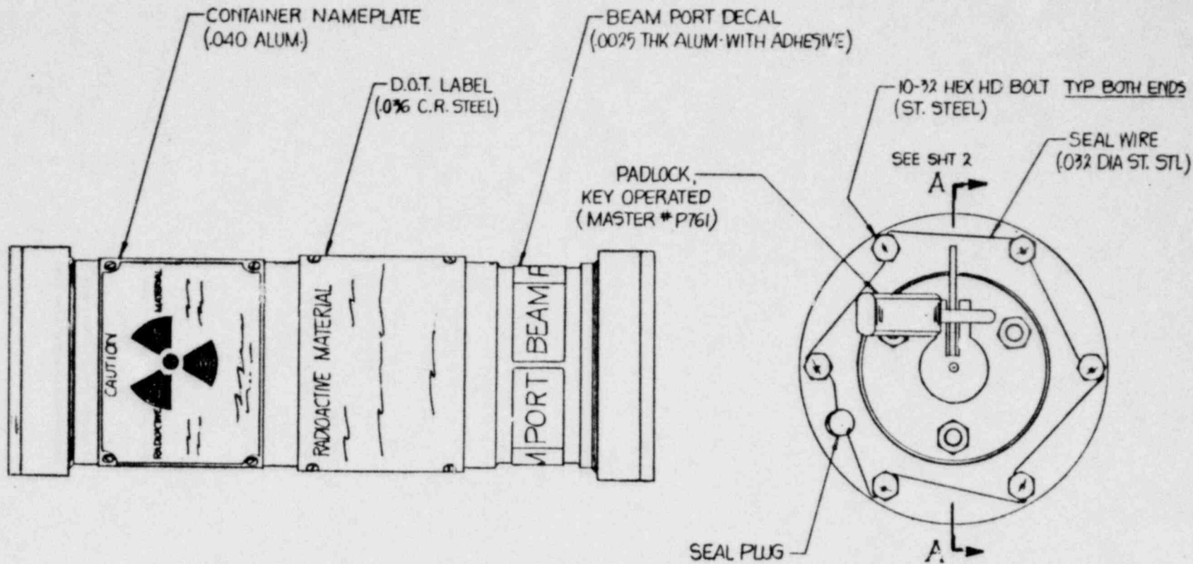
VIEW B-B (FROM SHT #2) SCALE: 3/4
