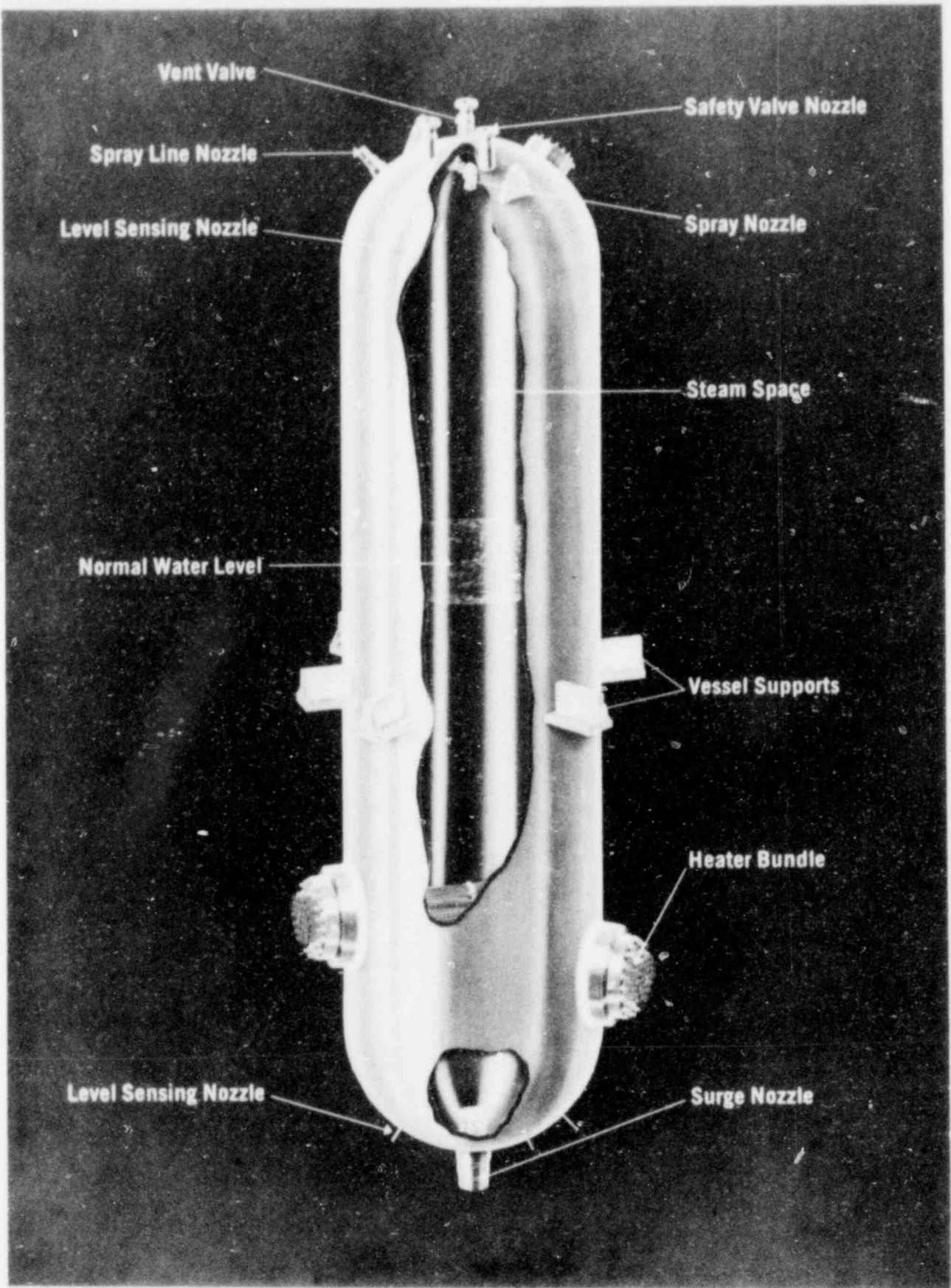
FIGURE I-12. The Pressurizer
