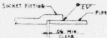
DETAIL - 'E'
