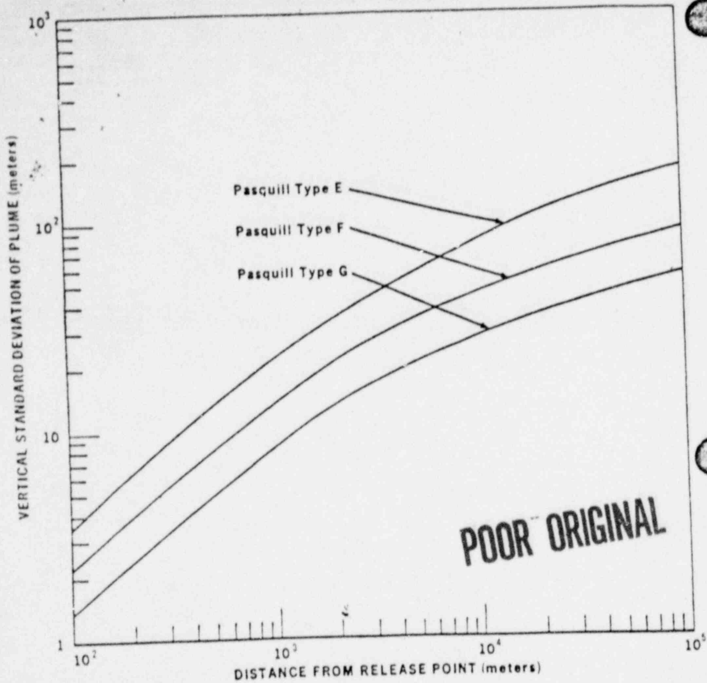
Figure 2. Vertical Standard Deviation of Material in a Plume
