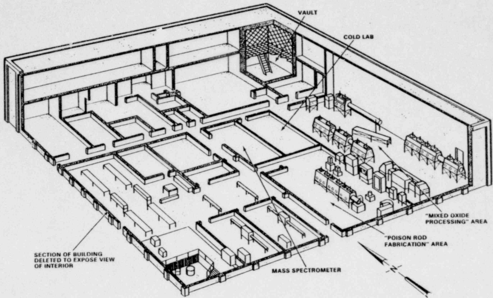
FIGURE 1. Exxon MOFP Building Arrangement for 36 kg per D 2 O Design Throughput
