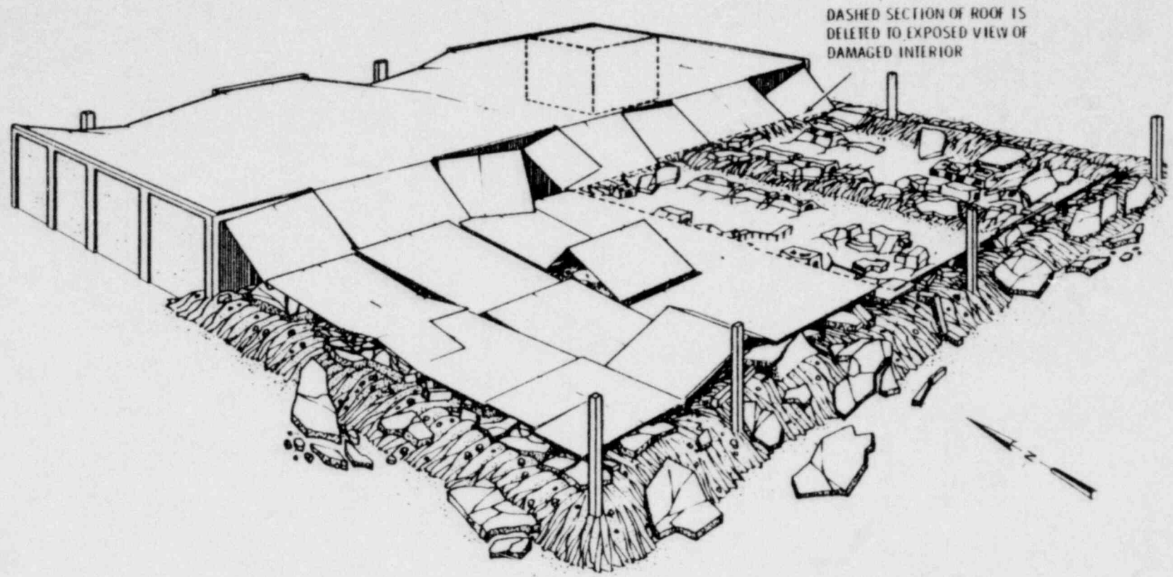
FIGURE 7. Type and Range of Damage Postulated for the MOFP at Nominal Wind Speed of 250 mph
