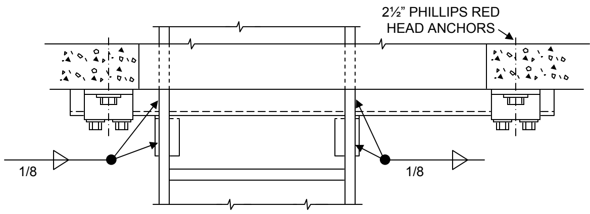
WALL PENETRATION ELEVATION
