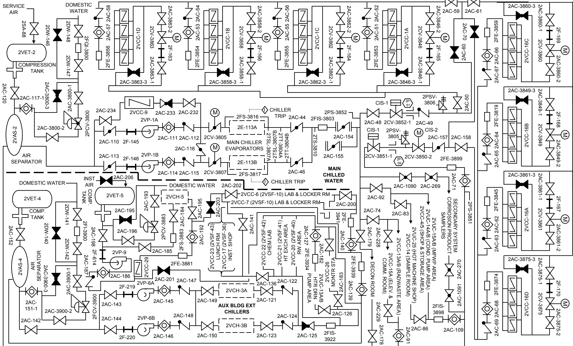
CONTAINMENT, TURBINE, AUXILIARY, AUXILIARY EXTENSION BUILDINGS AND CONTROLLED ACCESS CHILLED WATER SYSTEMS
