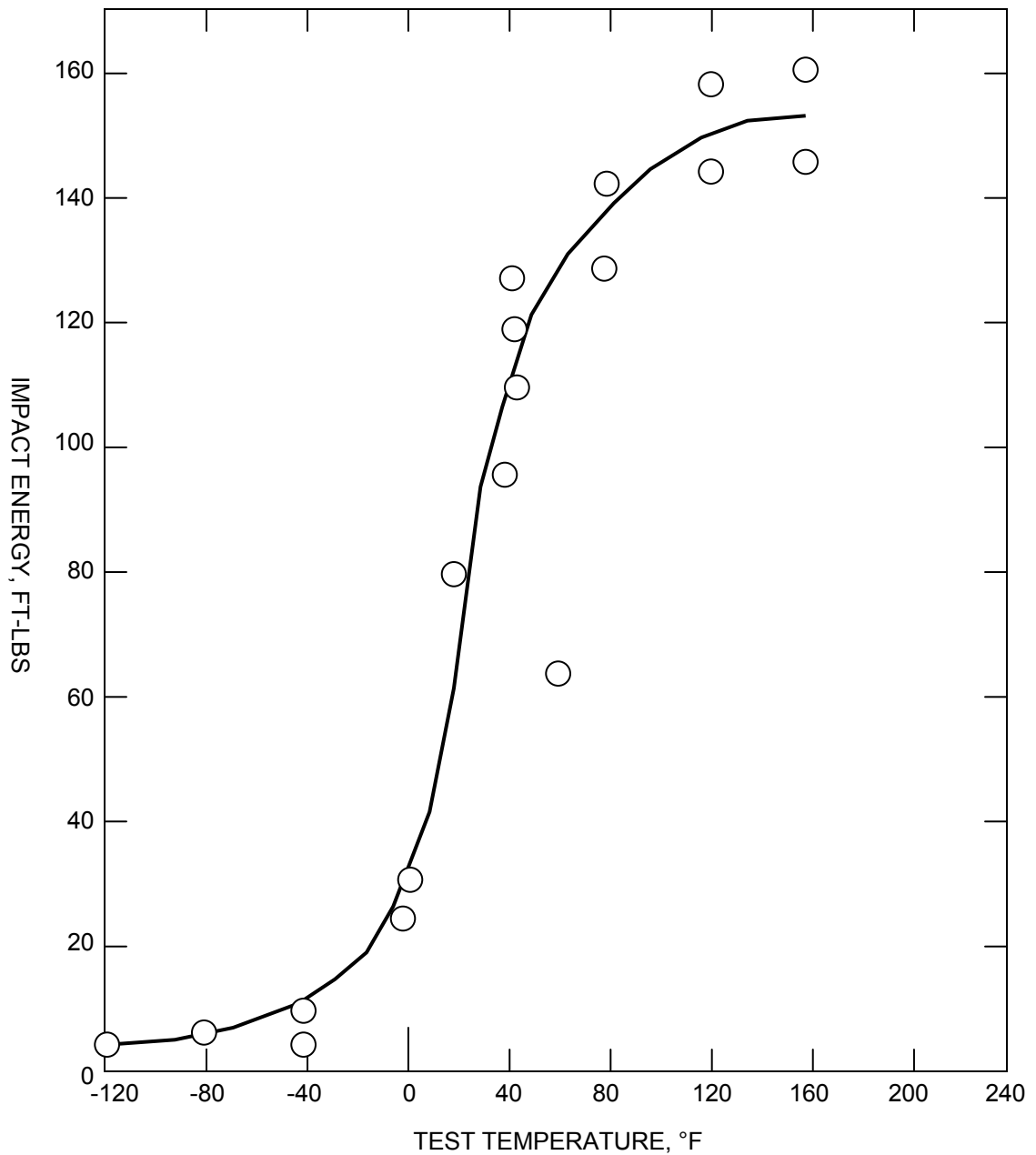
Weld Metal – Plate C-8009-1/C-8009-2 Impact Energy vs Temperature
