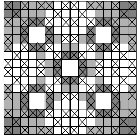
HC and GB (124 ZrB 2 Pins)
