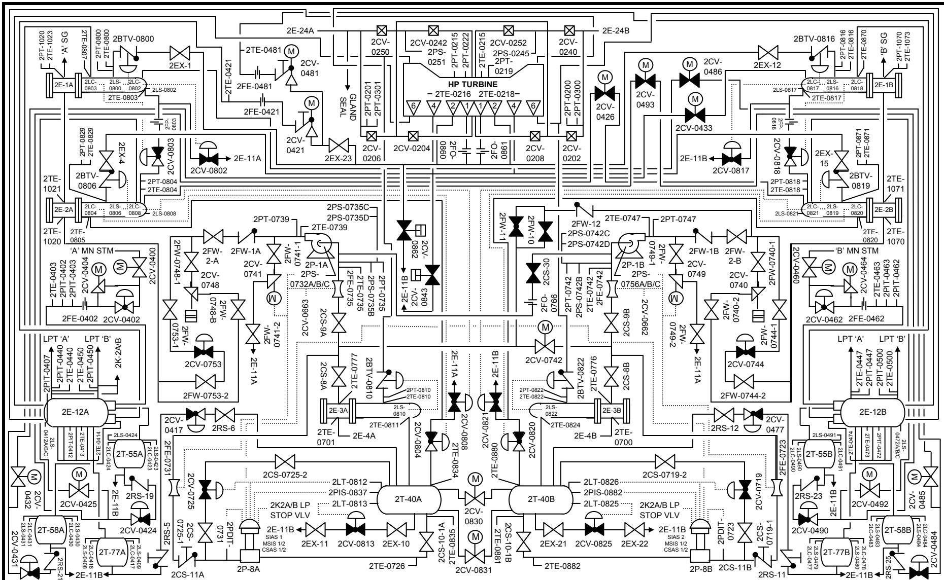
HEATER DRAINS, MAIN FEEDWATER, AND REHEAT STEAM
