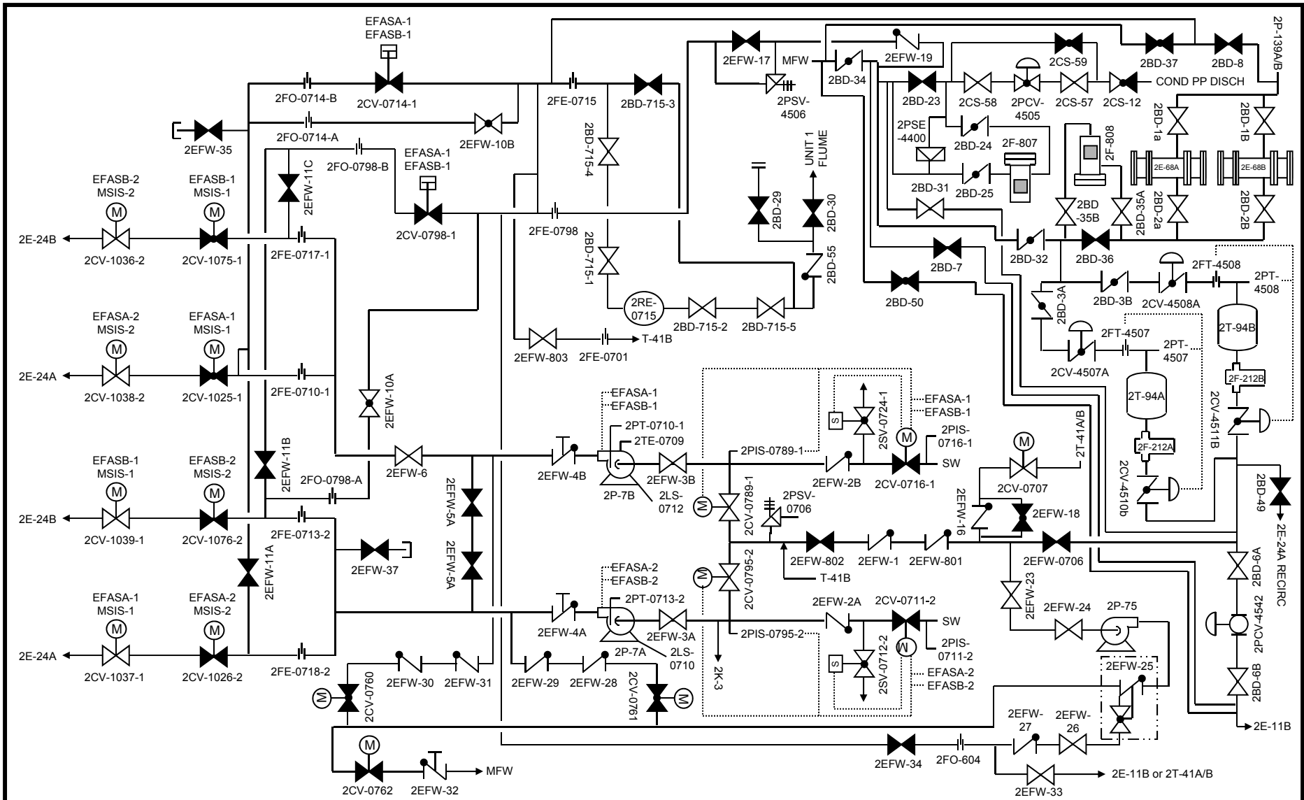
EMERGENCY AND AUXILIARY FEEDWATER, STARTUP & BLOWDOWN DEMINERALIZERS
