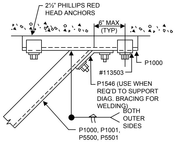
ALTERNATE B
