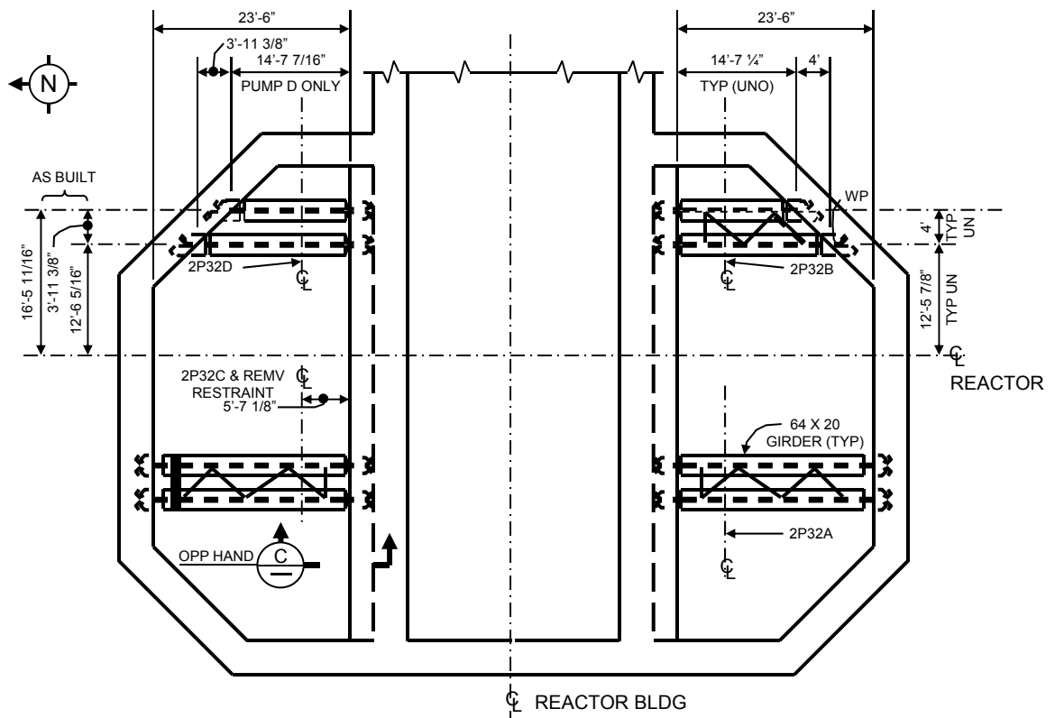
PLAN @ ELEVATION 403'-0"
