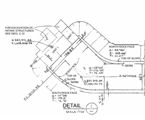
INTAKE CANAL PLAN, PROFILE & DETAILS
