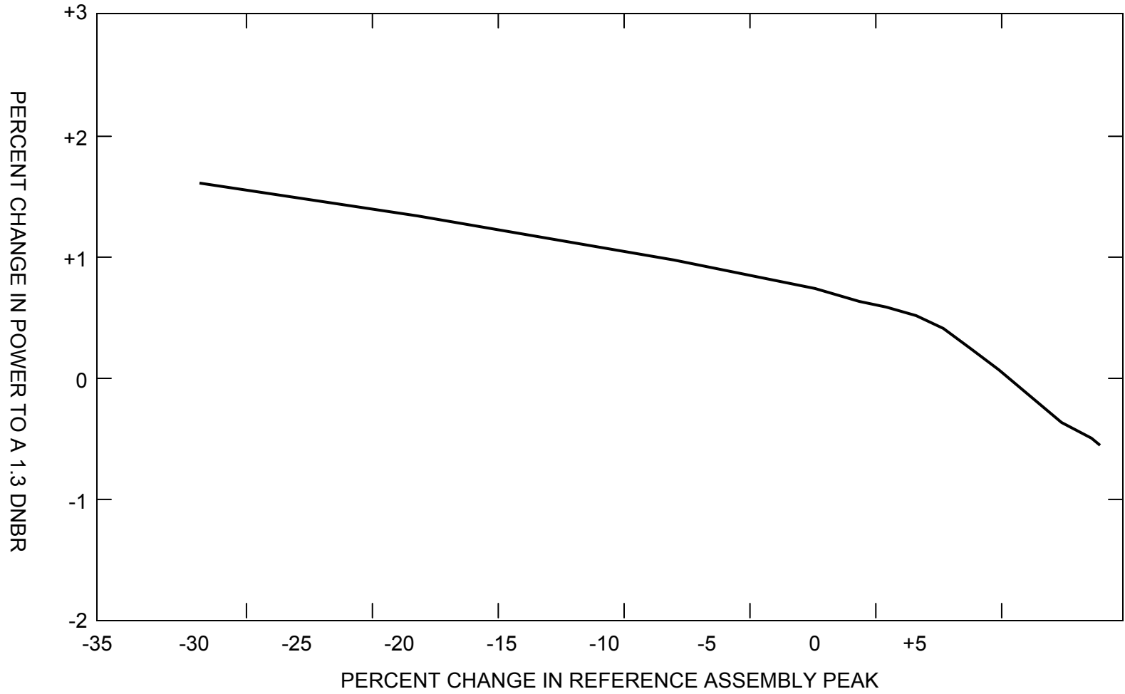
PERCENT CHANGE IN CORE POWER VS PERCENT CHANGE IN REFERENCE ASSEMBLY PEAK FROM DESIGN
