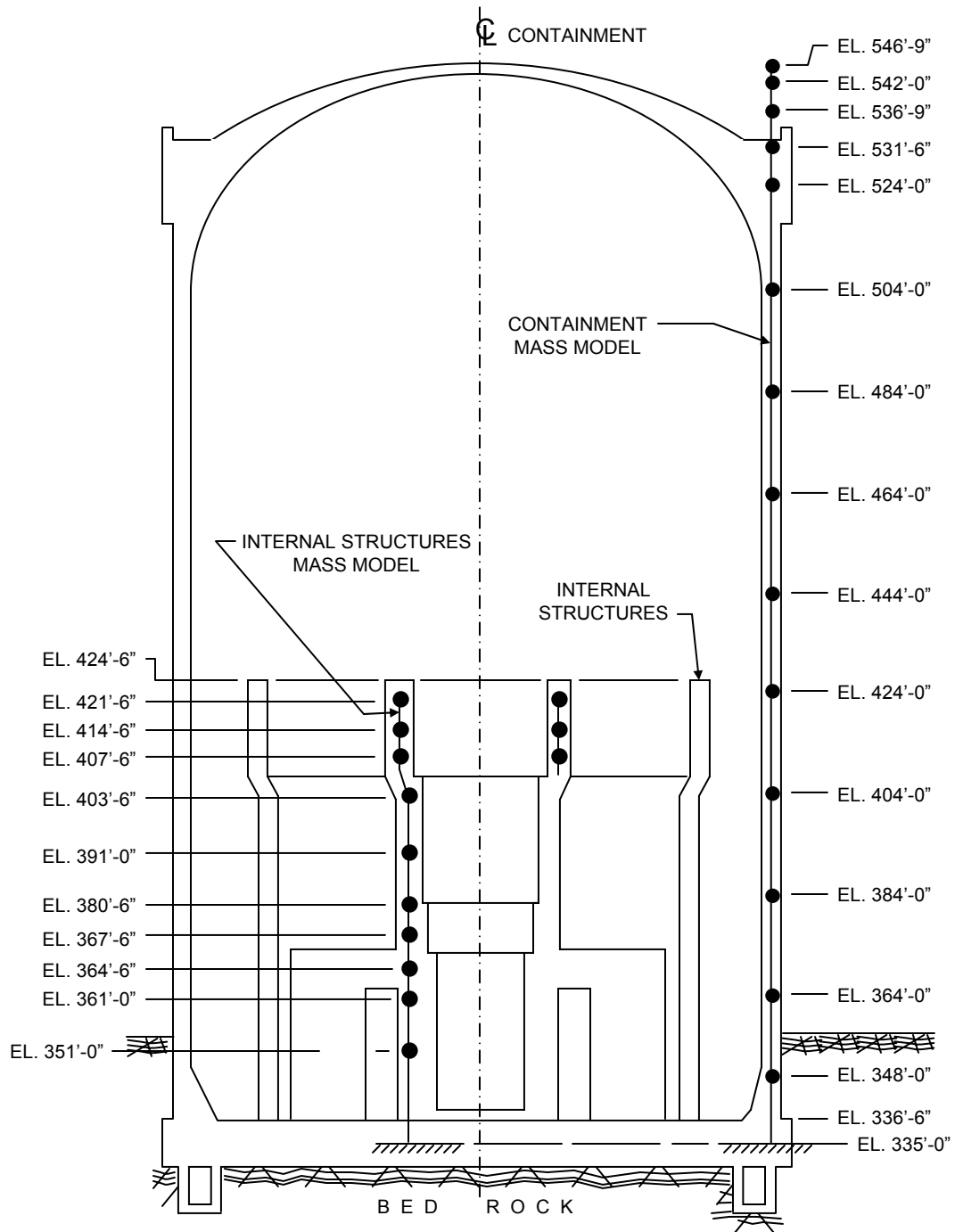
MASS MODEL NORTH SOUTH AND EAST WEST
