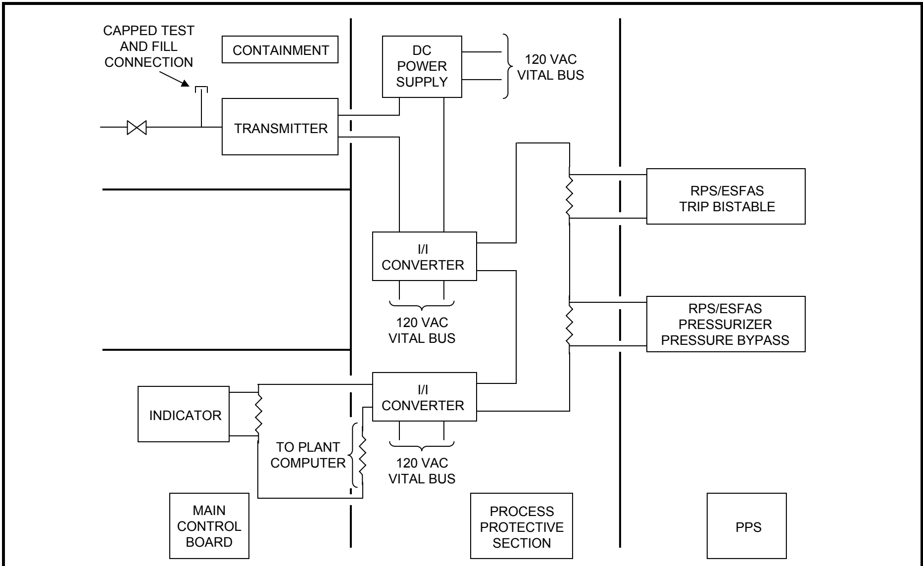
TYPICAL MEASUREMENT CHANNEL FUNCTIONAL DIAGRAM (PRESSURIZER PRESSURE) WIDE RANGE
