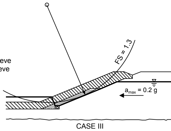
CASE III Minimum Reservoir, High Water Table & Earthquake
