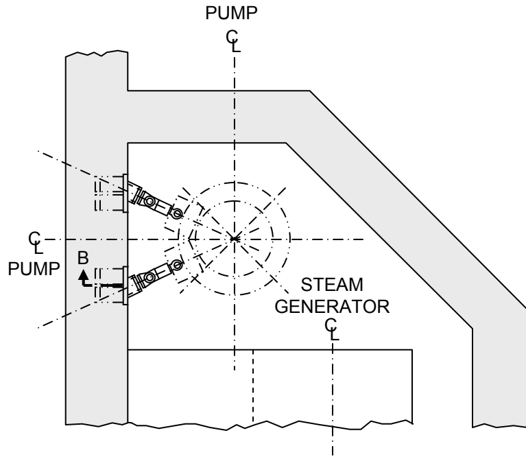
PLAN AT ELEVATION 390'-9"
