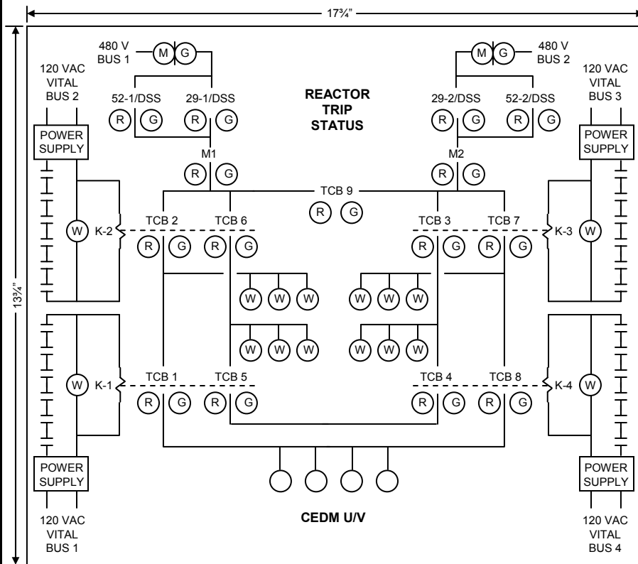
PLANT PROTECTION SYSTEM REMOTE REACTOR TRIP STATUS PANEL
