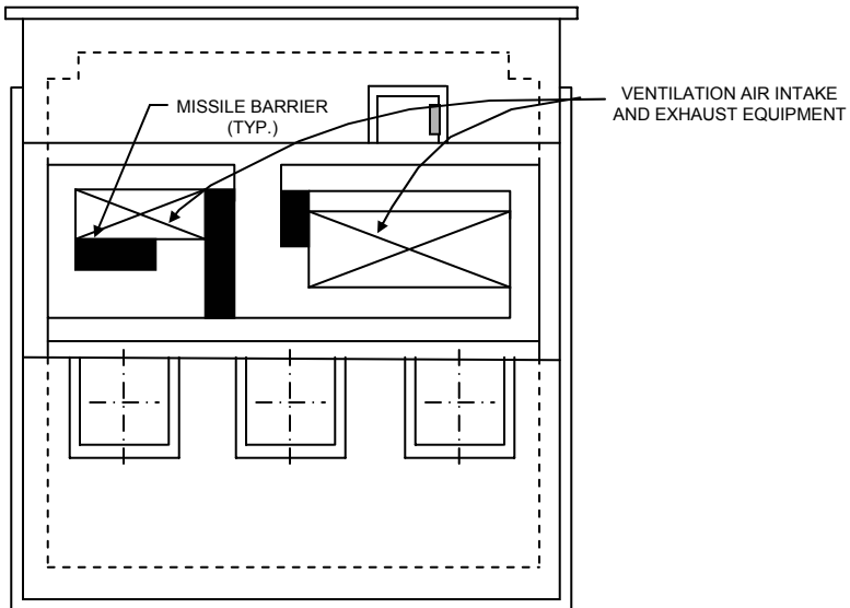
INTAKE STRUCTURE PLAN AT ELEV. 378'-0"
