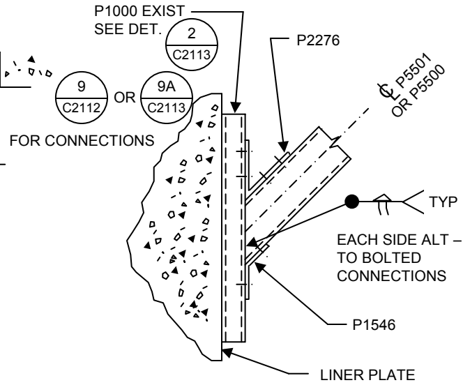
ALTERNATE D
