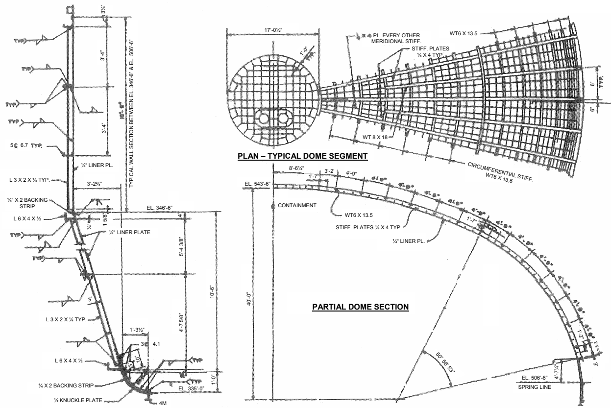
TYPICAL WALL LINER PLATE SECTION
