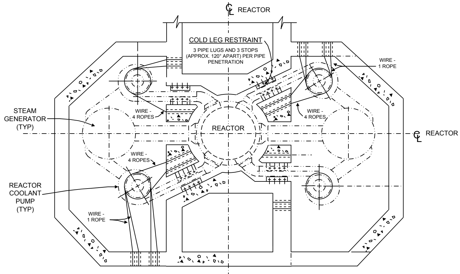
PLAN @ EL. 377' - 6"
