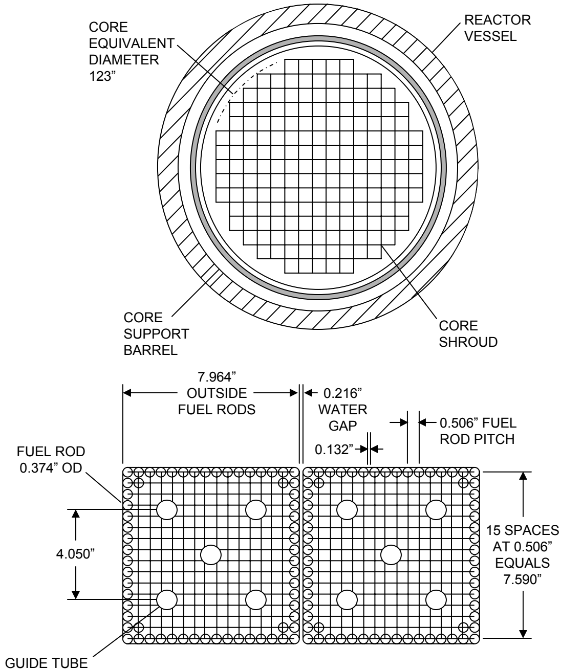
Cycle 20 Configuration Shown (NGF Design)
