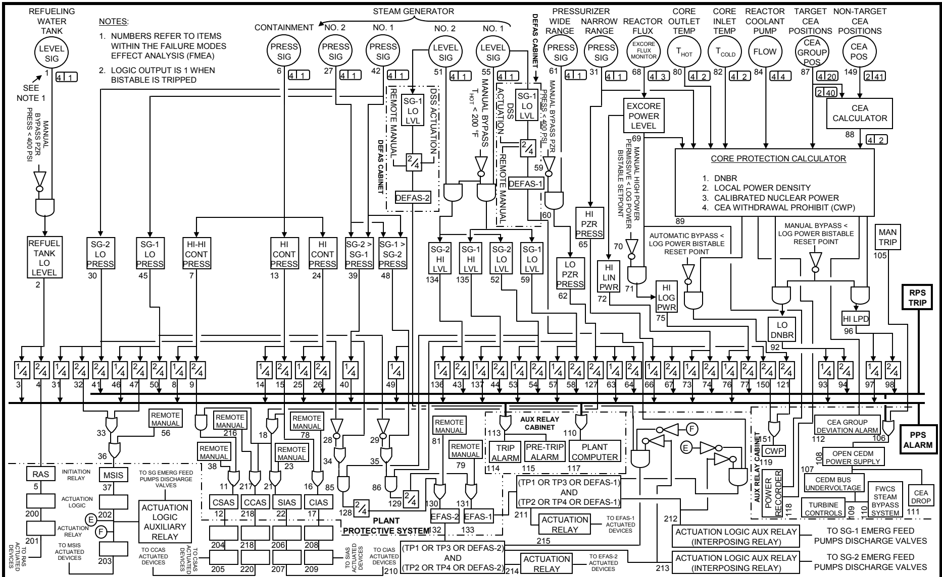
PLANT PROTECTIVE SYSTEM INTERFACE LOGIC DIAGRAM
