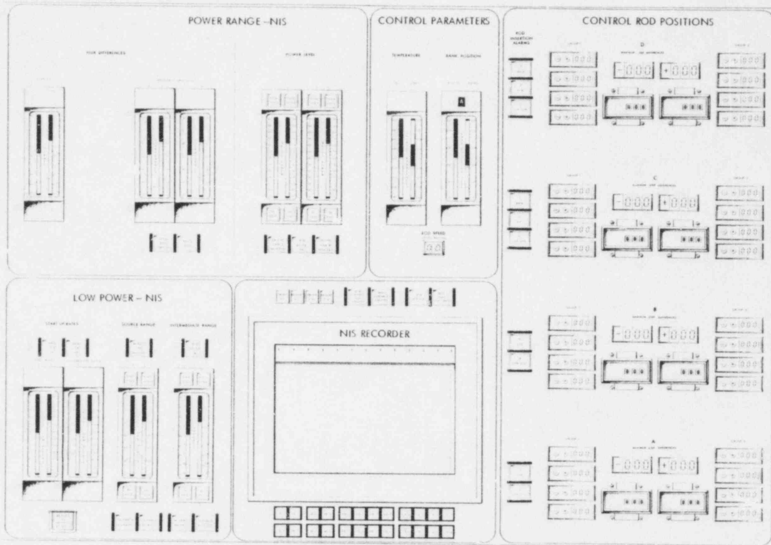
Figure 1-17. Initial arrangement of NIS and rod position indications.
