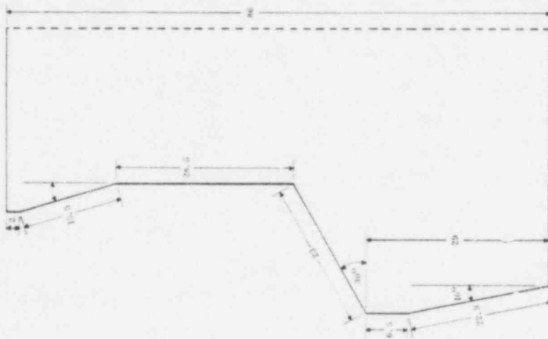
Figure 1-8. Recommended dimensions for a standup console to accommodate the 5th to 95th percentile operator population.
