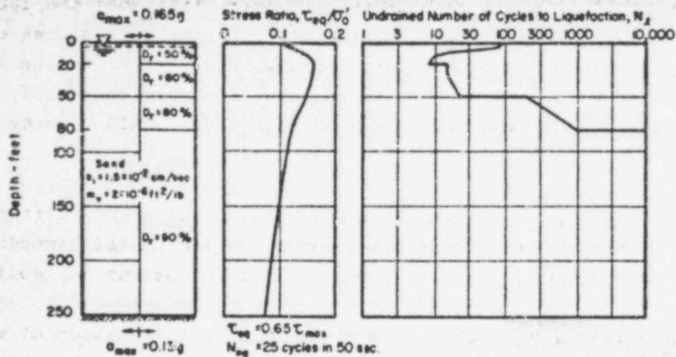
FIG. 1-3a SOIL PROFILE AND STRESS CONDITIONS USED FOR ANALYSIS
