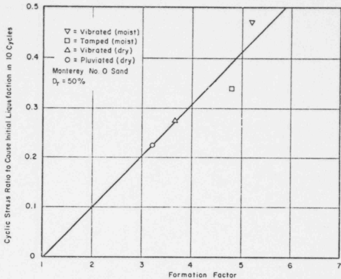
FIG. 2-10 RELATIONSHIP BETWEEN CYCLIC STRESS RATIO AND FORMATION FACTOR
