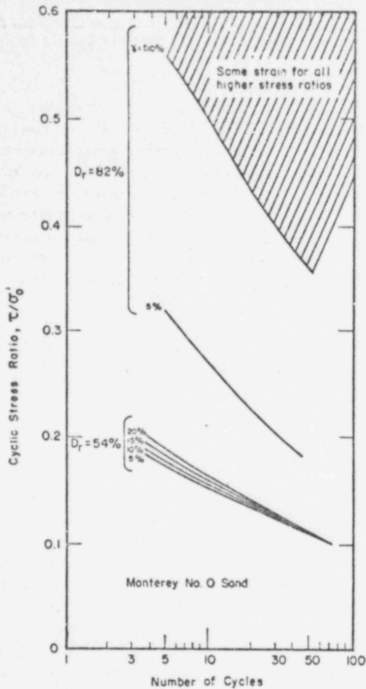
FIG. 5-1 RELATIONSHIP BETWEEN \tau/\sigma'_0 AND NUMBER OF CYCLES CAUSING DIFFERENT STRAIN LEVELS
