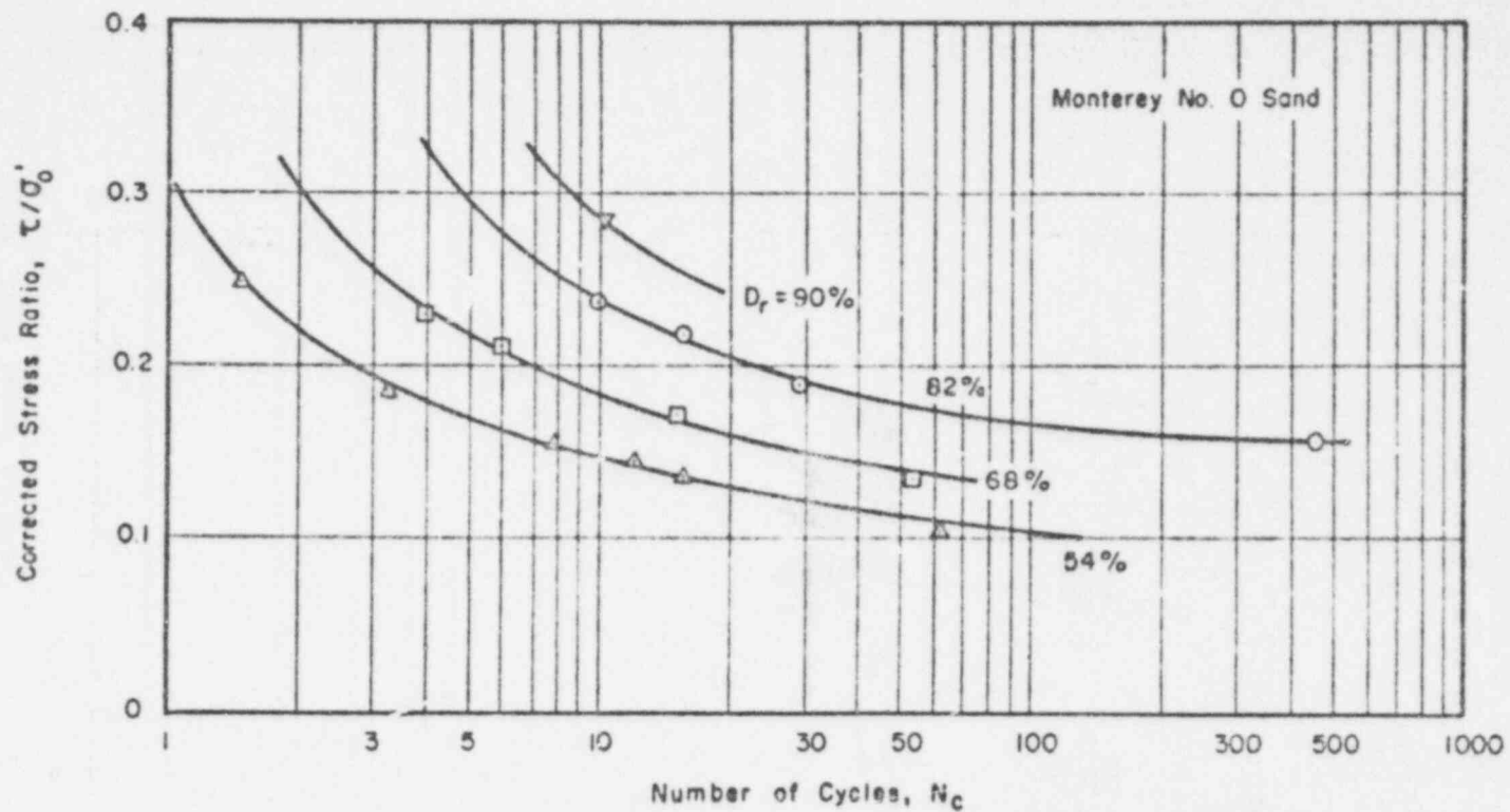
FIG. 3-1 CORRECTED \tau/\sigma'_0 VS N_c FOR INITIAL LIQUEFACTION
