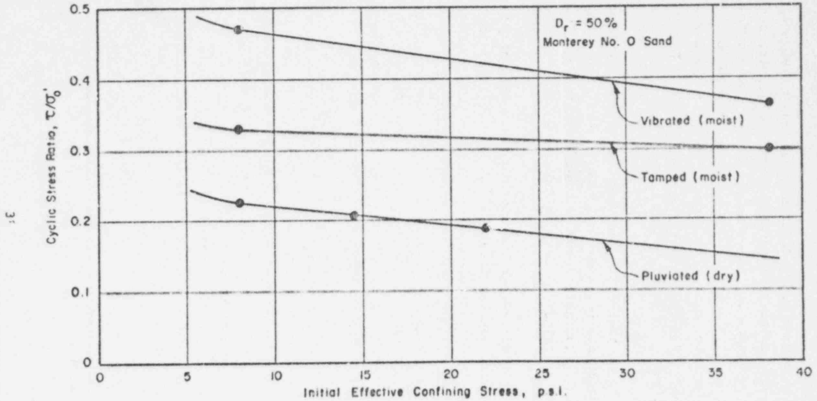
FIG. 2-8 CYCLIC STRESS RATIO AT 10 CYCLES FOR INITIAL LIQUEFACTION VS INITIAL EFFECTIVE CONFINING STRESS
