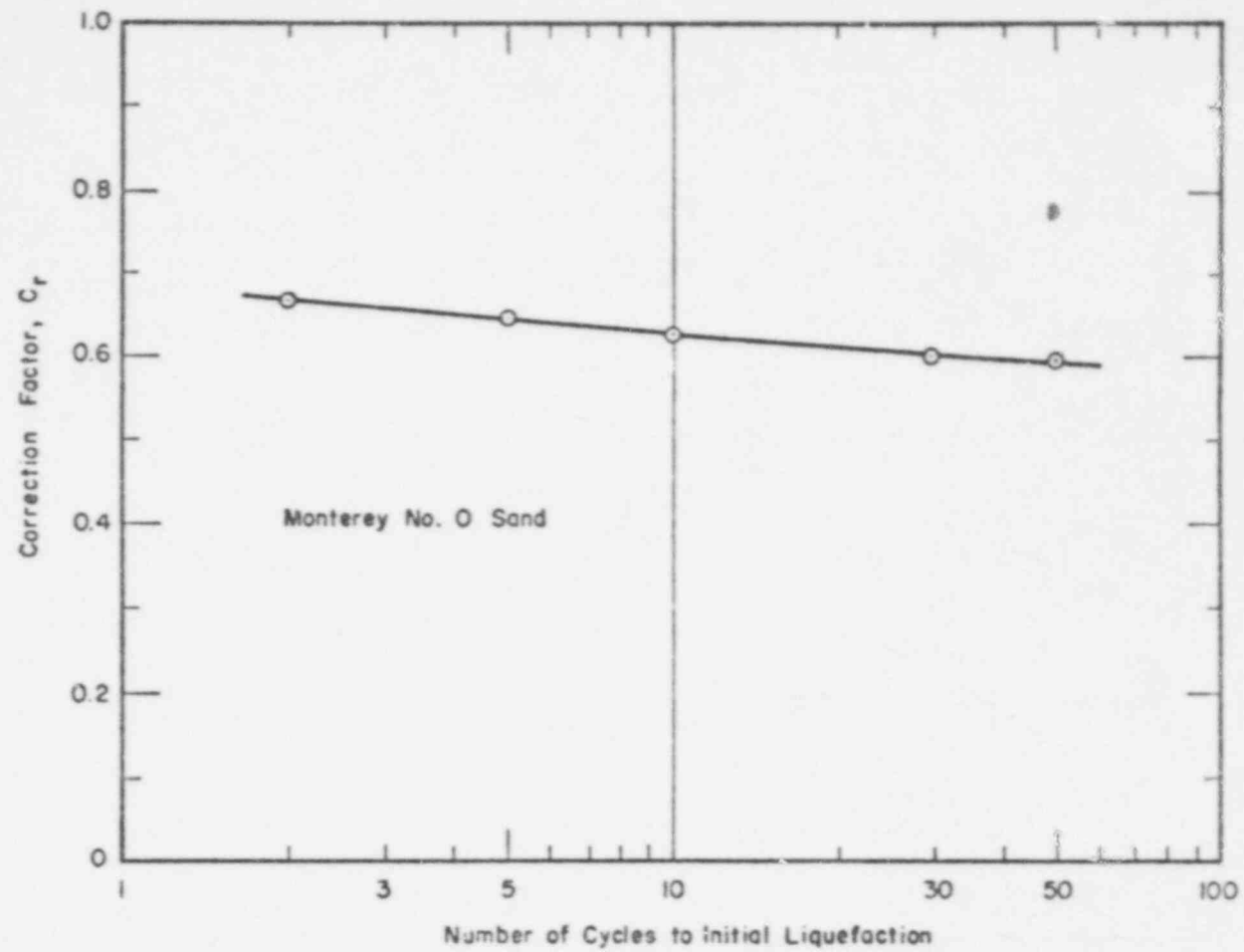
FIG. 3-7 CORRECTION FACTORS FOR TRIAXIAL TEST RESULTS
