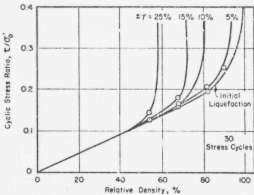
FIG. 4-2 LIMITING SHEAR STRAINS - 30 STRESS CYCLES
