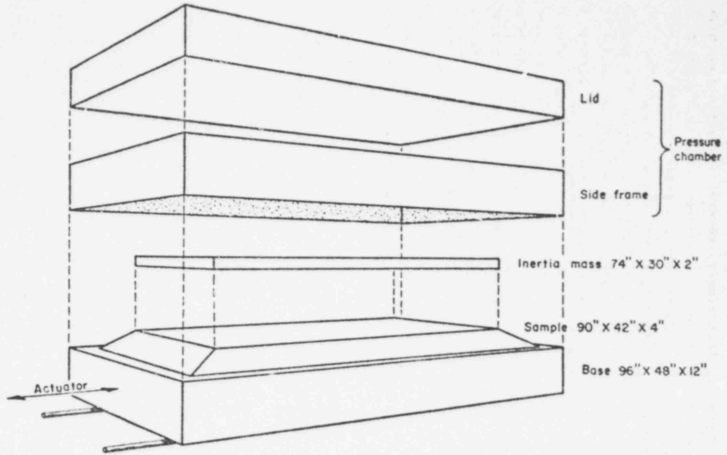
FIG. 2-1 SHAKING TABLE SYSTEM: SCHEMATIC VIEW
