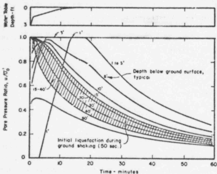
FIG. 1-3b COMPUTED VARIATION OF PORE WATER PRESSURE IN 60 MINUTE PERIOD FOLLOWING EARTHQUAKE FOR SOIL PROFILE
