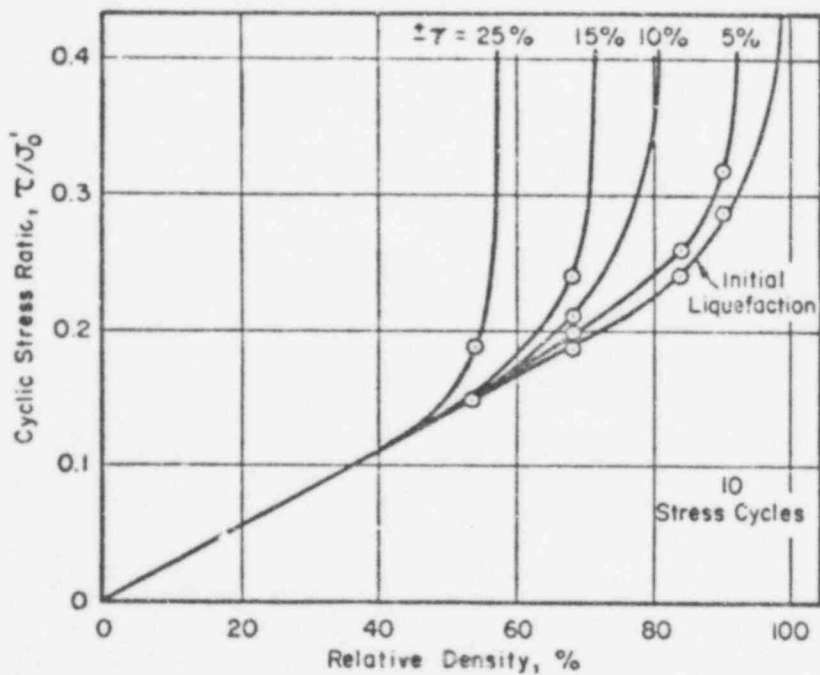
FIG. 4-1 LIMITING SHEAR STRAINS - 10 STRESS CYCLES
