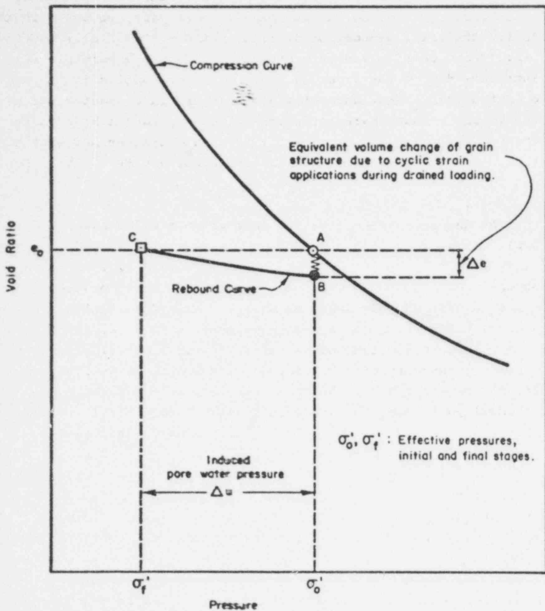
FIG. 1-2 SCHEMATIC ILLUSTRATION OF MECHANISM OF PORE PRESSURE GENERATION DURING CYCLIC LOADING
