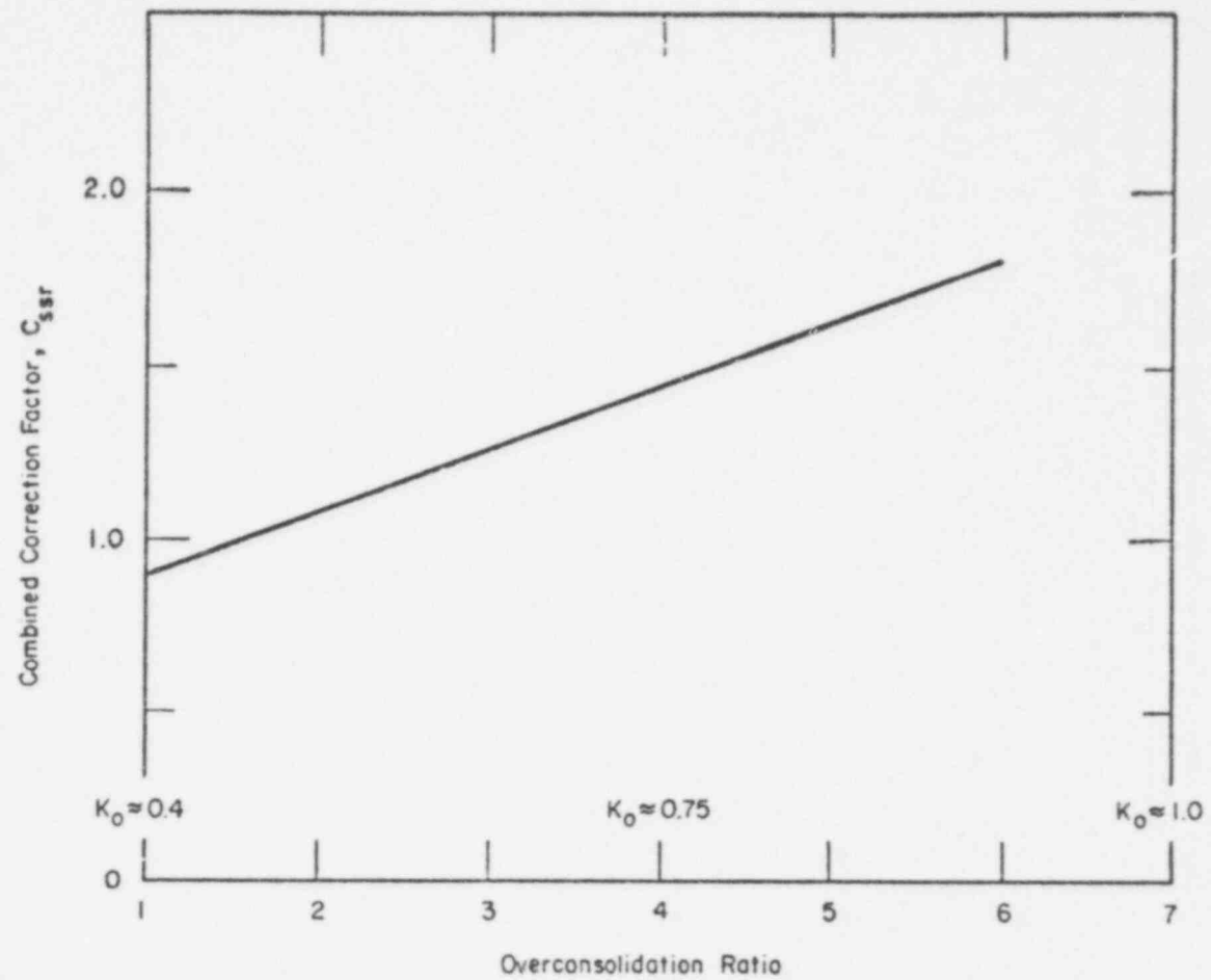
FIG. 3-15 COMBINED CORRECTION FACTOR FOR CYCLIC SIMPLE SHEAR TESTS ACCOUNTING FOR MULTIDIRECTIONAL SHAKING AND OVERCONSOLIDATION
