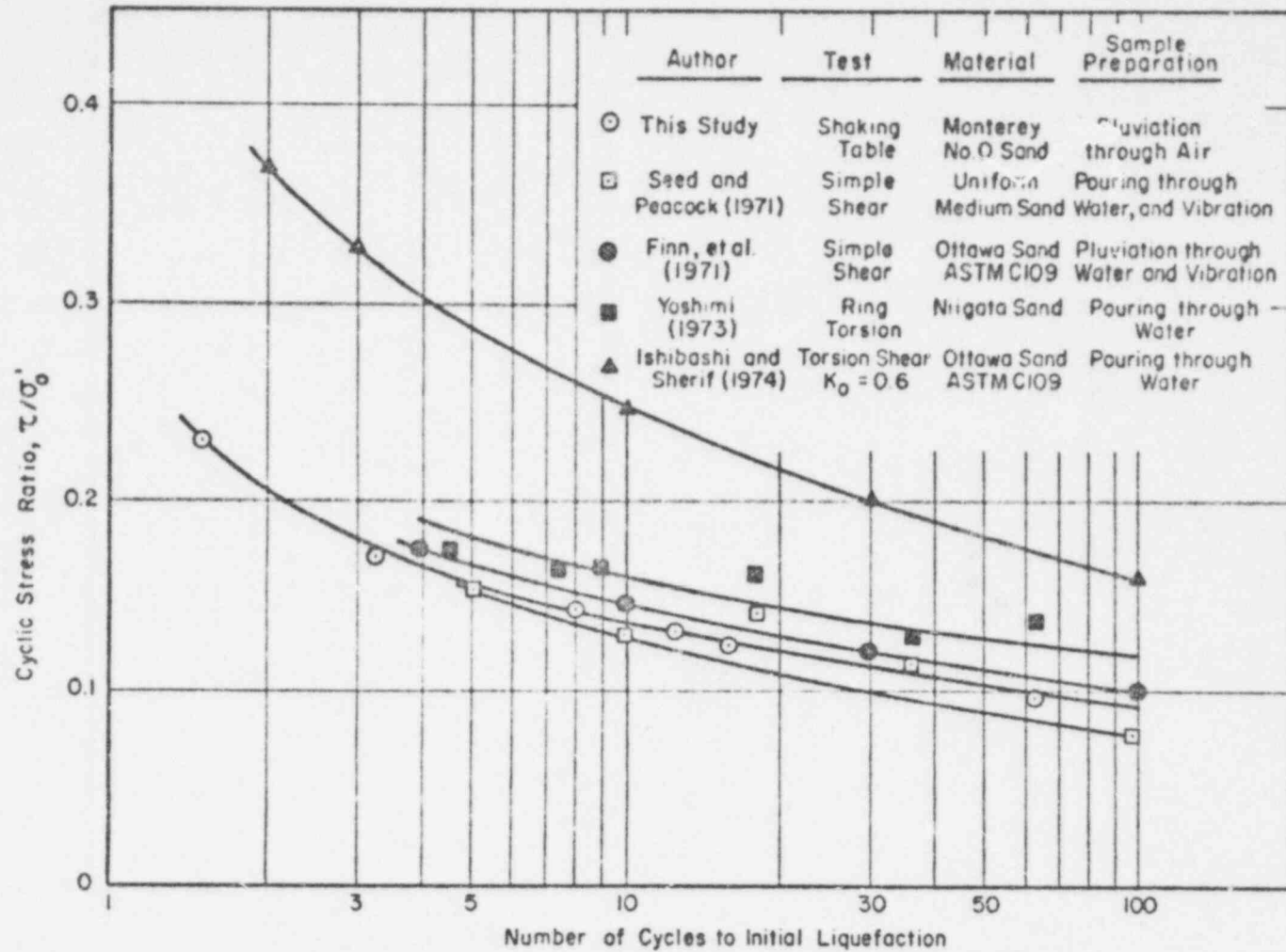
FIG. 3-4 COMPARISON OF SHAKING TABLE AND SIMPLE SHEAR LIQUEFACTION TEST RESULTS FOR D_r = 50\%
