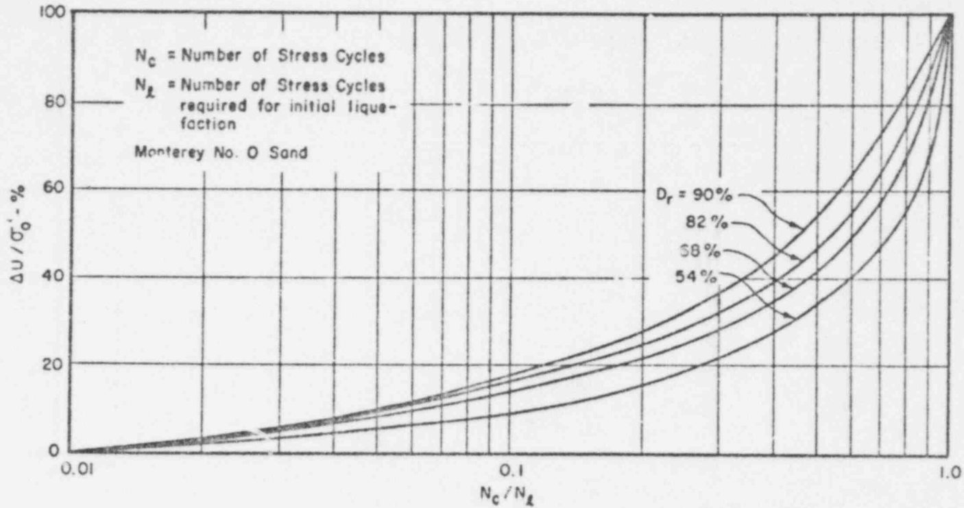
FIG. 3-2 NORMALIZED DYNAMIC PORE WATER PRESSURE CURVES
