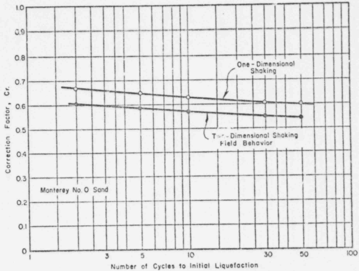
FIG. 3-12 CORRECTION FACTOR FOR CYCLIC TRIAXIAL TESTS ACCOUNTING FOR TWO-DIMENSIONAL SHAKING
