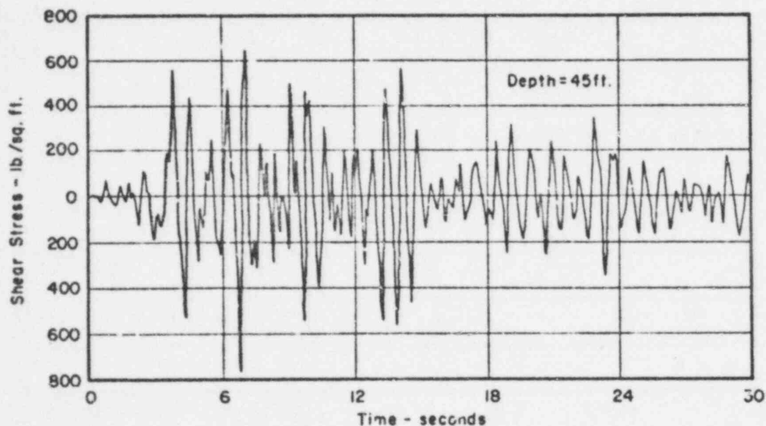
b) SHEAR STRESS VARIATION DETERMINED BY RESPONSE ANALYSIS
