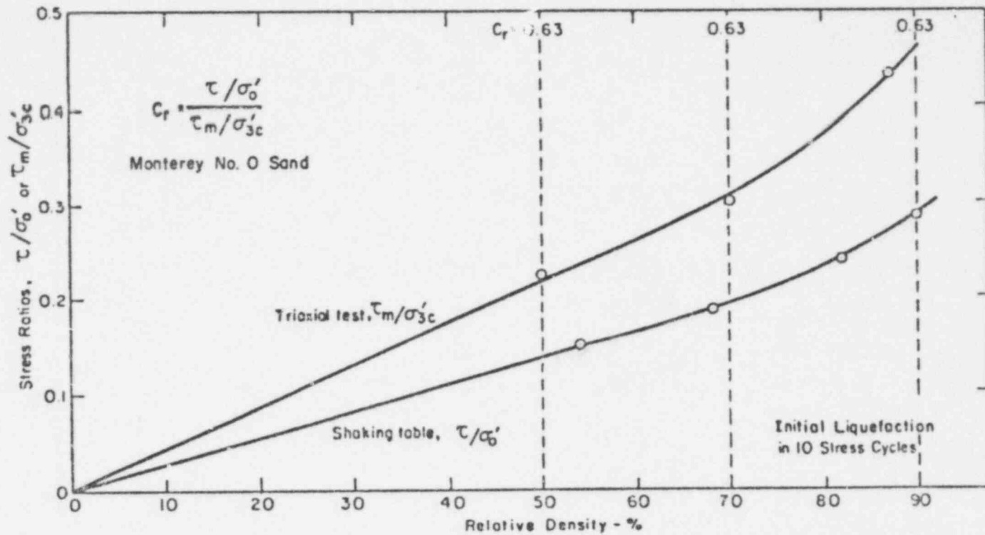
FIG. 3-6 COMPARISON OF SHAKING TABLE AND TRIAXIAL TEST RESULTS
