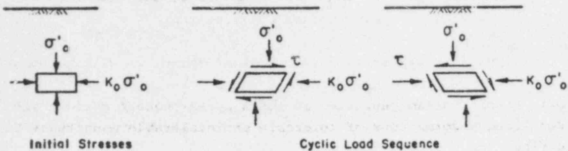
a) IDEALIZED FIELD LOADING CONDITIONS
