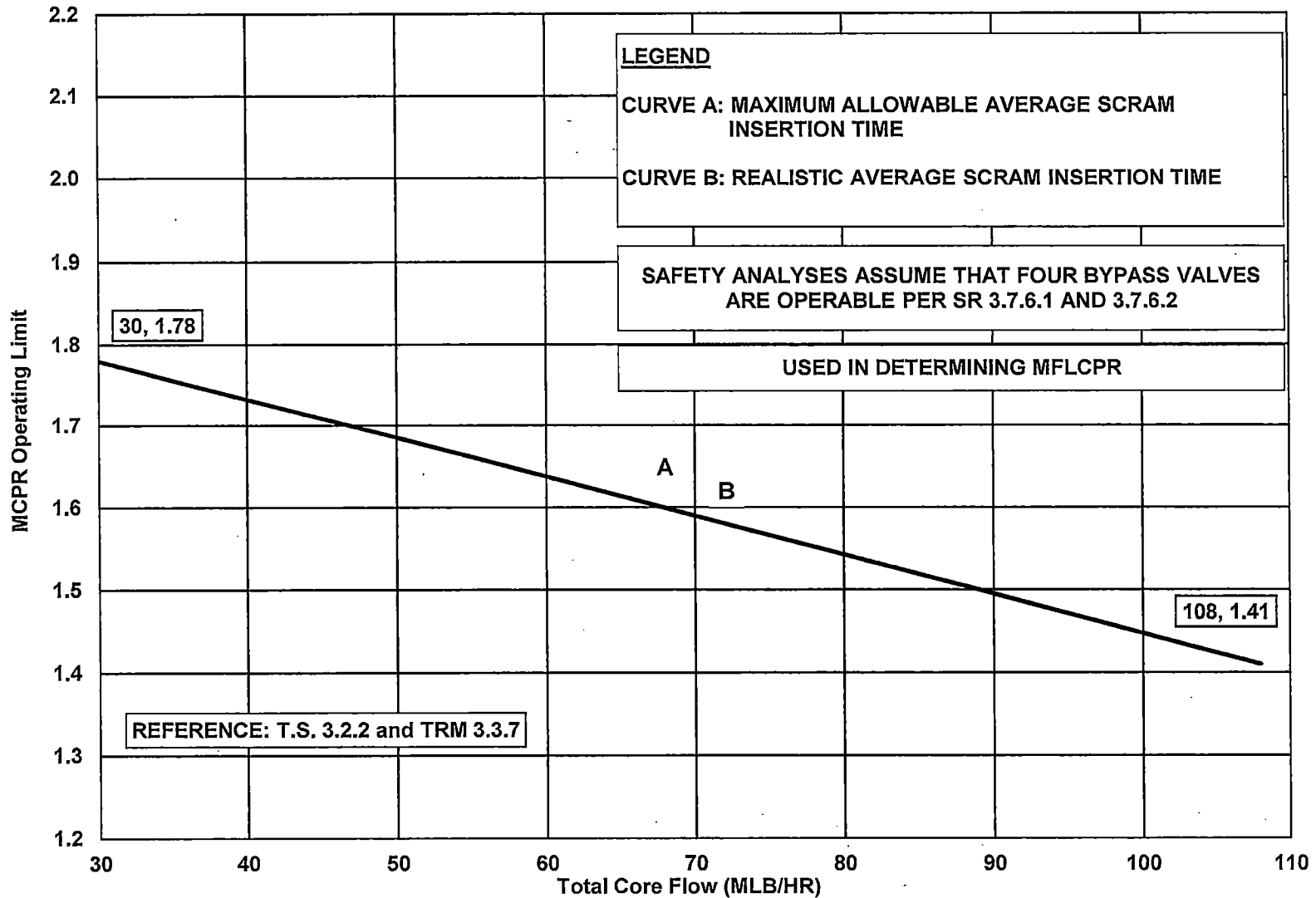
MCPR OPERATING LIMIT VERSUS TOTAL CORE FLOW ONE TSV OR TCV CLOSED* TWO LOOP OPERATION (BOC TO EOC) FIGURE 5.2-9
