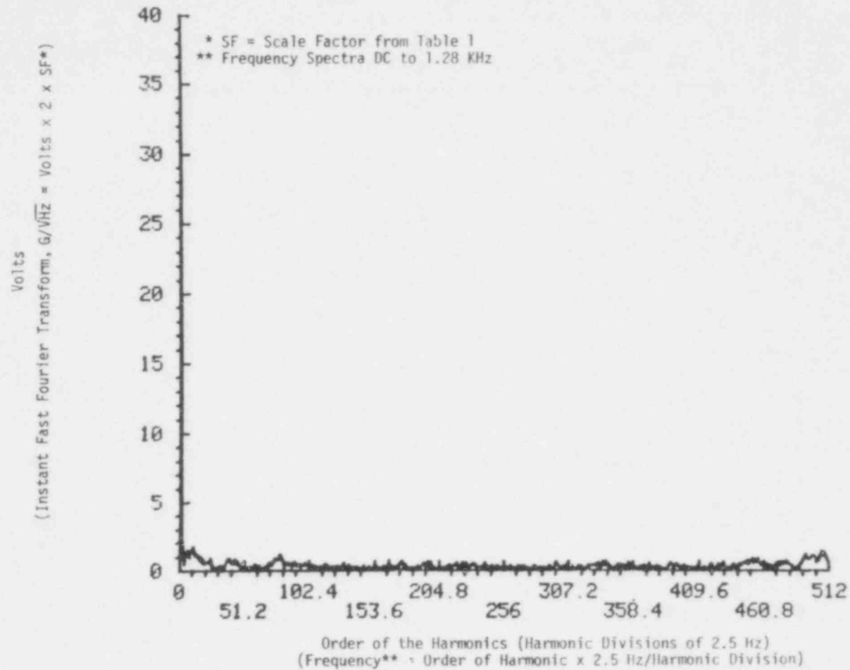
FIGURE 17. Horizontal Acceleration Response of Cask/Car Interface vs Frequency (Instrument No. 12 - Unfiltered).
