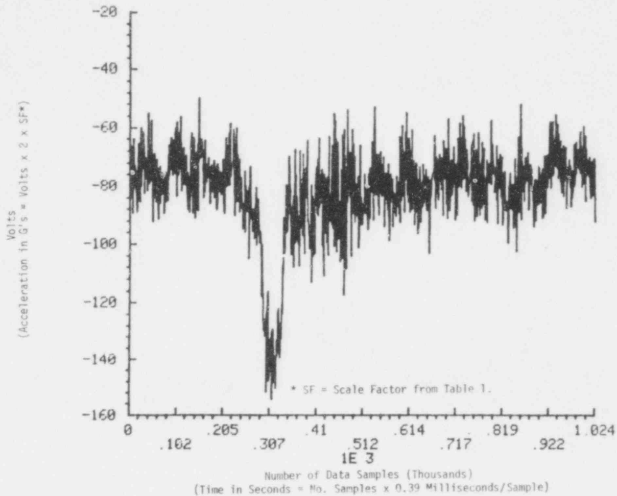
FIGURE 11. Horizontal or Longitudinal Acceleration of Cask at Far End vs Time (Instrument No. 10 - Unfiltered).
