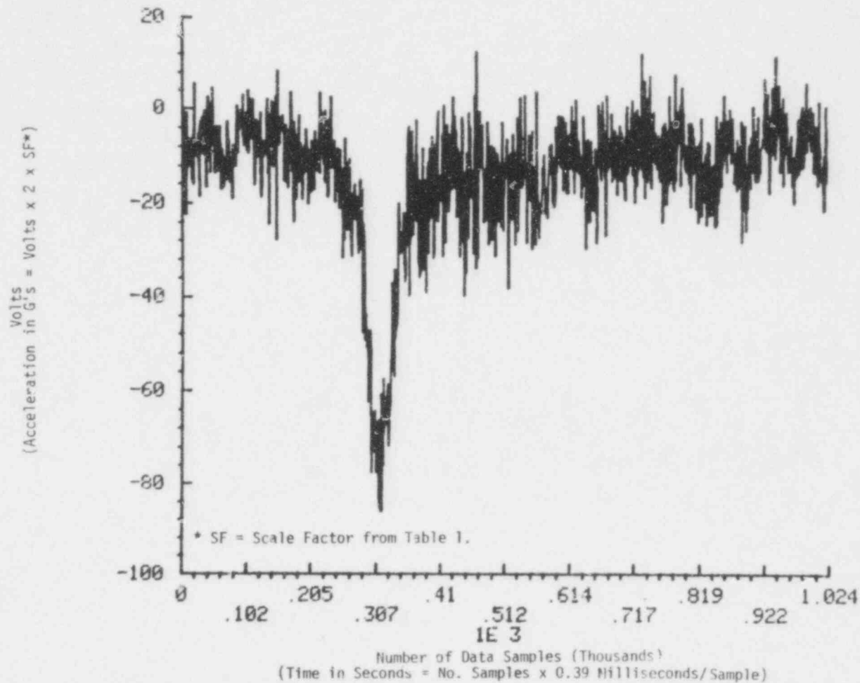
FIGURE 12. Horizontal or Longitudinal Acceleration of Cask at Struck End vs Time (Instrument No. 8 - Unfiltered).
