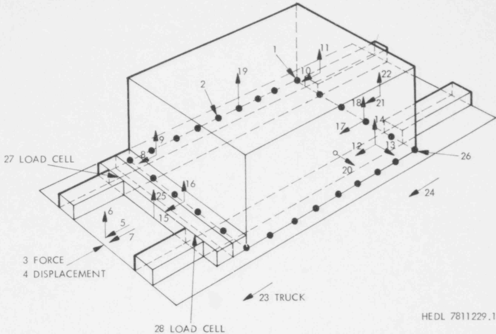
FIGURE 6. Tiedown Configuration and Instrument Location for Cask-Rail Car-Tiedown Tests (Tiedown Configuration "A"). Neg 7903318-1
