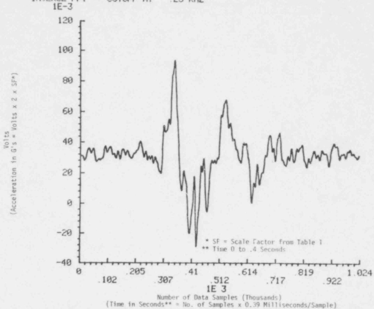
FIGURE 21. Vertical Acceleration of Cask at Far End vs Time (Instrument No. 11 - Filtered at 250 Hz).
