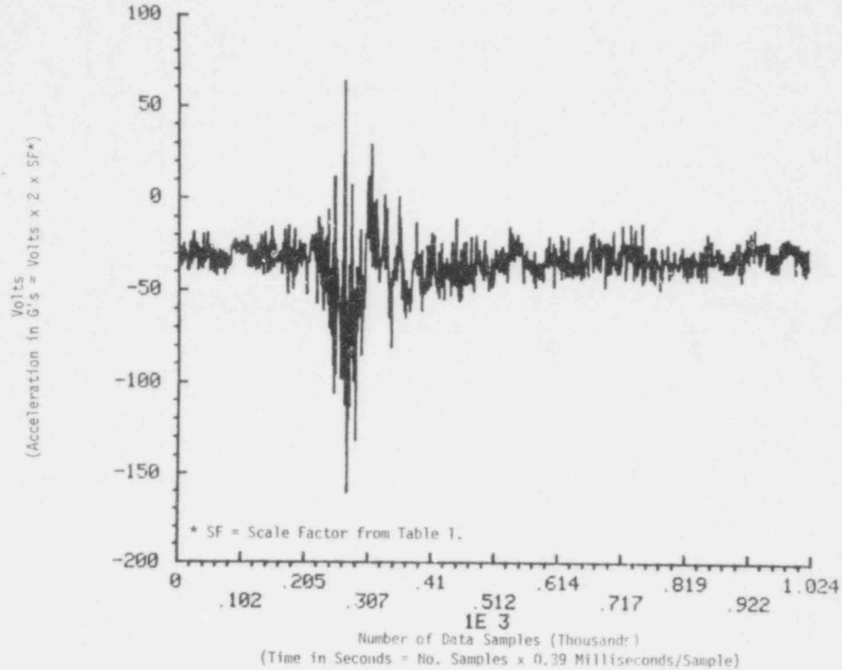
FIGURE 10. Horizontal or Longitudinal Acceleration of Car at Car/Cask Interface vs Time (Instrument No. 12 - Unfiltered).
