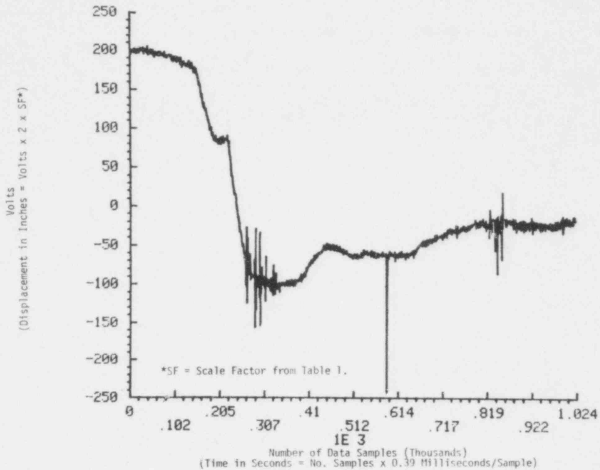
FIGURE 13. Horizontal Displacement of the Car at the Struck End vs Time (Instrument No. 4 - Unfiltered).
