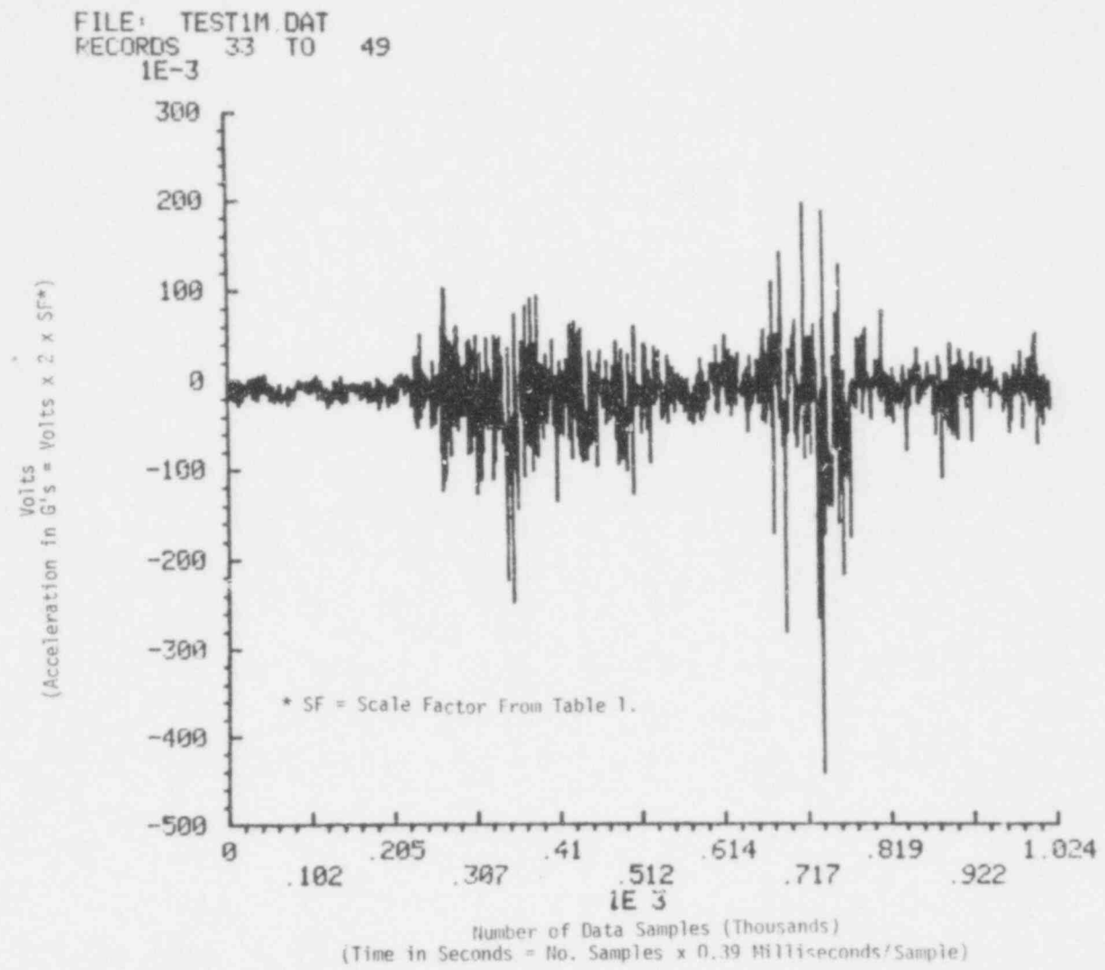
FIGURE 7. Vertical Acceleration of Car Structure at Far End vs Time (Instrument No. 22 - Unfiltered).
