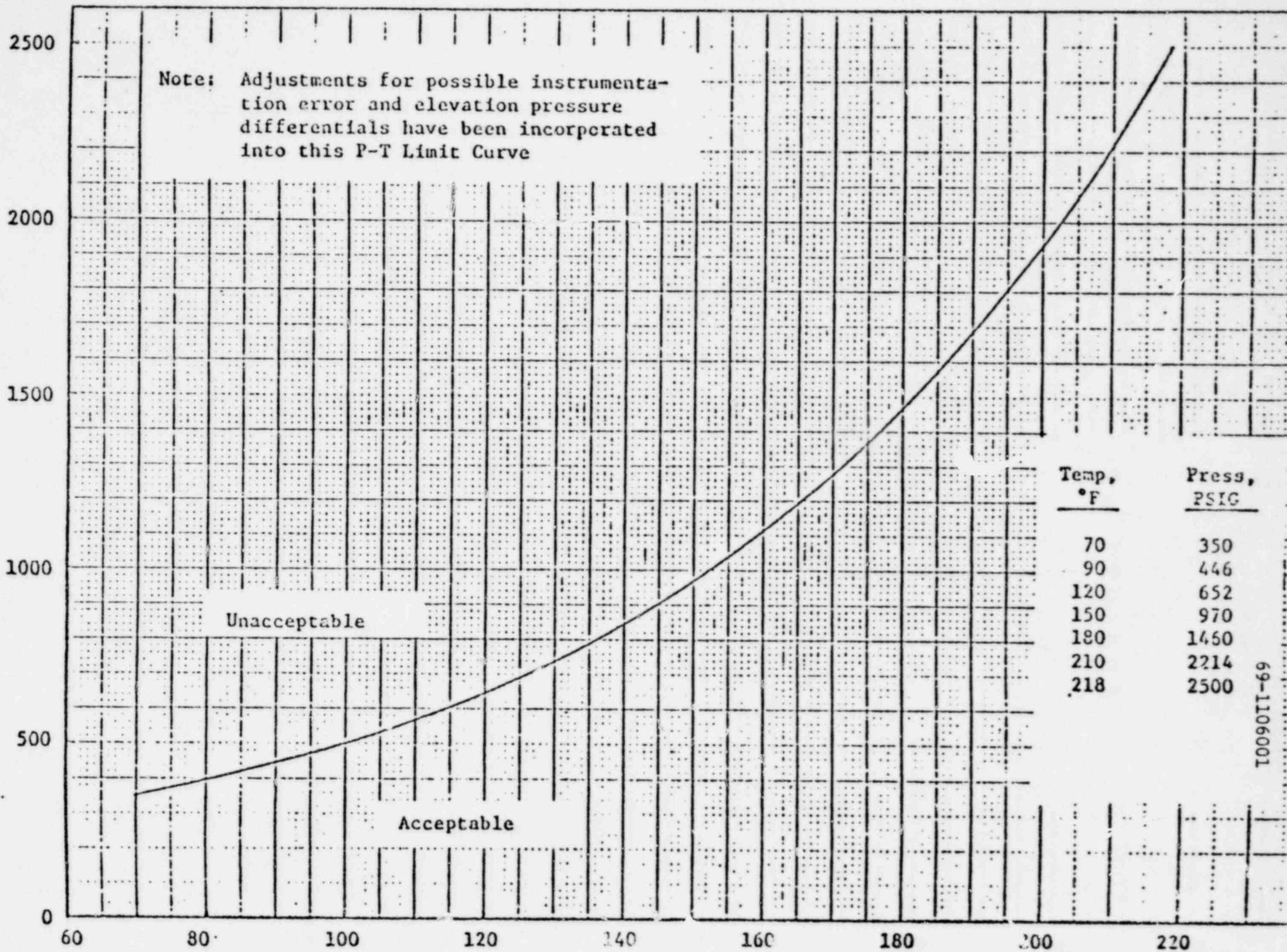
Figure 1 Pressure-Temperature Limit Curve to Preclude Reactor Vessel Brittle Fracture during RCS Depressurization Following Accident Conditions. Applicability: 2 EFPY of Operation beyond 6/79
