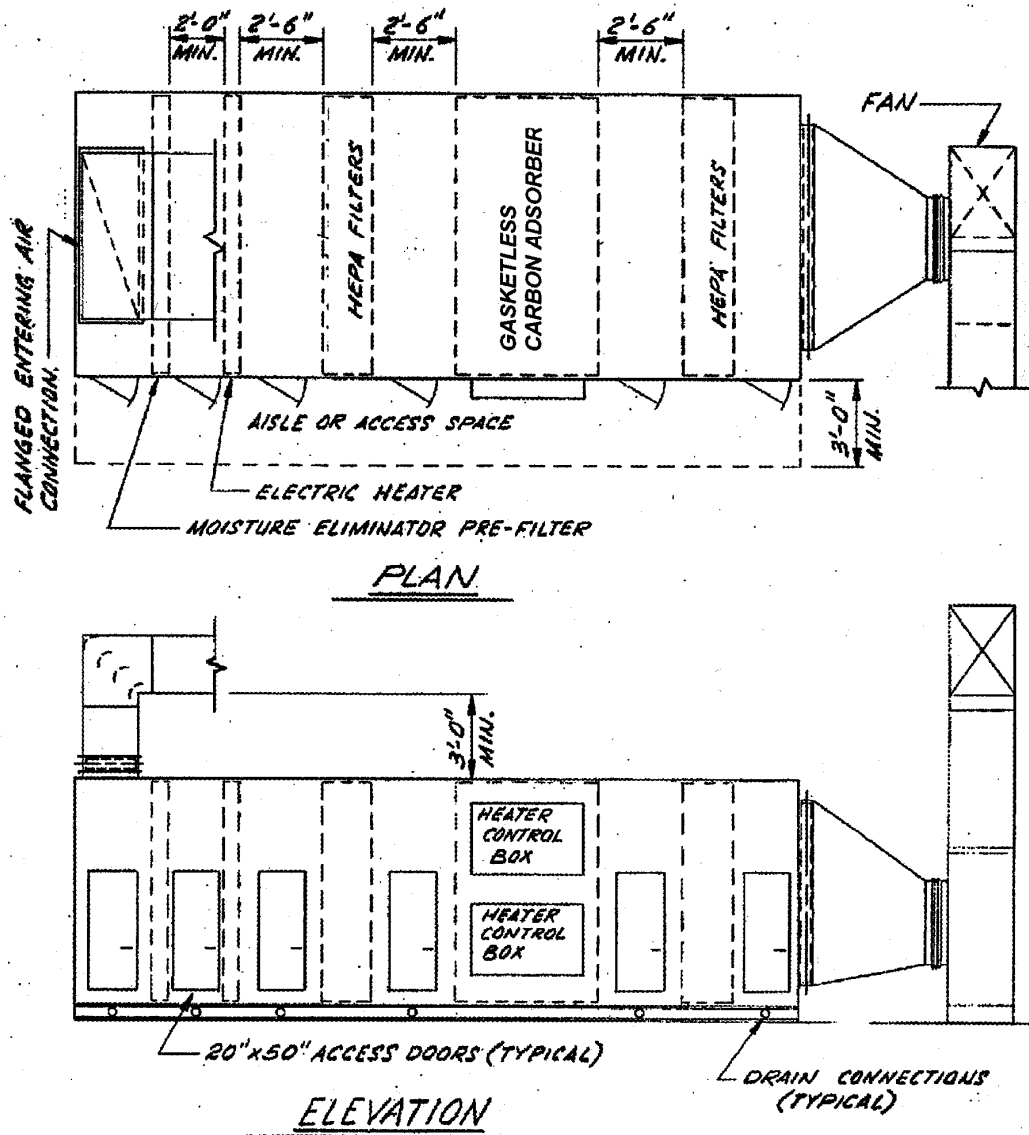
Figure 12-30. Typical Nuclear Safety Related Air Clean-Up System
