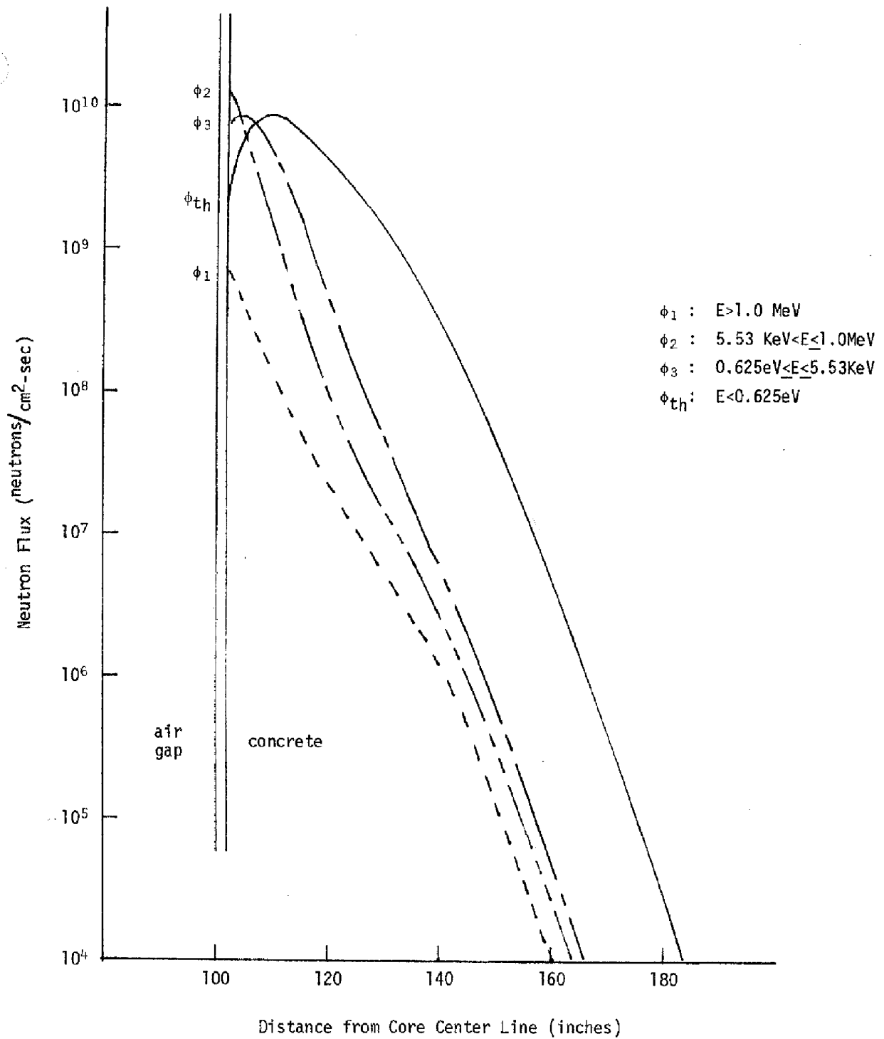
Figure 12-29. Primary Shield Neutron Flux Distribution
