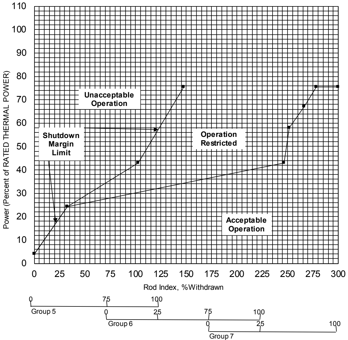
Figure 2c Regulating Group Position Operating Limits 0 to 300 ±10 EFPD, Three RC Pumps Davis-Besse 1, Cycle 21
