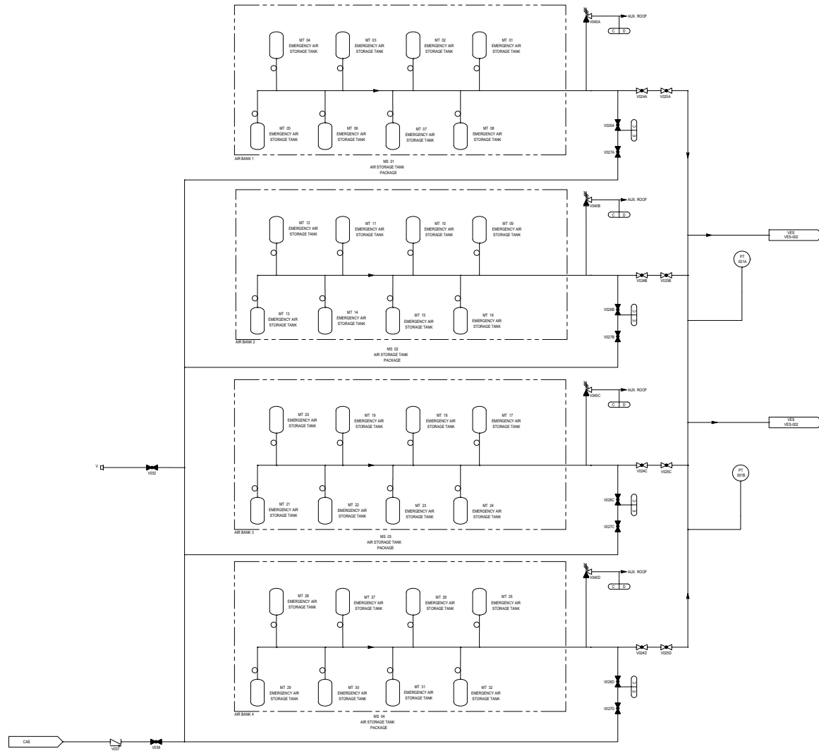
Figure 6.4-2 (Sheet 1 of 2) Simplified Main Control Room Habitability System Piping and Instrumentation Diagram (REF) VES 001
