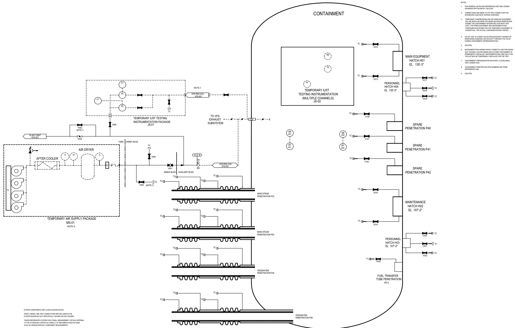
Figure 6.2.5-1 Simplified Containment Leak Rate Test System Piping and Instrumentation Diagram (REF) VUS 001
