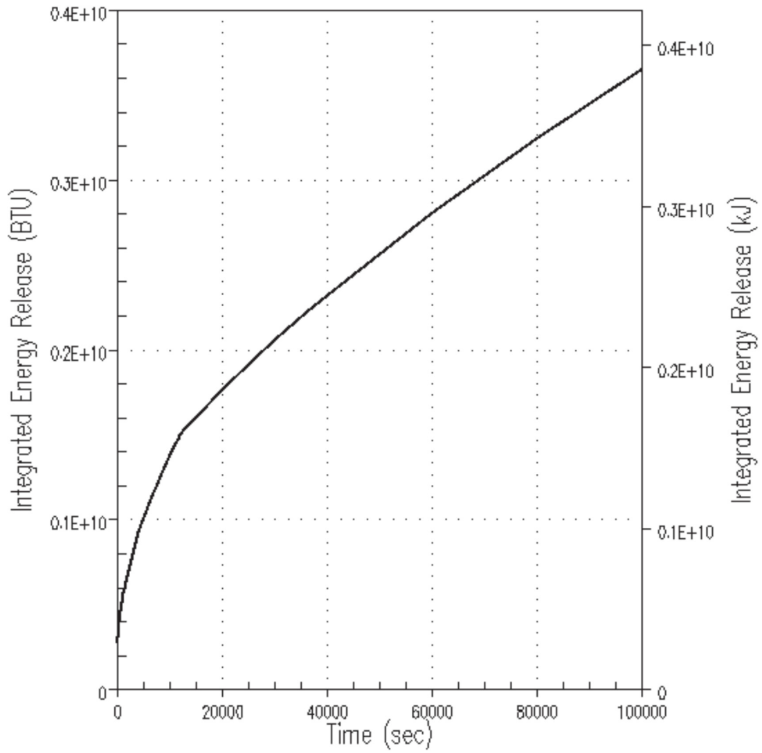
Figure 6.2.1.3-2 AP1000 DECLG LOCA Integrated Energy Released
