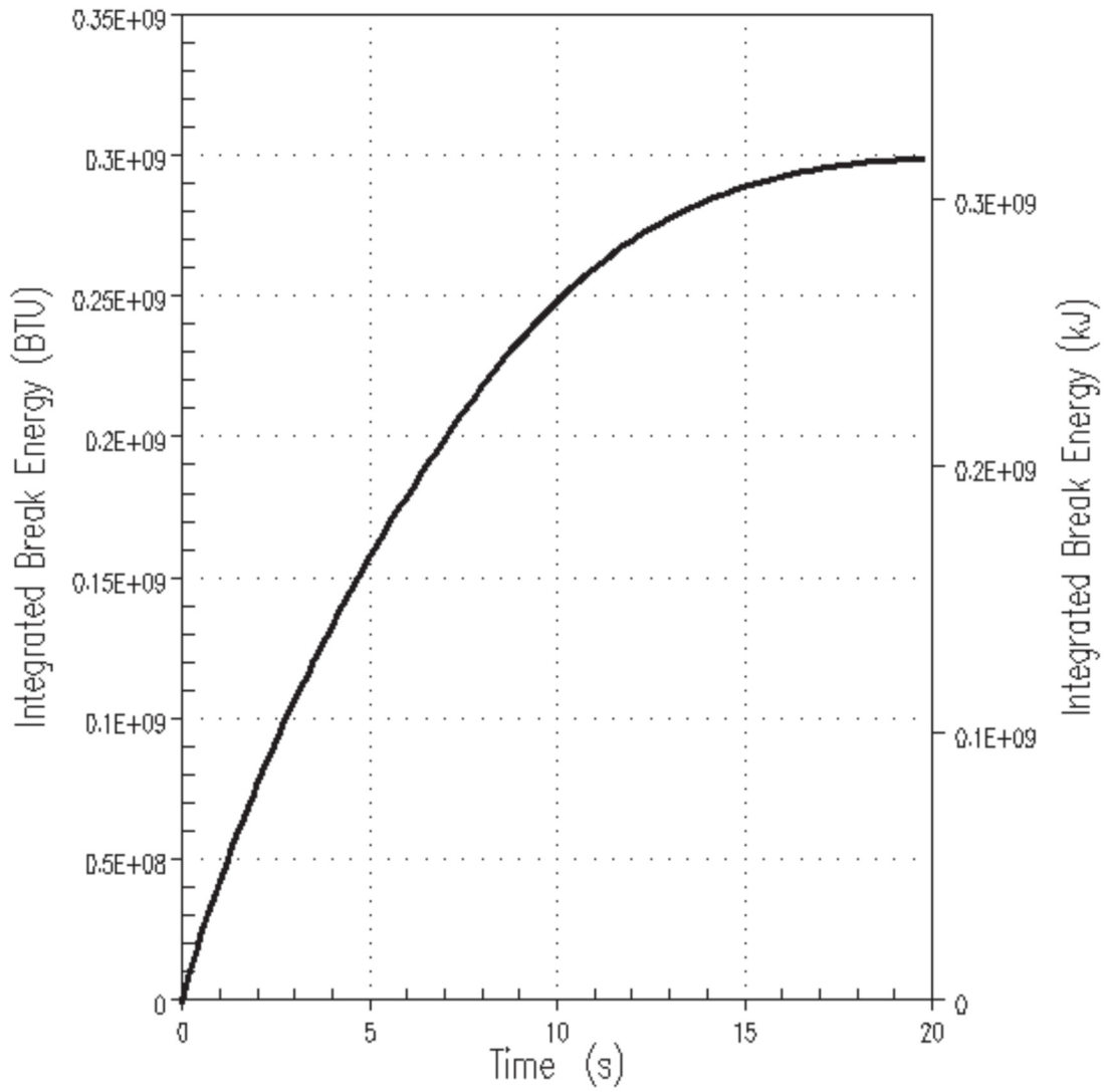
Figure 6.2.1.3-4 AP1000 DEHLG LOCA Integrated Energy Released
