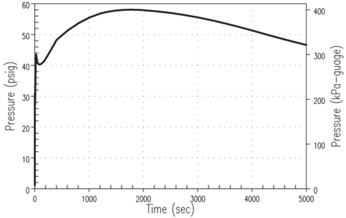
Figure 6.2.1.1-5 AP1000 Containment Pressure Response for DECLG LOCA – 5000 sec
