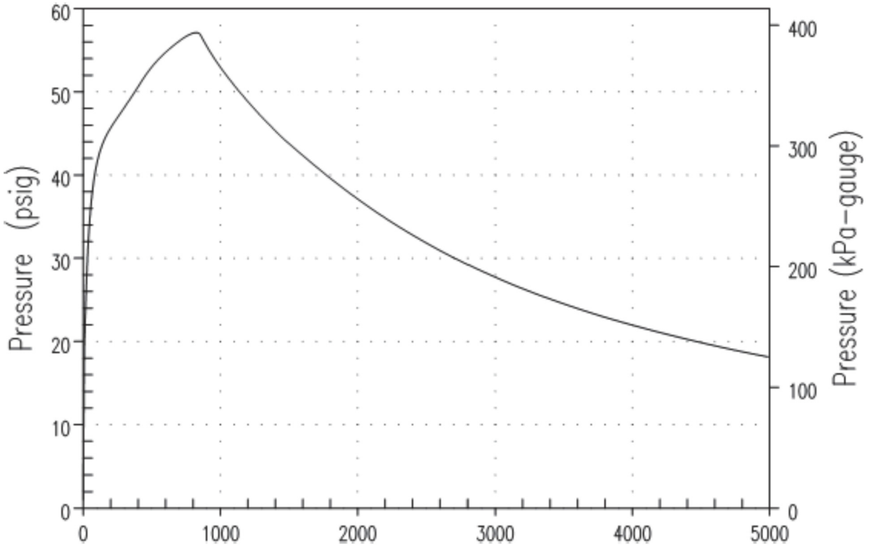
Figure 6.2.1.1-1 AP1000 Containment Pressure Response for Full DER MSLB – 30% Power
