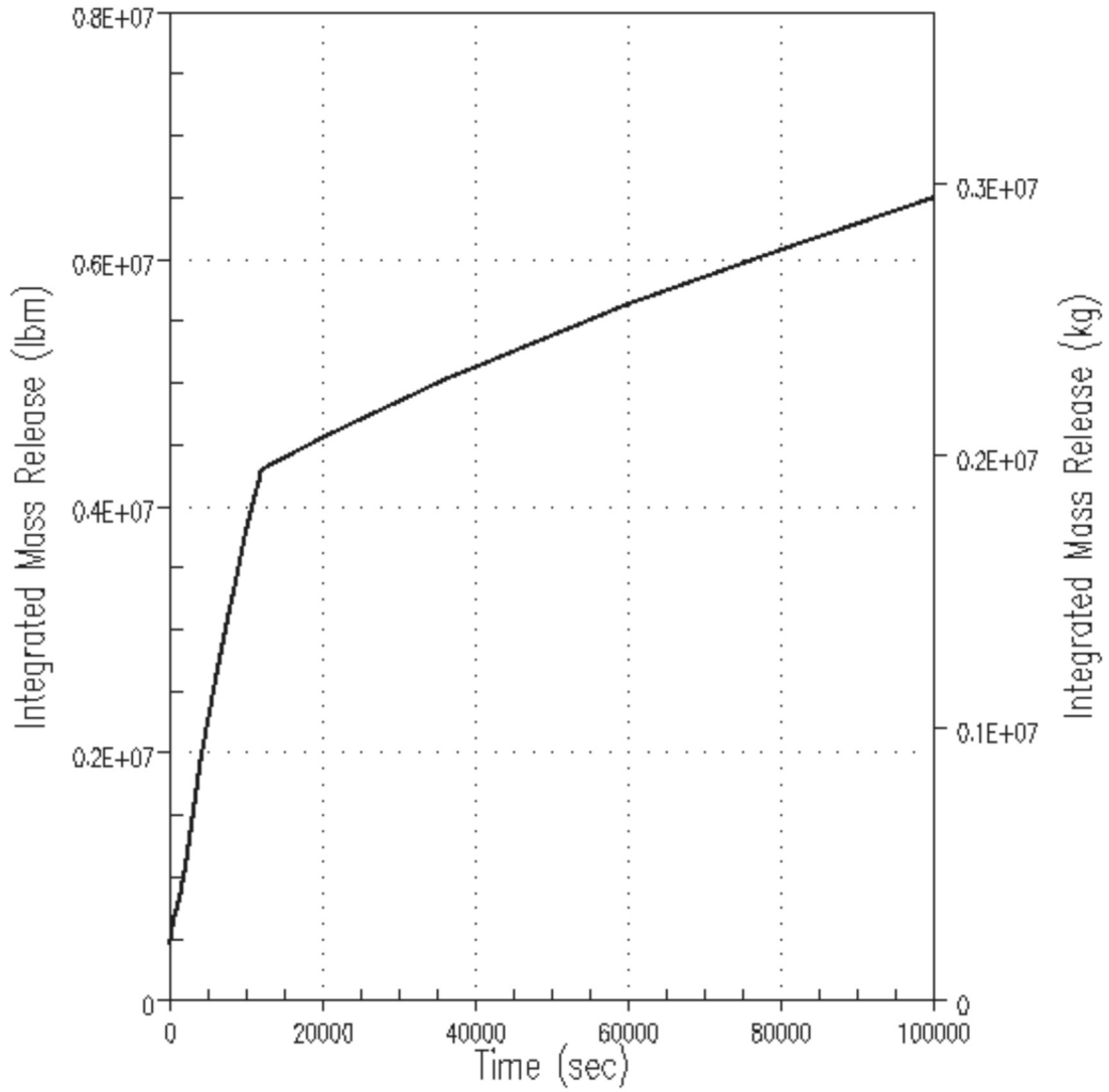
Figure 6.2.1.3-1 AP1000 DECLG Integrated Break Flow
