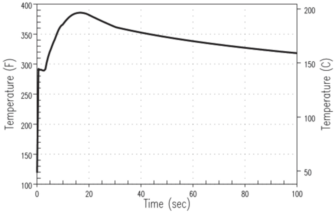
Figure 6.2.1.1-10 AP1000 Containment Temperature Response for DEHLG LOCA
