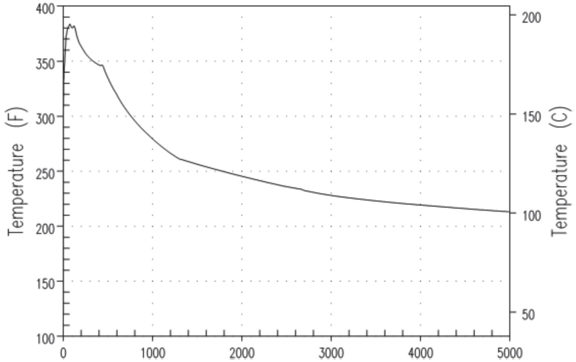
Figure 6.2.1.1-2 AP1000 Containment Temperature Response for Full DER MSLB – 101% Power
