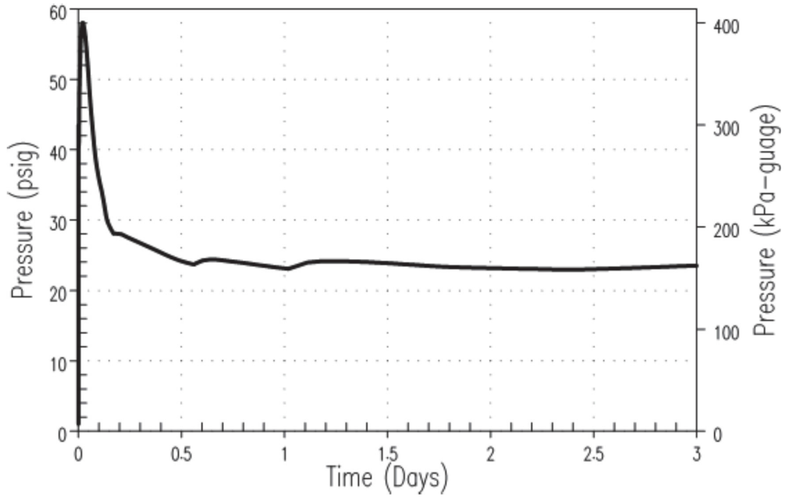
Figure 6.2.1.1-7 AP1000 Containment Pressure Response for DECLG LOCA – 3 Days
