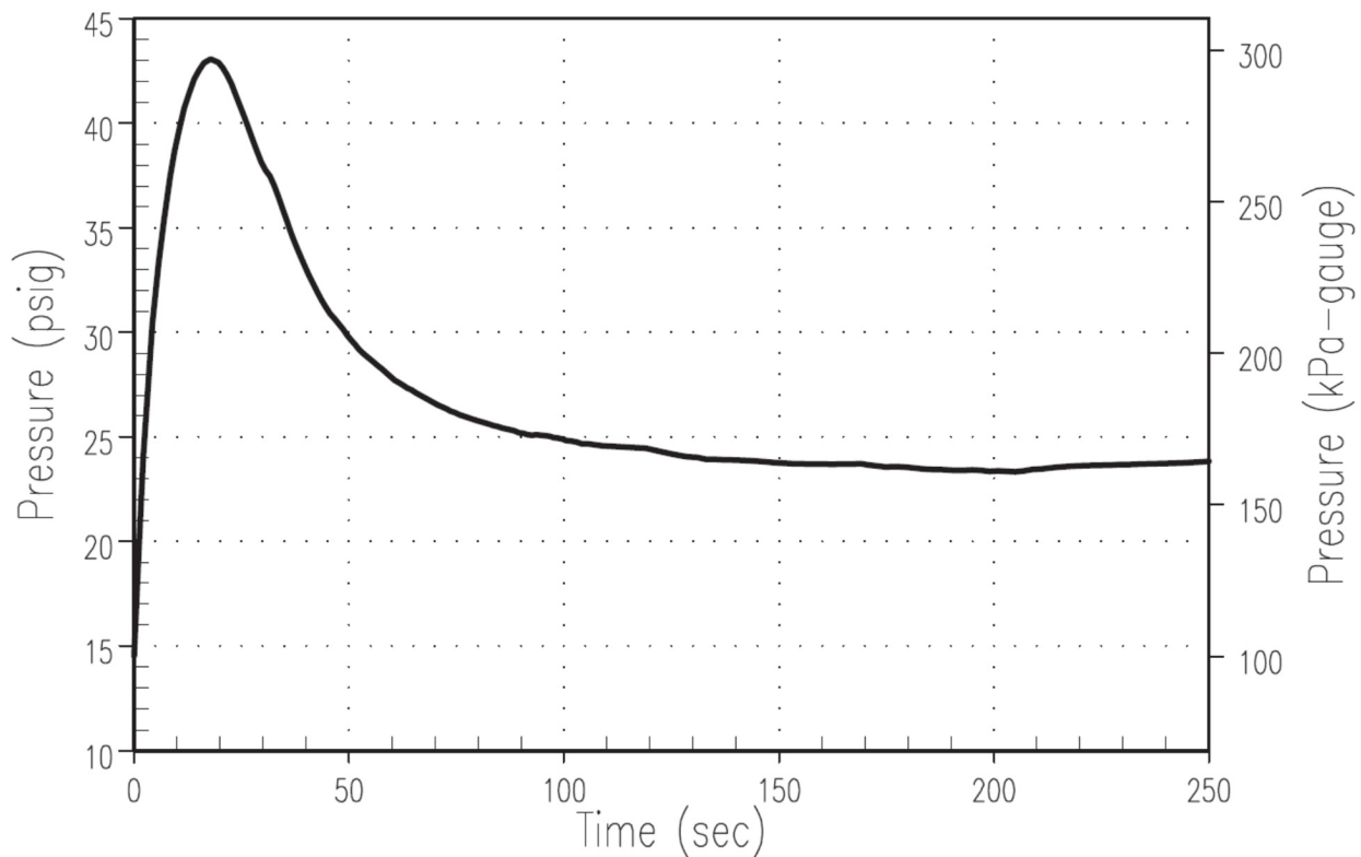
Figure 6.2.1.5-1 AP1000 Minimum Containment Pressure for DECLG LOCA
