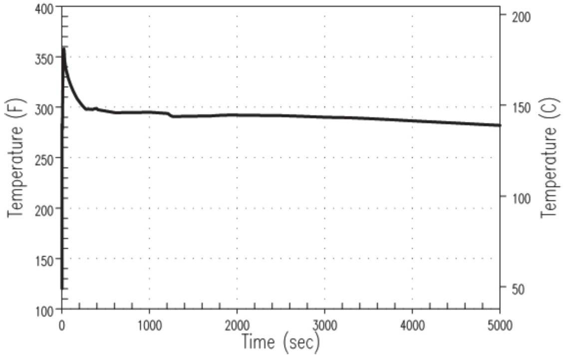
Figure 6.2.1.1-6 AP1000 Containment Temperature Response to DECLG LOCA – 5000 sec
