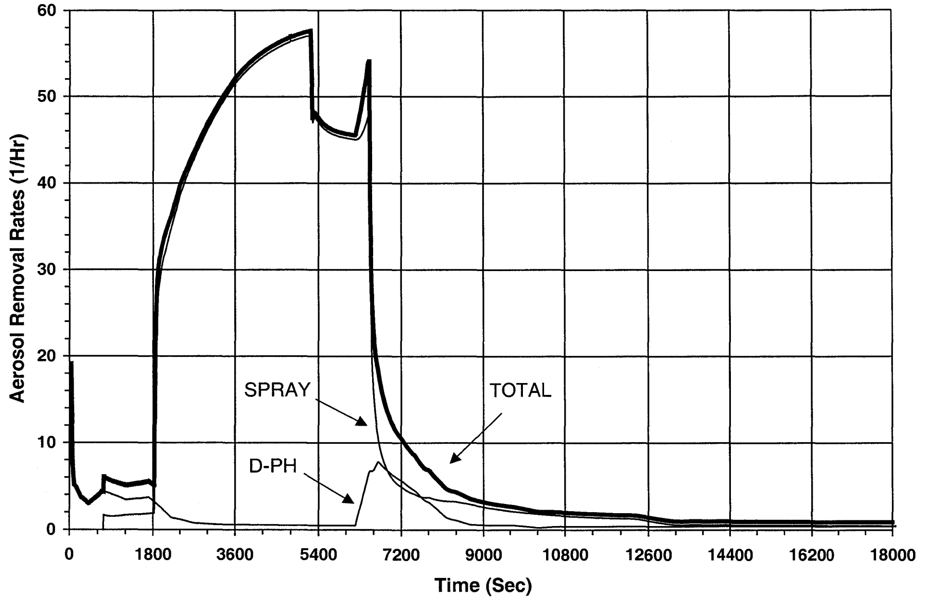
FIGURE 6.5-3 Aerosol Removal Rates Within Sprayed Region (NUREG 1465 HLDER Min. Case) BEAVER VALLEY POWER STATION-UNIT 2 UPDATED FINAL SAFETY ANALYSIS REPORT
