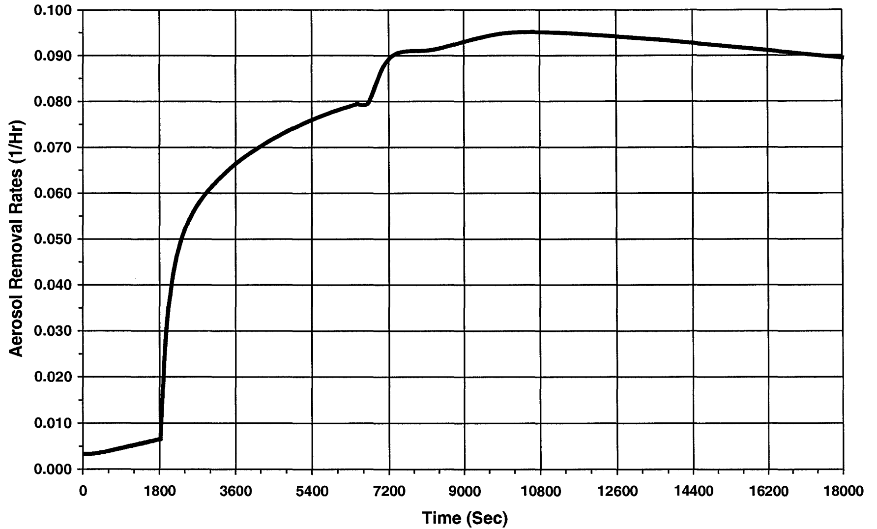
FIGURE 6.5-4 Aerosol Removal Rates Within Unsprayed Region (NUREG 1465 HLLER Min. Case) BEAVER VALLEY POWER STATION-UNIT 2 UPDATED FINAL SAFETY ANALYSIS REPORT
