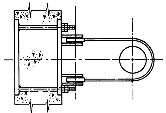
VIEW 2-2
