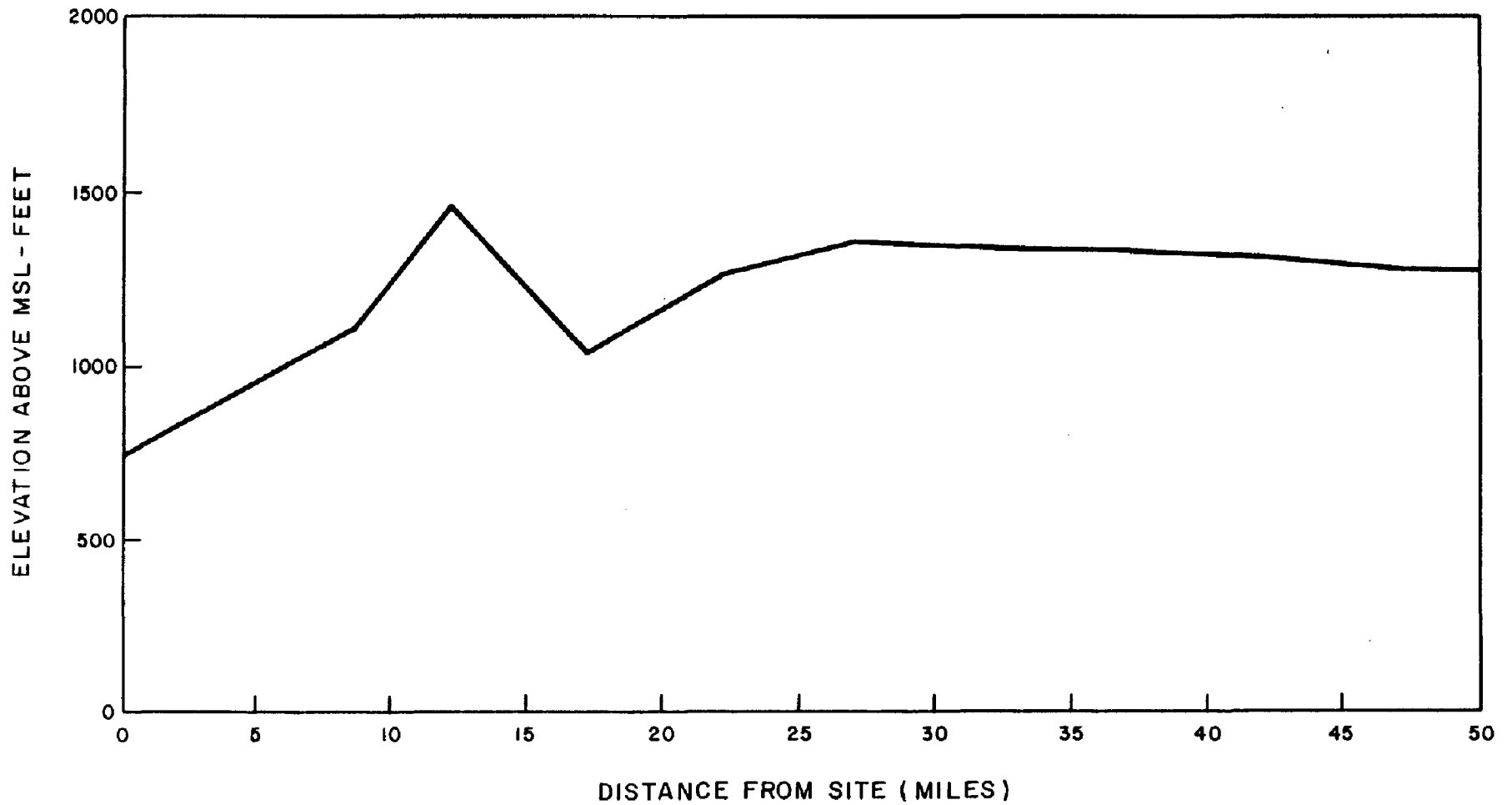
FIGURE 2.3 - 26 TOPOGRAPHIC CROSS SECTIONS TO 50 MILES FOR THE WEST NORTHWEST SECTOR BEAVER VALLEY POWER STATION - UNIT 2 FINAL SAFETY ANALYSIS REPORT
