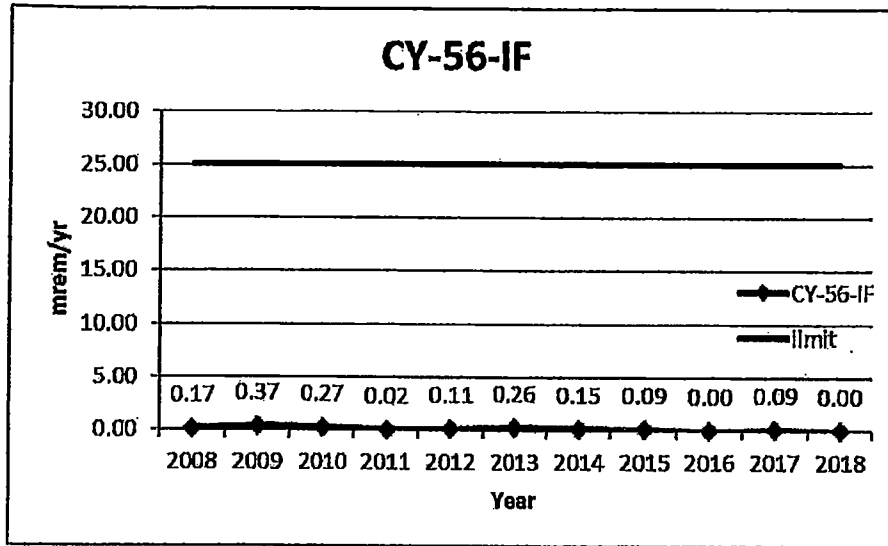
Figure 4.7 Annual Dose Trend at CY-56-IF
