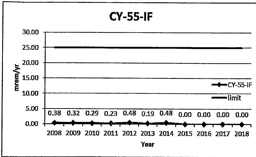
Figure 4.6 Annual Dose Trend at CY-55-IF
