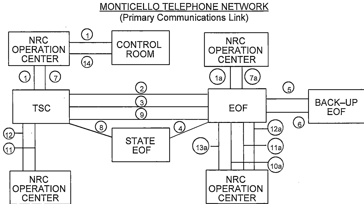
Figure 13.6 DIRECT DEDICATED TELEPHONES (HOT LINES)
