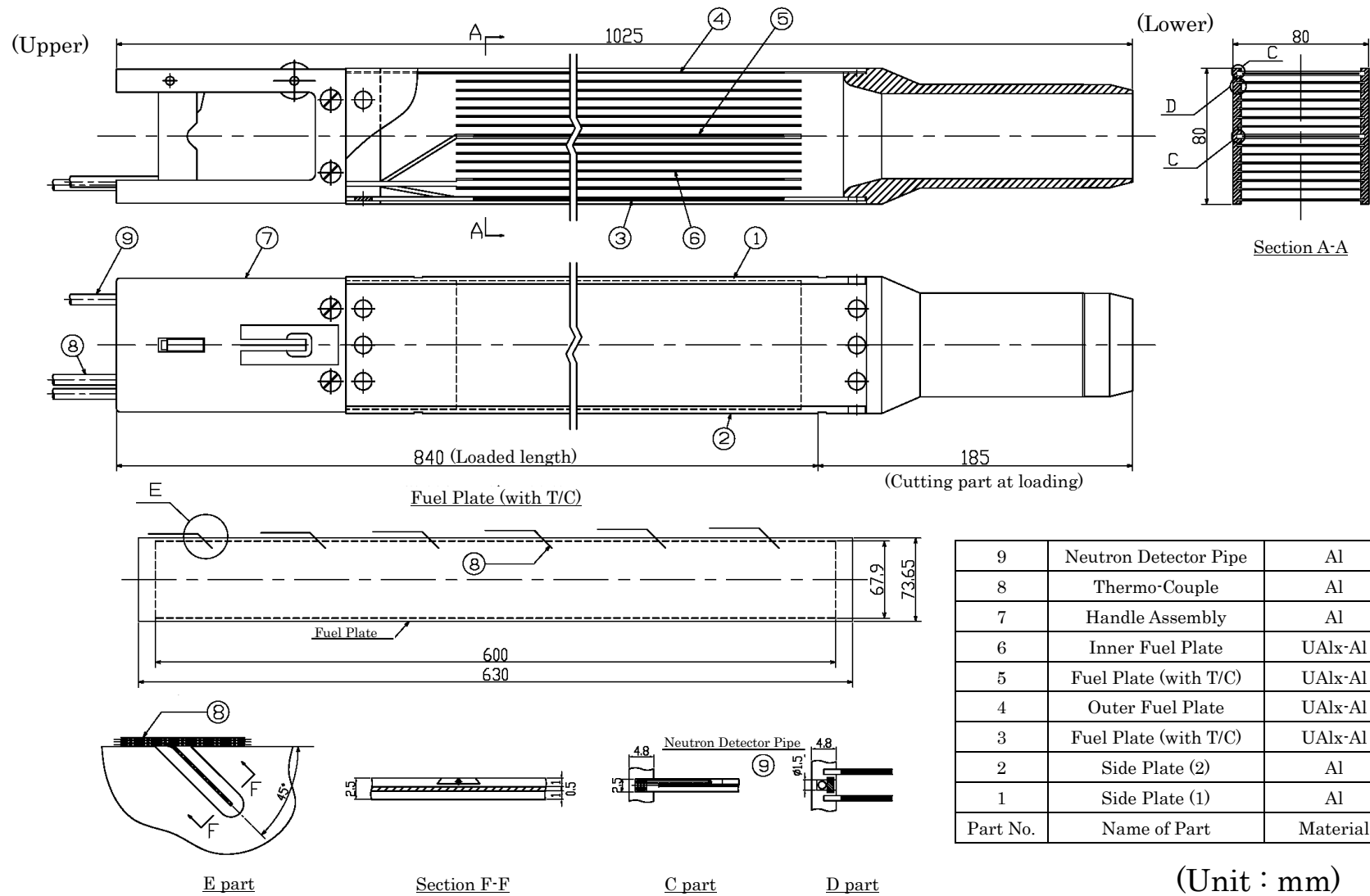
(I)-Fig.D.4 JRR-4 High Enrichment Instrumented Fuel (HEU)
