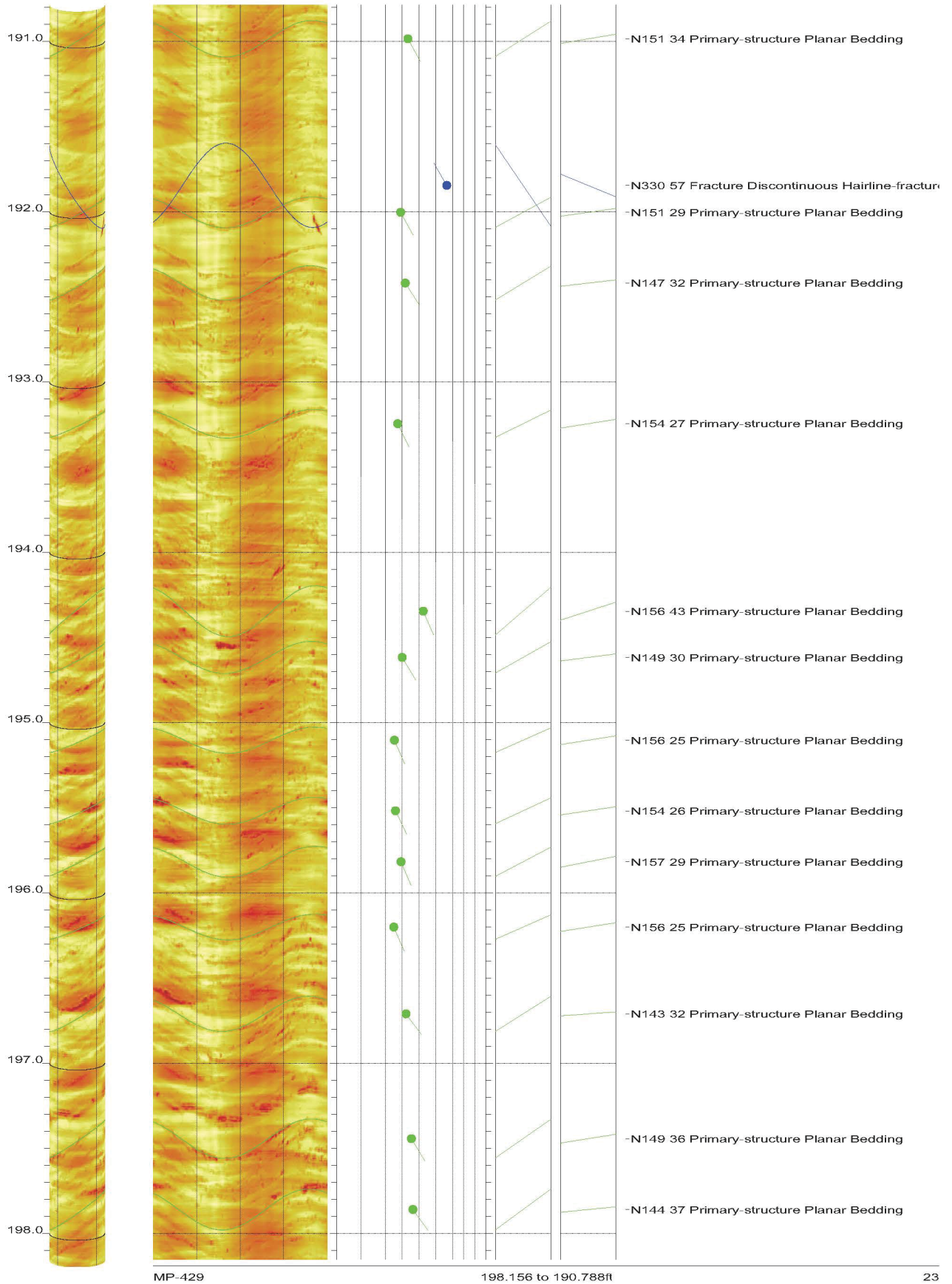
AMEC Clinch River SMR Project Borehole MP-429 Acoustic Televiewer Features rev 2 Sheet 23 of 24
