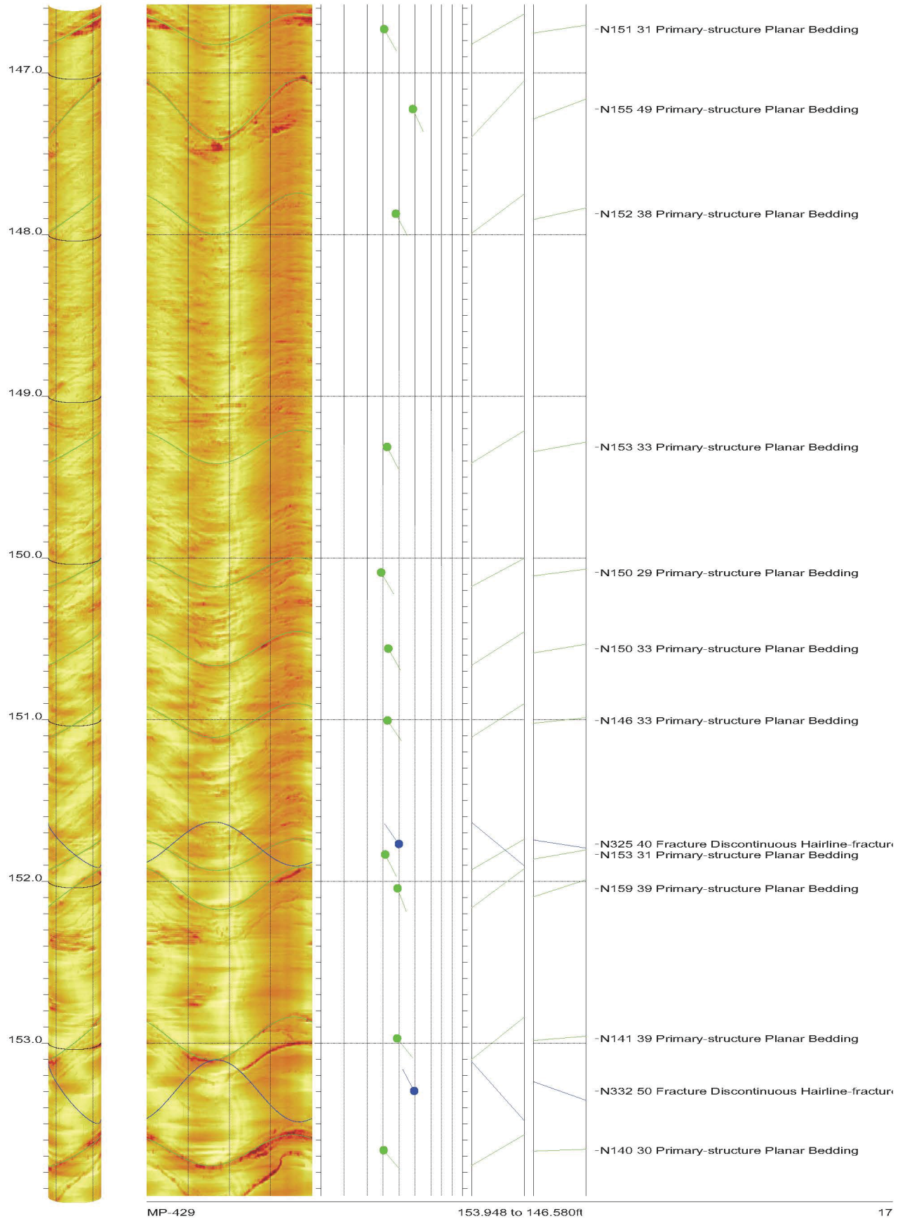
AMEC Clinch River SMR Project Borehole MP-429 Acoustic Televiewer Features rev 2 Sheet 17 of 24
