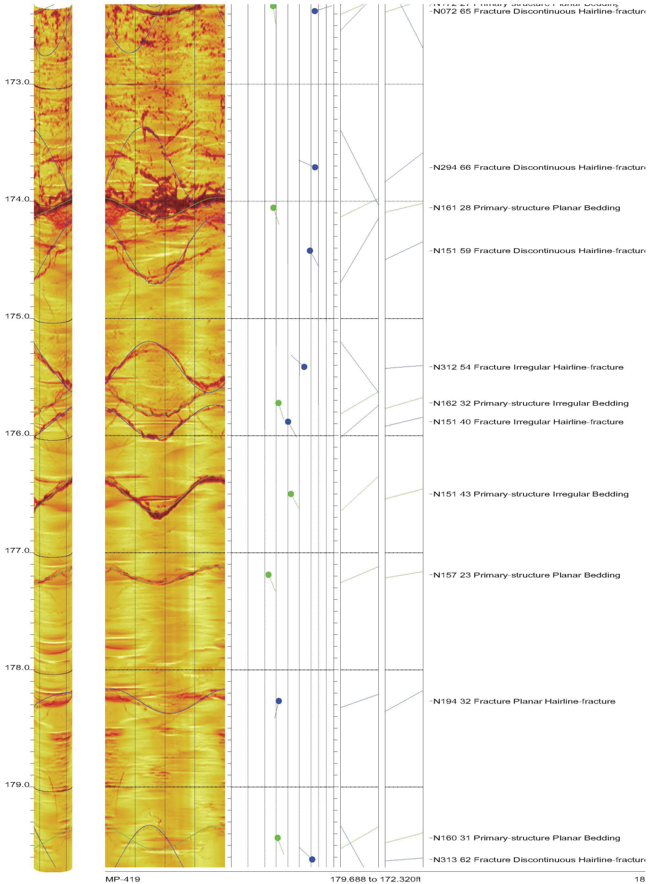
AMEC Clinch River SMR Project Borehole MP-419 Acoustic Televiewer Features rev 2 Sheet 18 of 37
