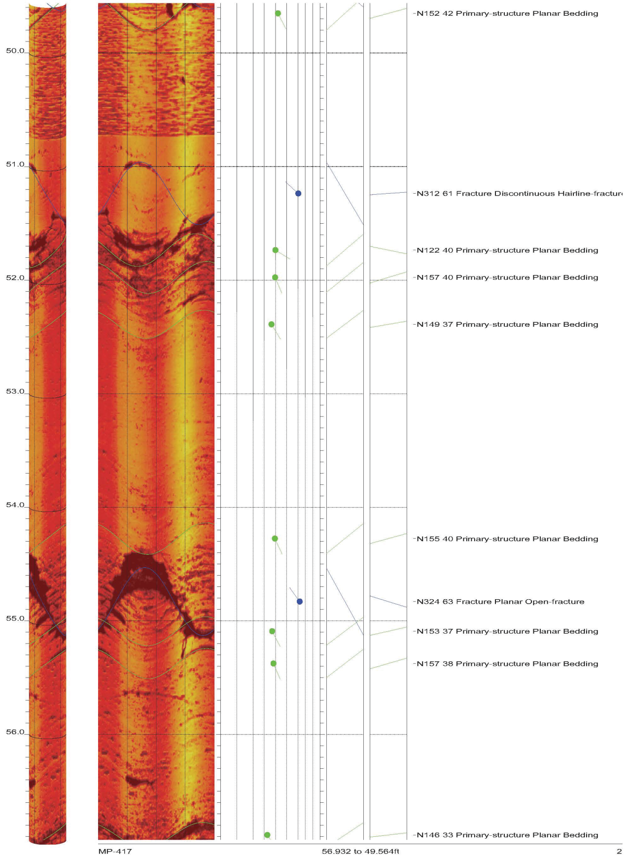
AMEC Clinch River SMR Project Borehole MP-417 Acoustic Televiewer Features rev 2 Sheet 2 of 38
