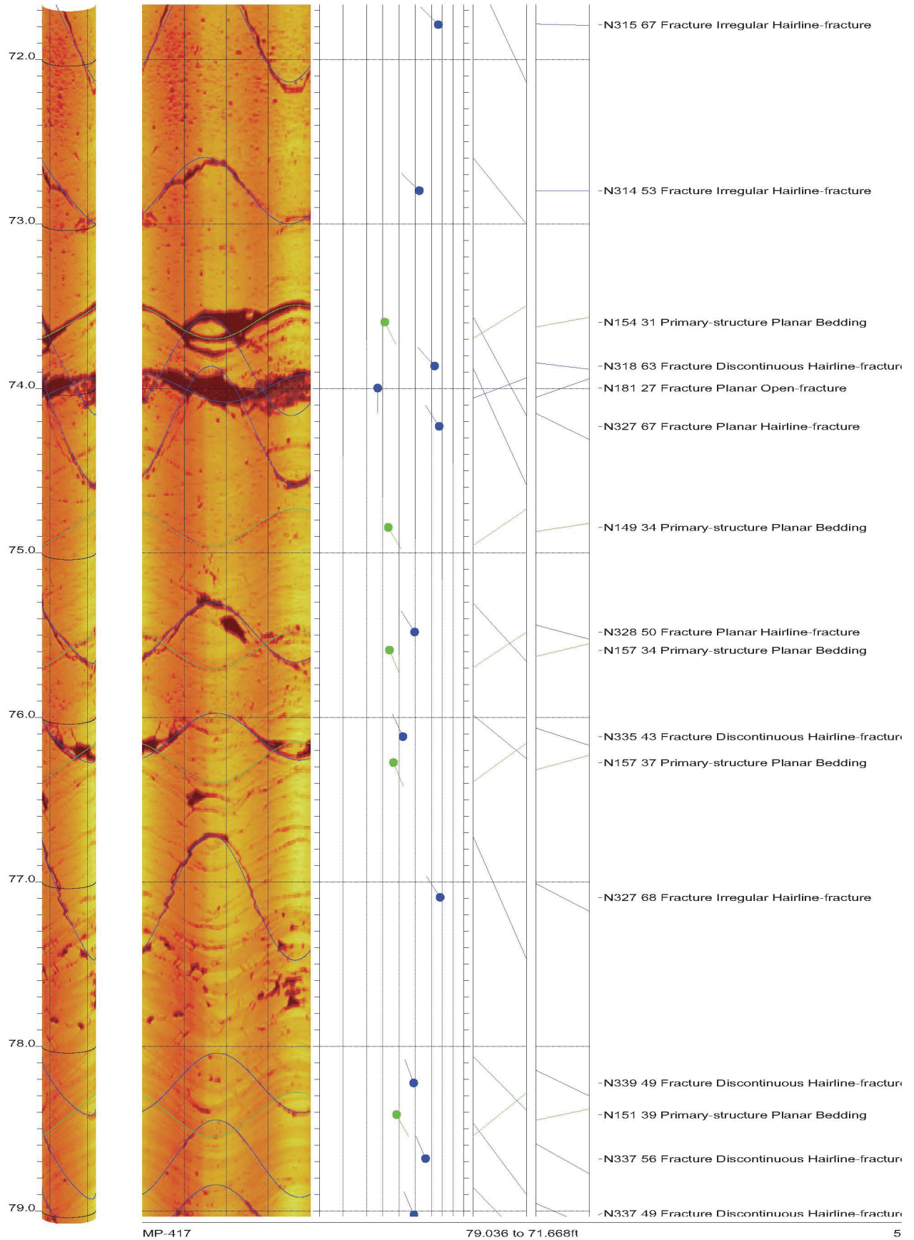
AMEC Clinch River SMR Project Borehole MP-417 Acoustic Televiewer Features rev 2 Sheet 5 of 38
