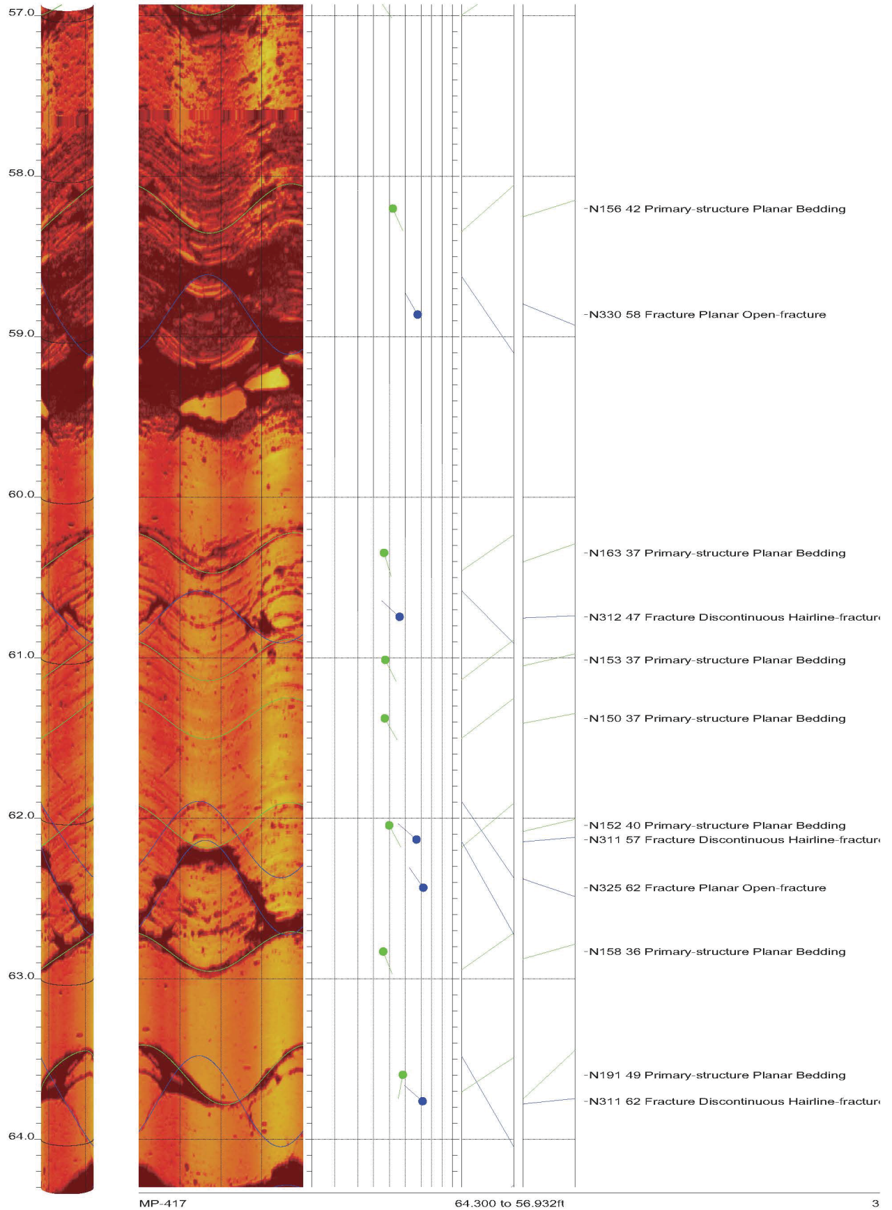
AMEC Clinch River SMR Project Borehole MP-417 Acoustic Televiewer Features rev 2 Sheet 3 of 38
