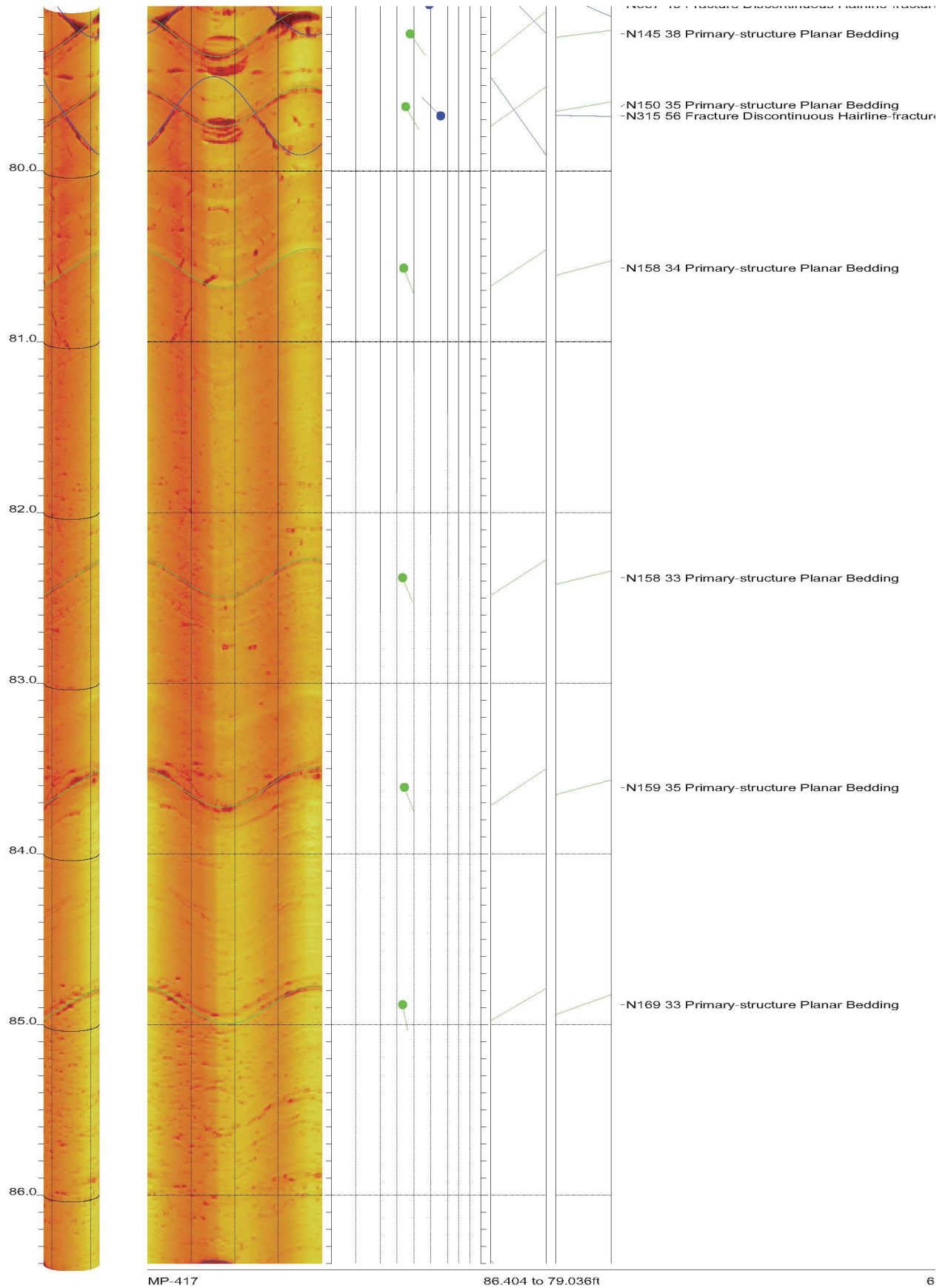
AMEC Clinch River SMR Project Borehole MP-417 Acoustic Televiewer Features rev 2 Sheet 6 of 38
