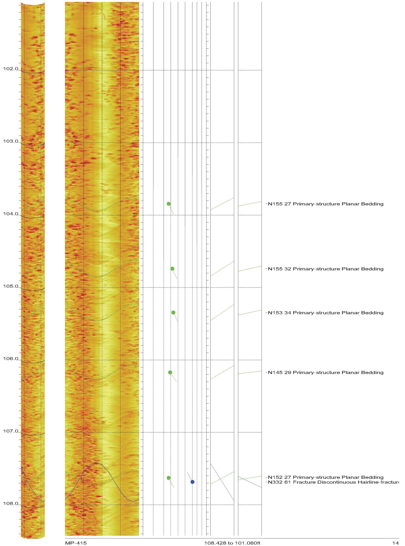
AMEC Clinch River SMR Project Borehole MP-415 Acoustic Televiewer Features rev 2 Sheet 14 of 42
