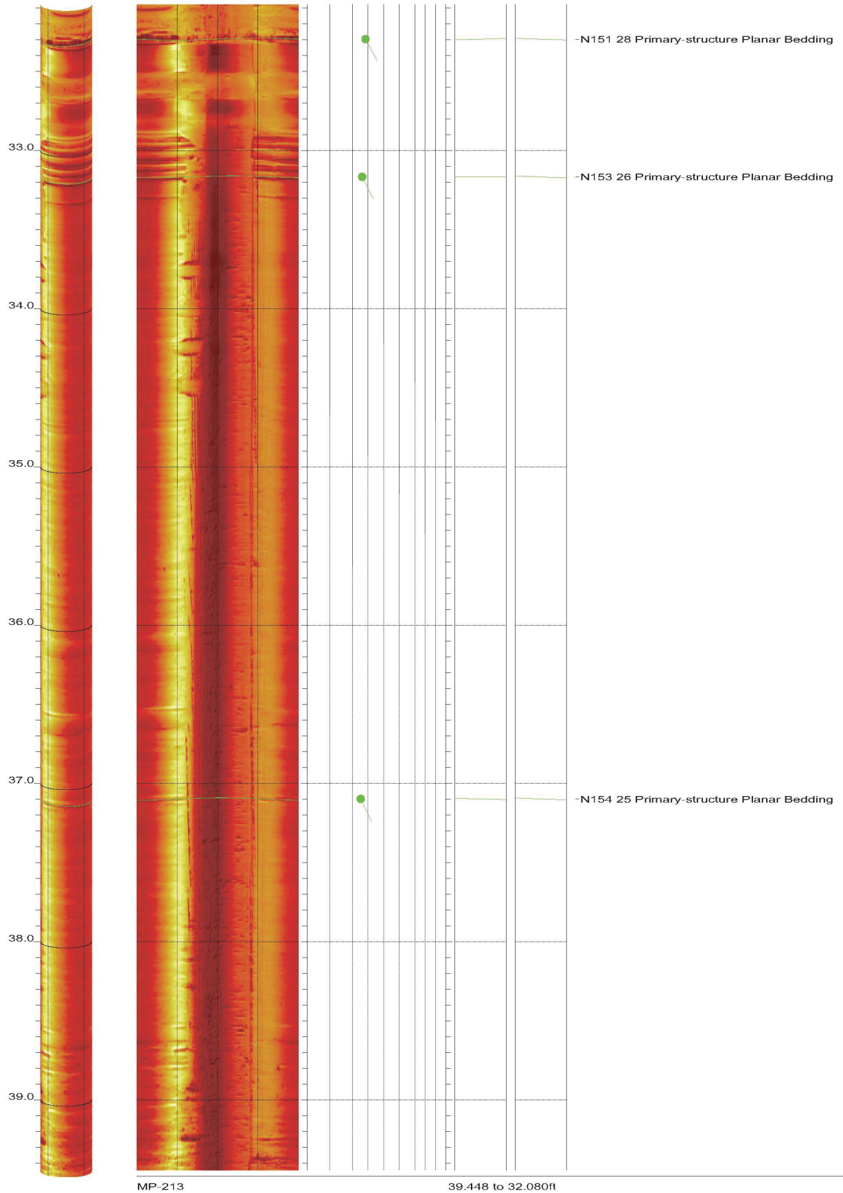
AMEC Clinch River SMR Project Borehole MP-213 Acoustic Televiewer Features rev 2 Sheet 4 of 23
