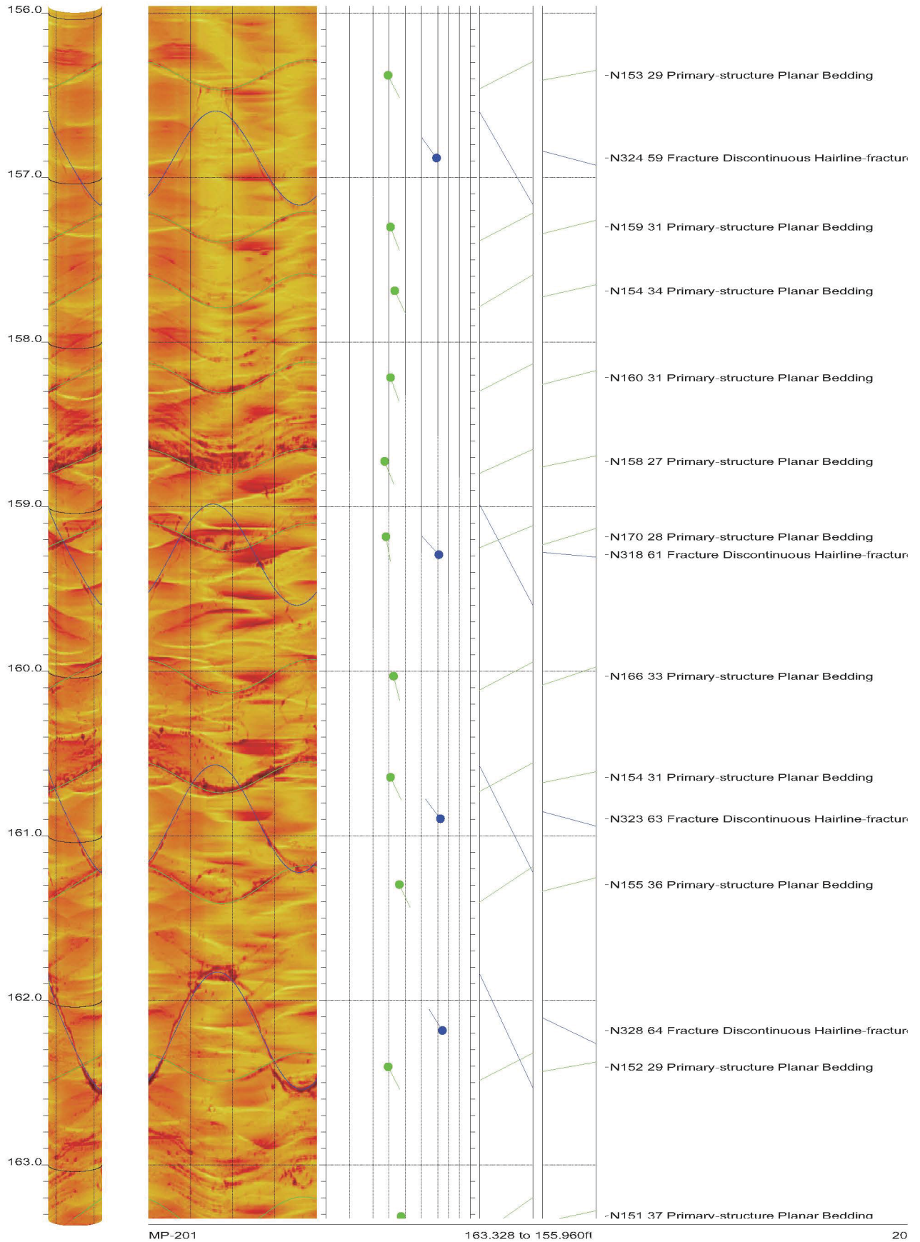
AMEC Clinch River SMR Project Borehole MP-201 Acoustic Televiewer Features rev 2 Sheet 20 of 55
