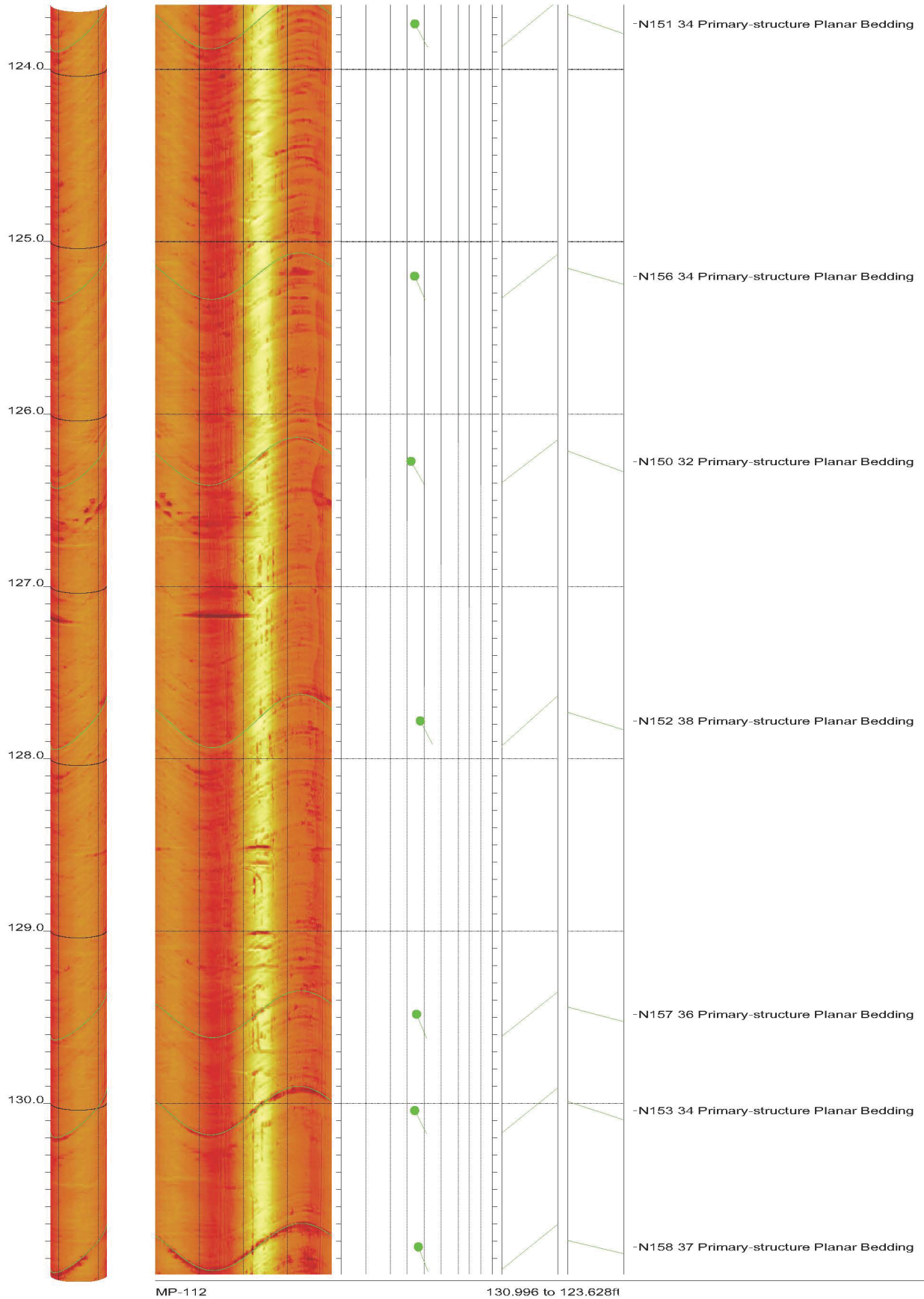
AMEC Clinch River SMR Project Borehole MP-112 Acoustic Televiewer Features rev 2 Sheet 15 of 22
