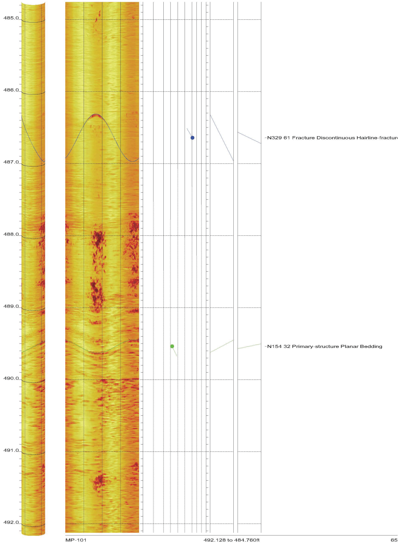
AMEC Clinch River SMR Project Borehole MP-101 Acoustic Televiewer Features rev 2 Sheet 65 of 72
