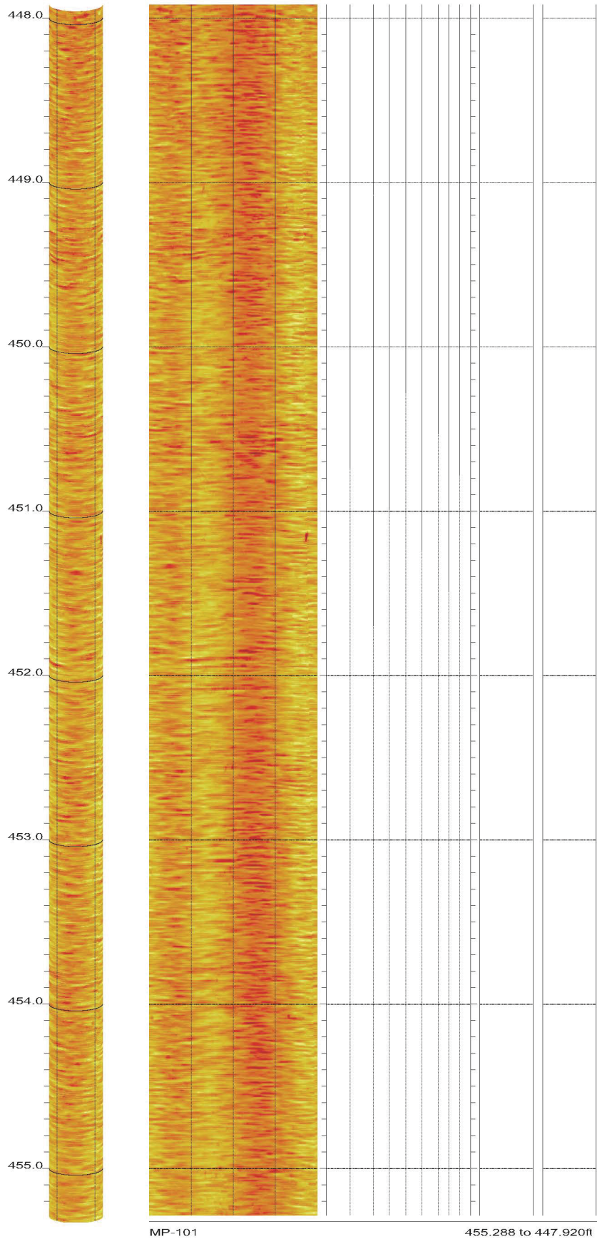
AMEC Clinch River SMR Project Borehole MP-101 Acoustic Televiewer Features rev 2 Sheet 60 of 72
