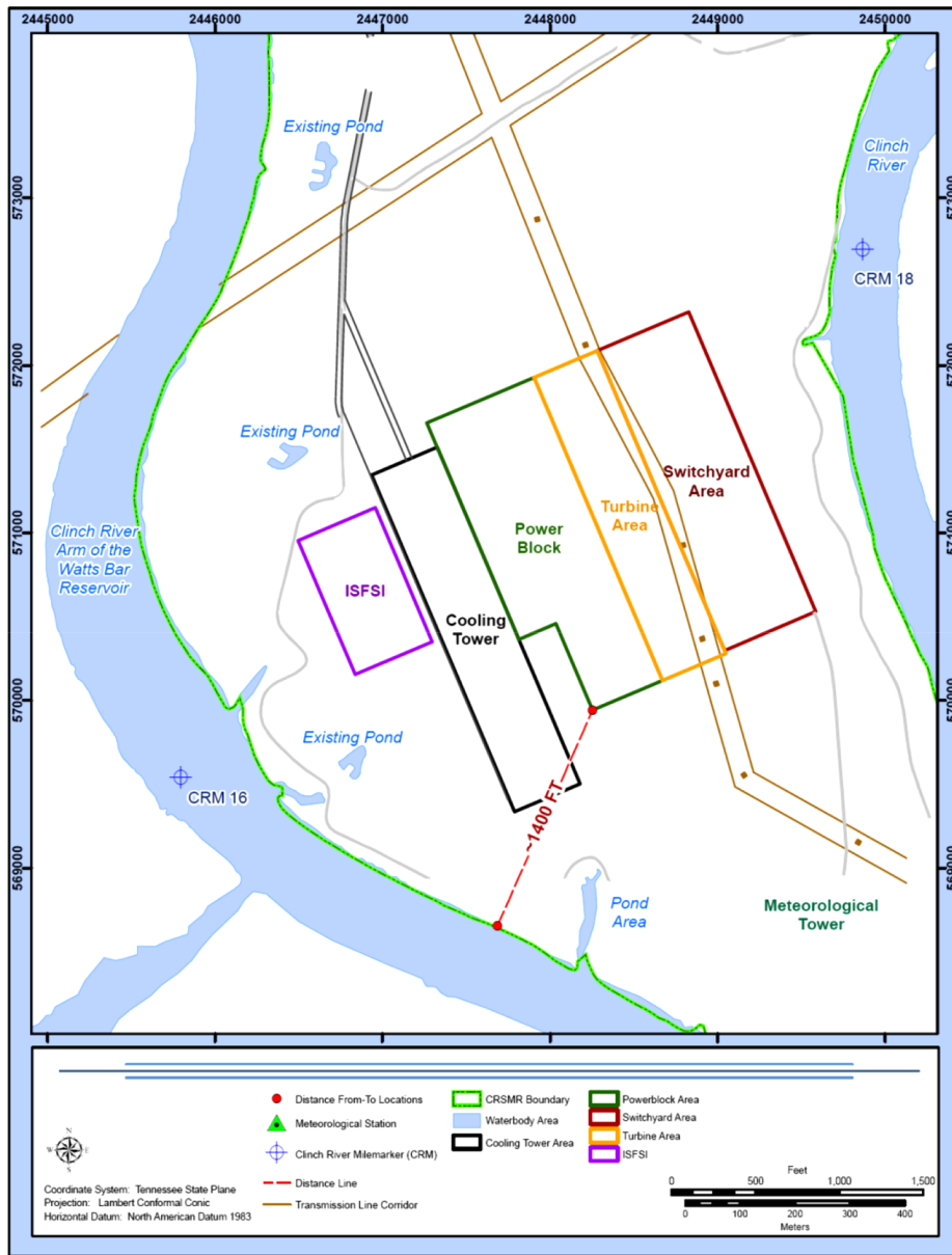
Figure 2.4.13-1. Minimum Distance from the Power Block Area to the Clinch River Arm of the Watts Bar Reservoir
