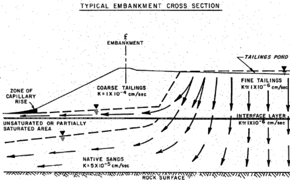
Figure 27: Snapshot of Figure 28 D'Appolonia (1980) showing schematic of cross-section through the large tailings pile embankment.
