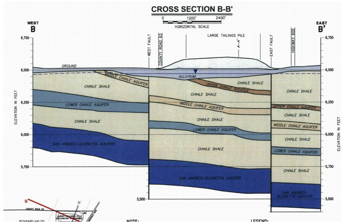
Figure 12: Snapshot of Figure 3.1-6 (HMC 2012) showing cross section B-B'. See Figure 10 for location.
