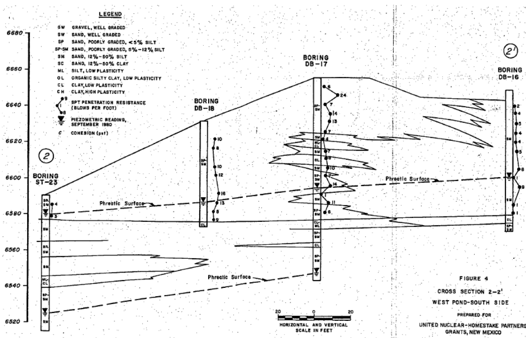
Figure 26: Snapshot of Figure 4, D'appolonia (1980) showing a cross-section through the south side of the west pond of the large tailings pile
