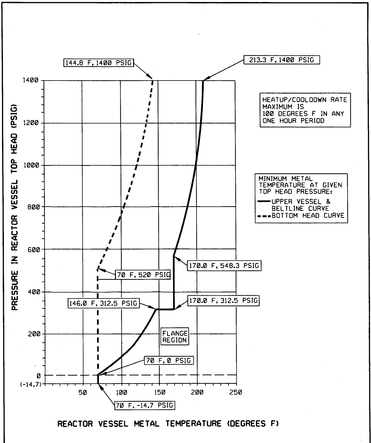
FIGURE 3.4.11-1(c): CORE CRITICAL OPERATION CURVES (VALID UP TO 32 EFPY)
