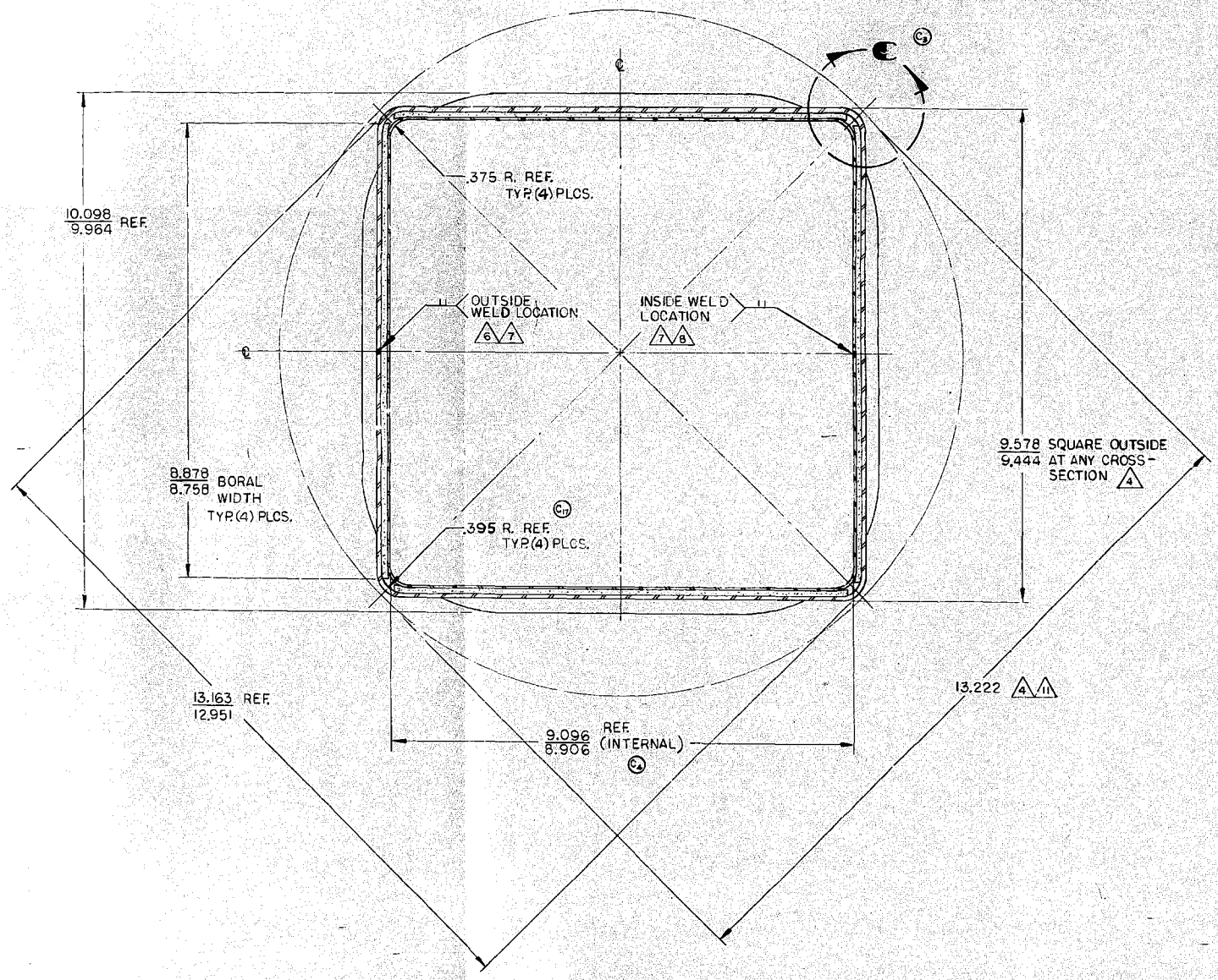
SECTION B-B SCALE 1/1
