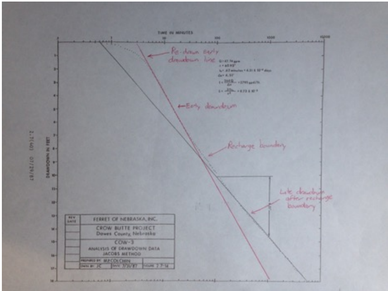
Kreamer Testimony September 2015 Exhibit 3. Cooper Jacob semi-logarithmic plot (Figure 2.7 -14) modified (in red) to show early drawdown. A recharge boundary appears at approximately 30 minutes, and forms a line of late time data to the right of the red early data trend.
