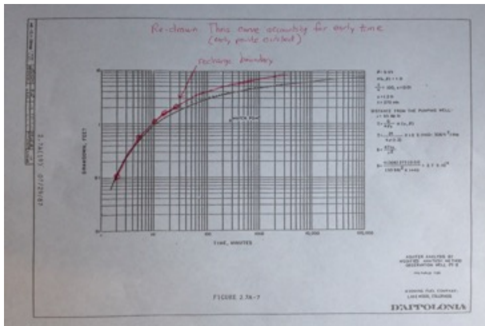
Kreamer Testimony September 2015 Exhibit 2. Re-drawn Figure 2.7A-7, with This type-curve matching early time in red. Early data points are circled – late time data below type curve indicates recharge.
