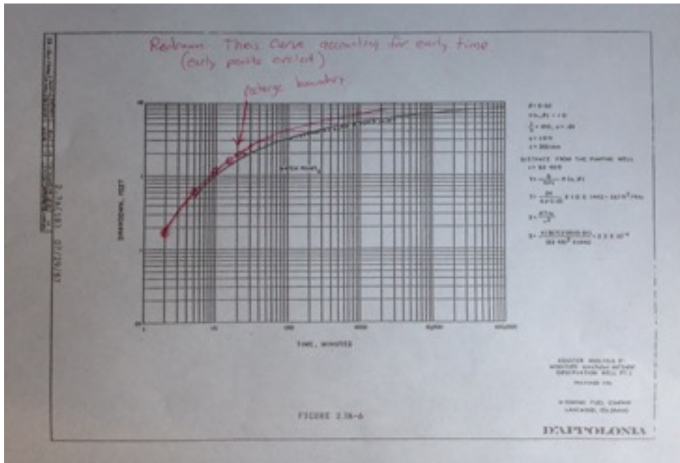
Kreamer Testimony September 2015 Exhibit 1. Re-drawn Figure 2.7A-6, with This type-curve matching early time in red. Early data points are circled – late time data below type curve indicates recharge.
