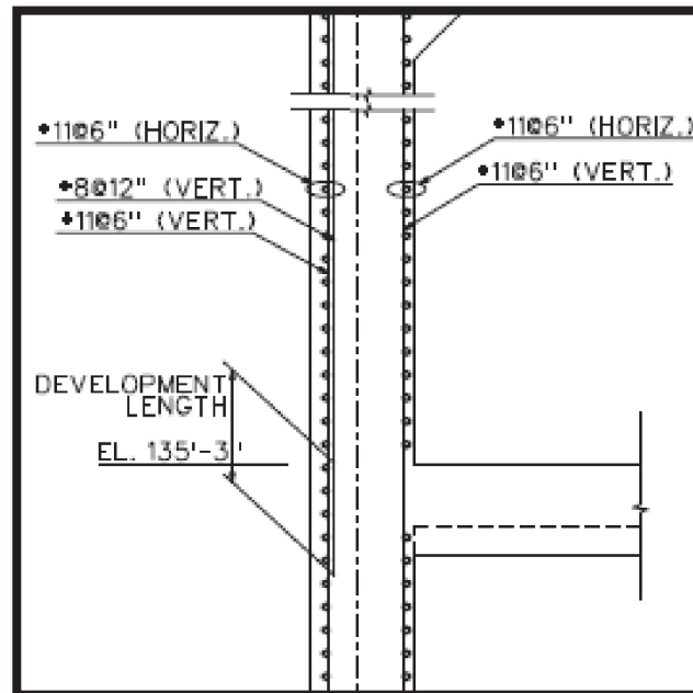
Figure 3H.5-3 [Typical Reinforcement in Wall on Column Line 1]*
