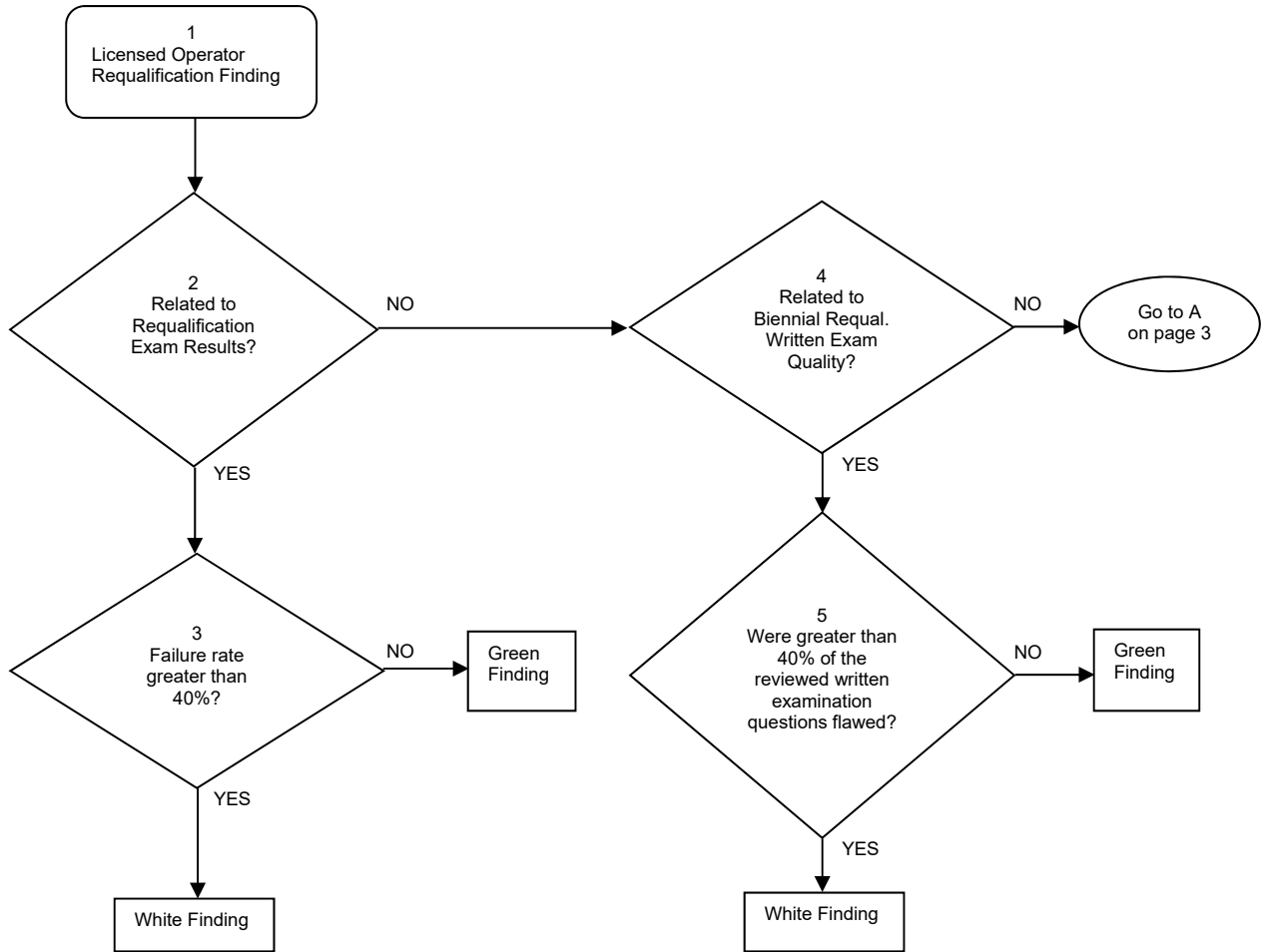
Figure I.1 – Licensed Operator Requalification SDP Flowchart
