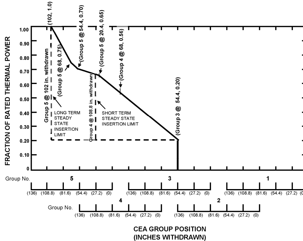
CEA GROUP POSITION (INCHES WITHDRAWN) FIGURE 3.1-2 CEA Group Insertion Limits vs. THERMAL POWER
