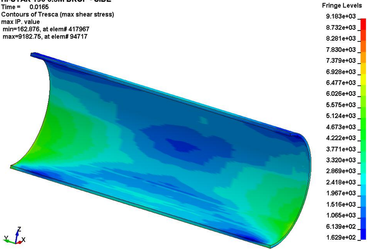
Figure 2.6.5: Maximum Shear (1/2 Times Stress Intensity) Distribution in Containment Shell for Load Combination N2 (1-Ft Side Drop)
