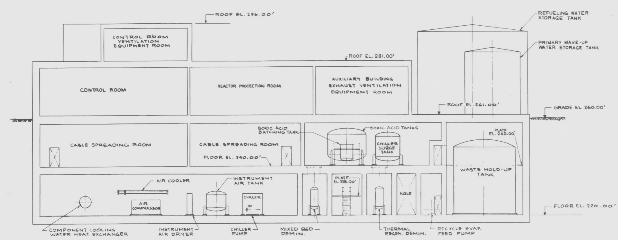
SECTION B-B
