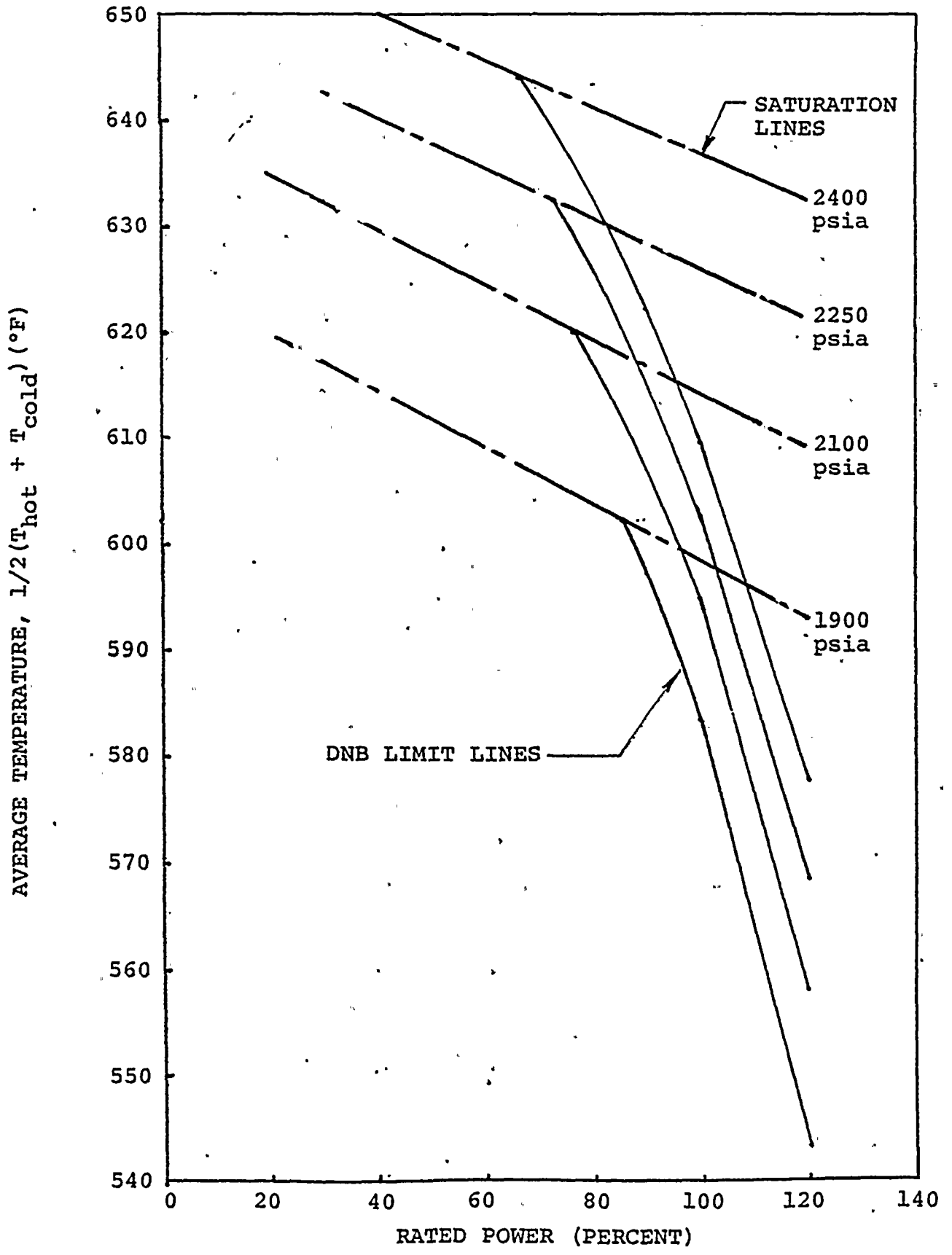
Figure 2 Reactor Core Thermal and Hydraulic Safety Limits
