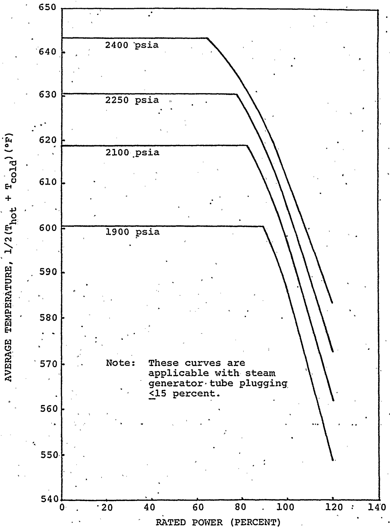
Figure 2.1-1. Reactor Core Thermal and Hydraulic Safety Limits, 3 Loop Operation
