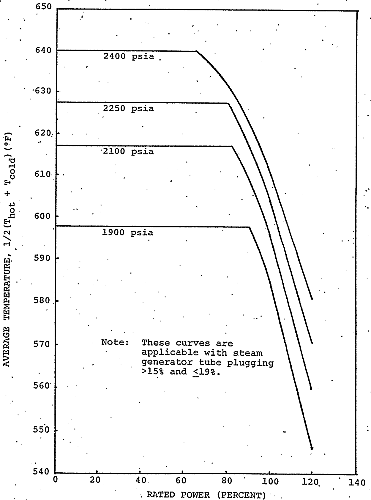
Figure 2.1-1a. Reactor Core Thermal and Hydraulic Safety Limits, 3-Loop Operation
