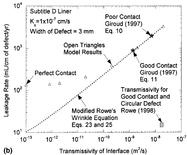
FIG. 9. Leakage Rates through Defective Seams in Composite Liners Having Imperfect Contact: (a) GCL Composite Liner; (b) Subtitle D Liner
