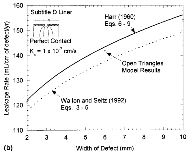
FIG. 4. Leakage Rates through Defective Seams in Composite Liners Having Perfect Contact: (a) GCL Composite Liner; (b) Subtitle D Liner
