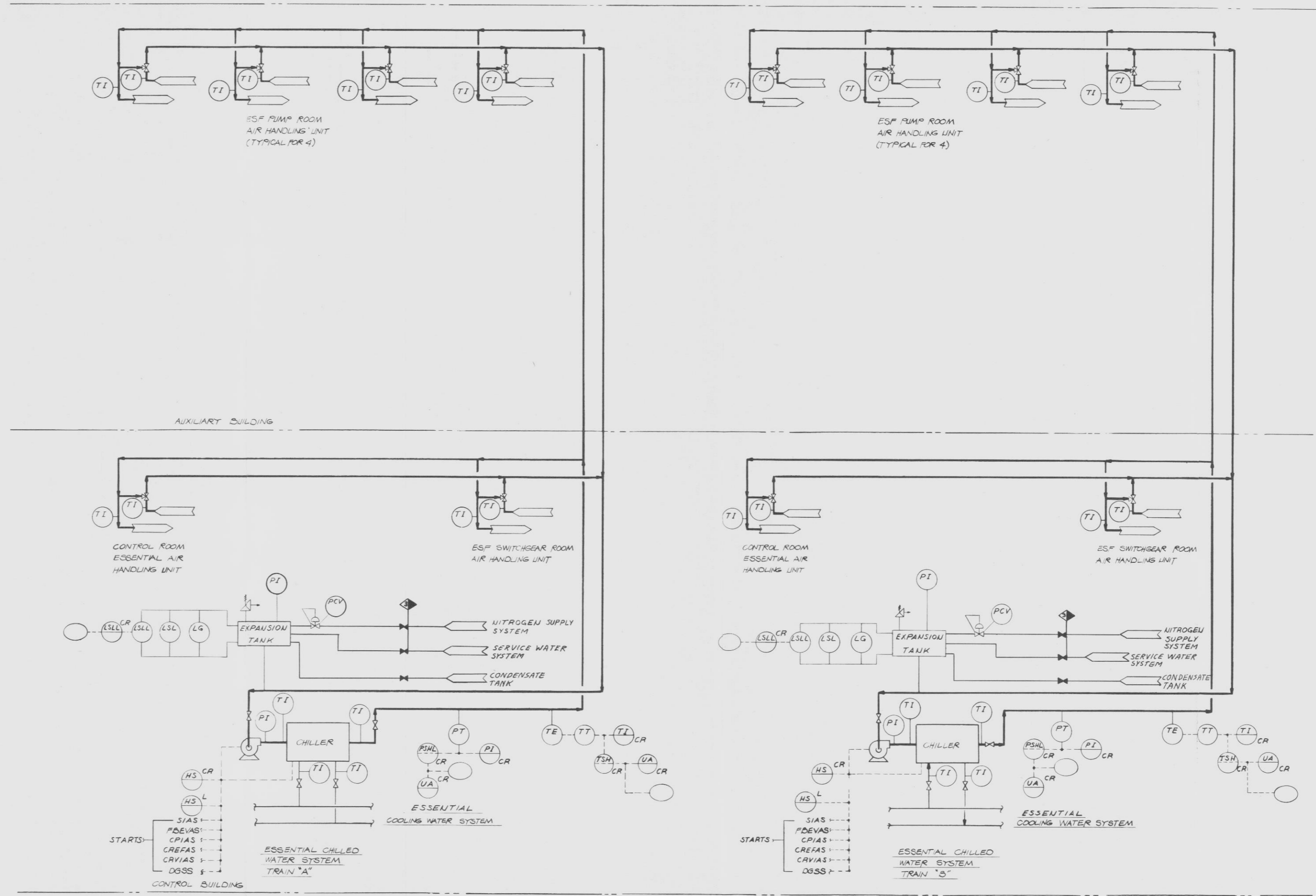
Arizona Nuclear Power Project Palo Verde Nuclear Generating Station Units 1, 2 & 3 ESSENTIAL CHILLED WATER SYSTEM Figure 9.2-11
