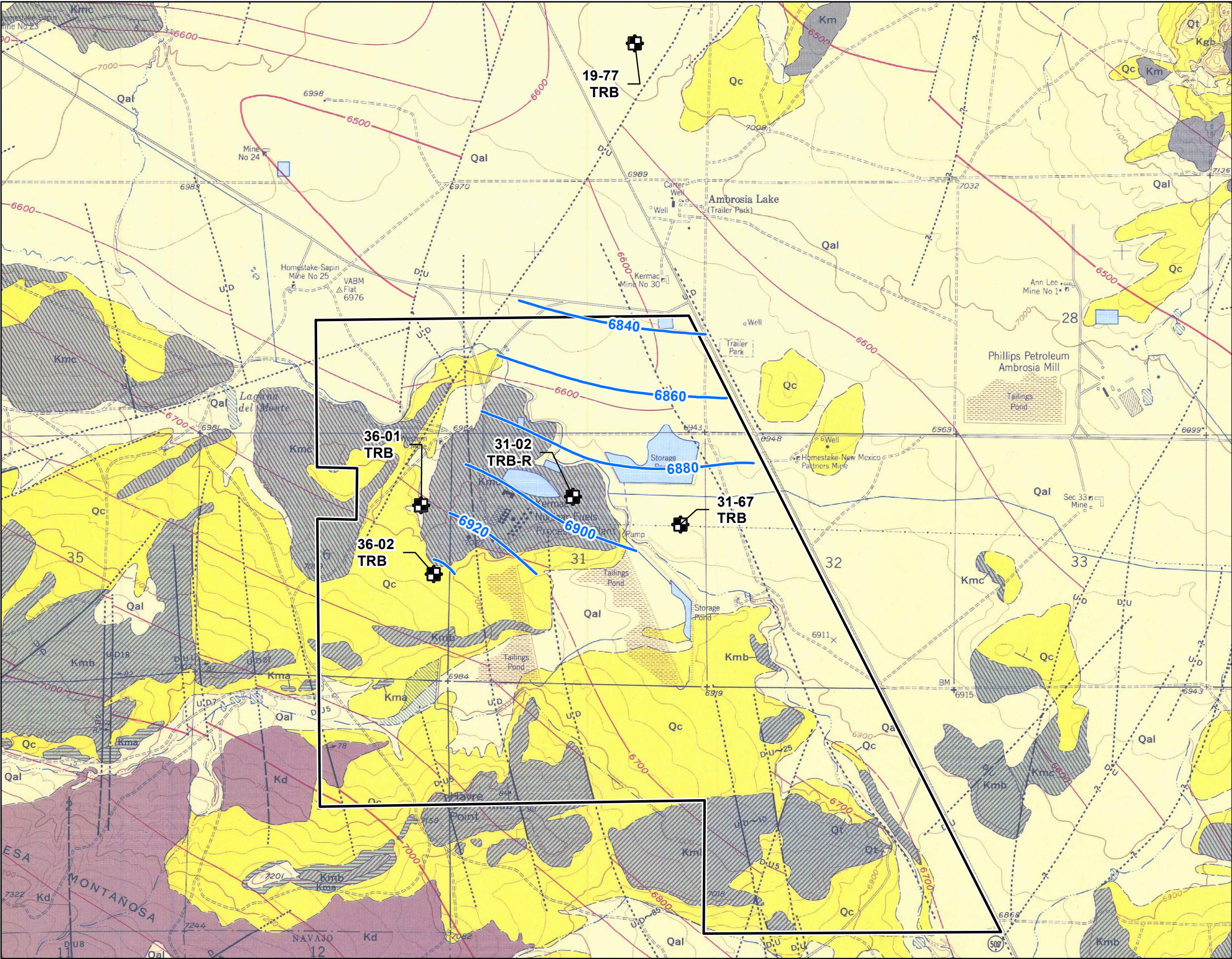
Figure 2 Tres Hermanos B Potentiometric Surface Contours Rio Algom Mining LLC, 2017 ACL Workplan: Response to Comments
