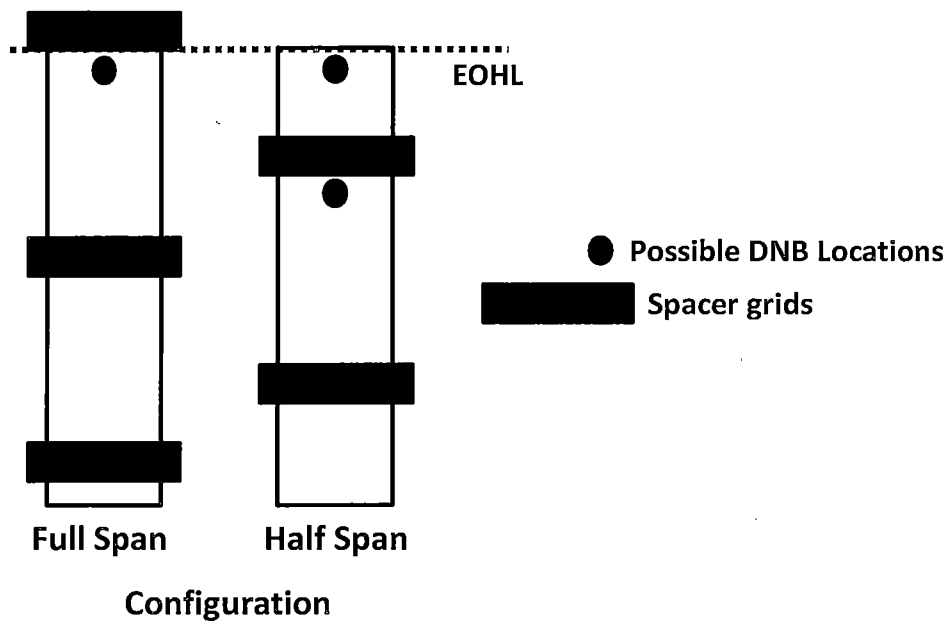
Figure 1-1 "Half-span" vs. "full-span" CHF test configurations
