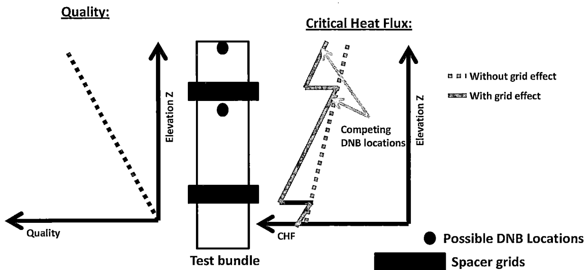
Figure 1-2 "Half-span" vs. "full-span" CHF detection locations
