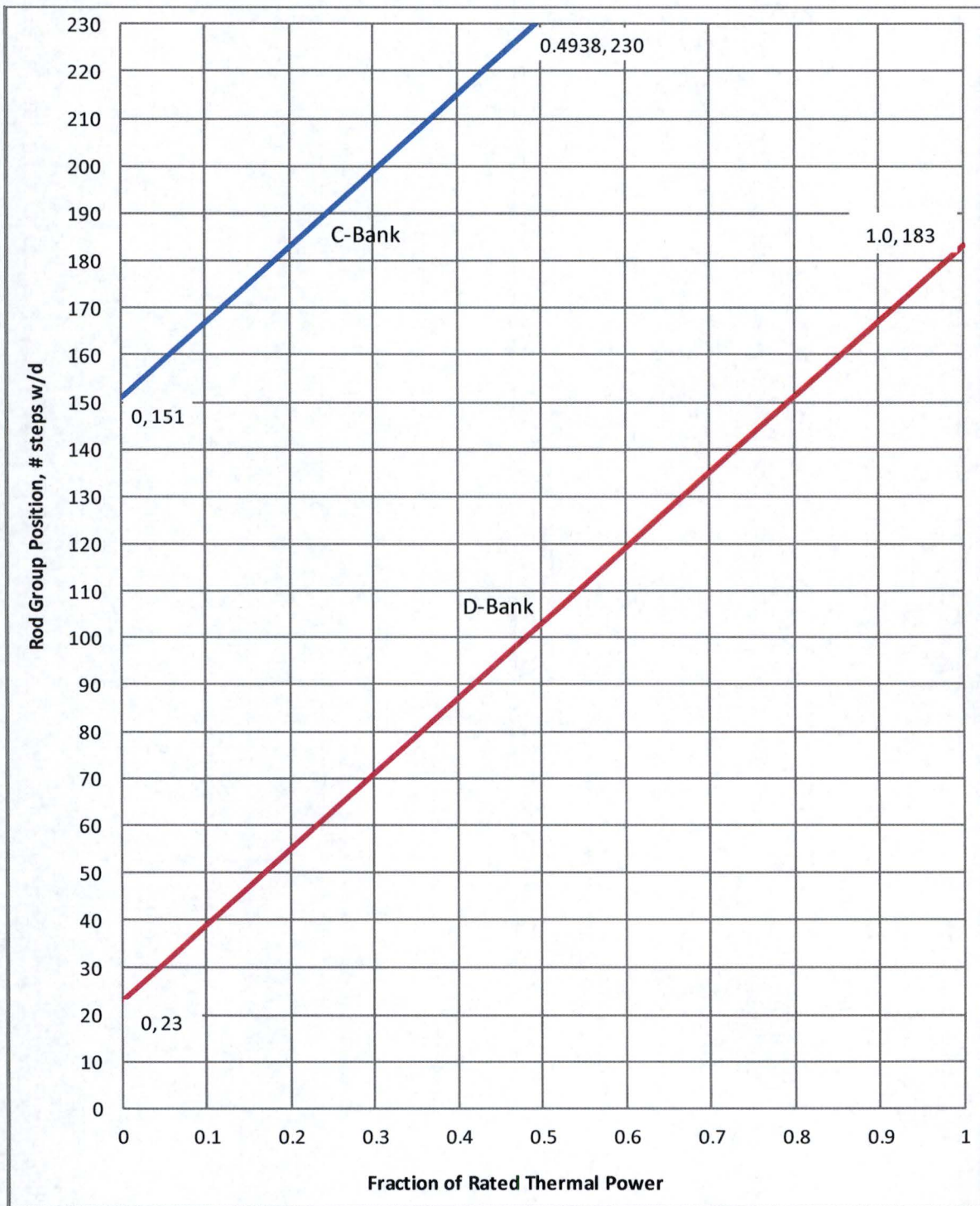
Figure A-2 Surry 1 Cycle 29 Rod Group Insertion Limits Max w/d position =230 steps
