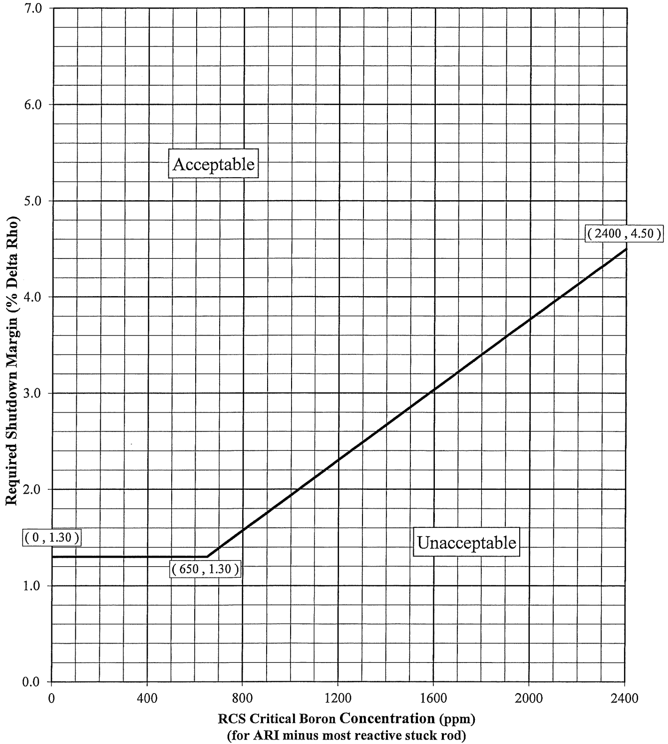
Required Shutdown Margin for Mode 5
