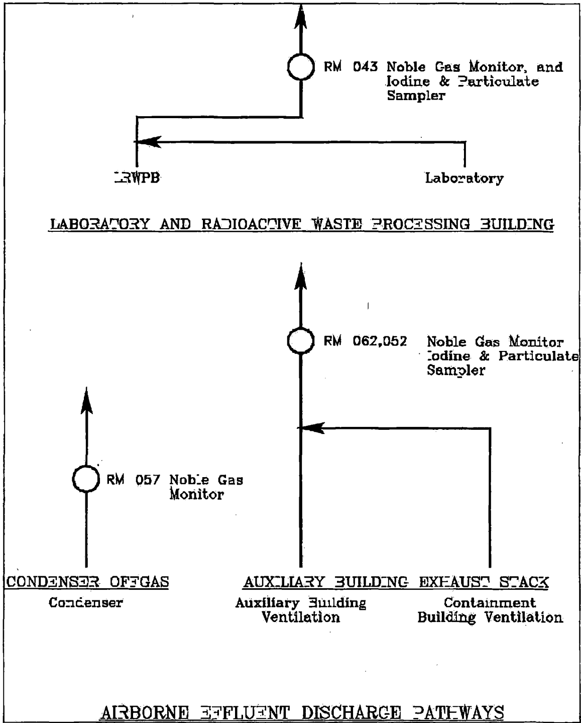
Figure 4 - Airborne Effluent Discharge Pathways
