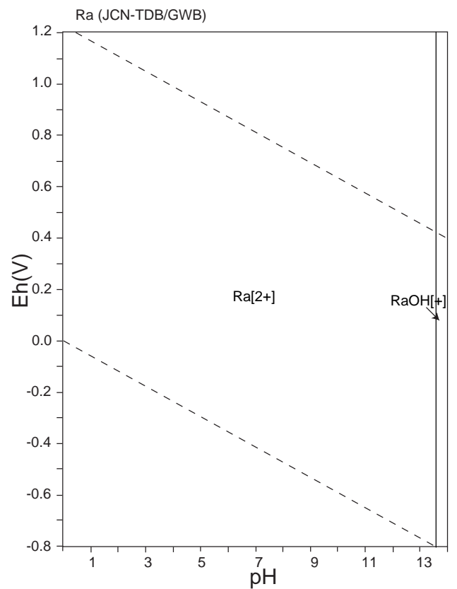
Figure 99: Eh-pH diagrams of the system Ra-O-H (1). \sum \text{Ra} = 10^{-10} , 298.15K, 10^5 Pa.
