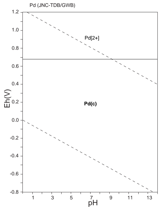
Figure 92: Eh-pH diagrams of the system Pd-O-H. \sum \text{Pd} = 10^{-10} , 298.15K, 10^5 Pa.
