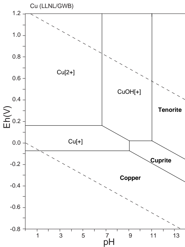
Figure 39: Eh-pH diagrams of the system Cu-O-H (1). \Sigma \text{Cu} = 10^{-10} , 298.15K, 10^5 Pa.
