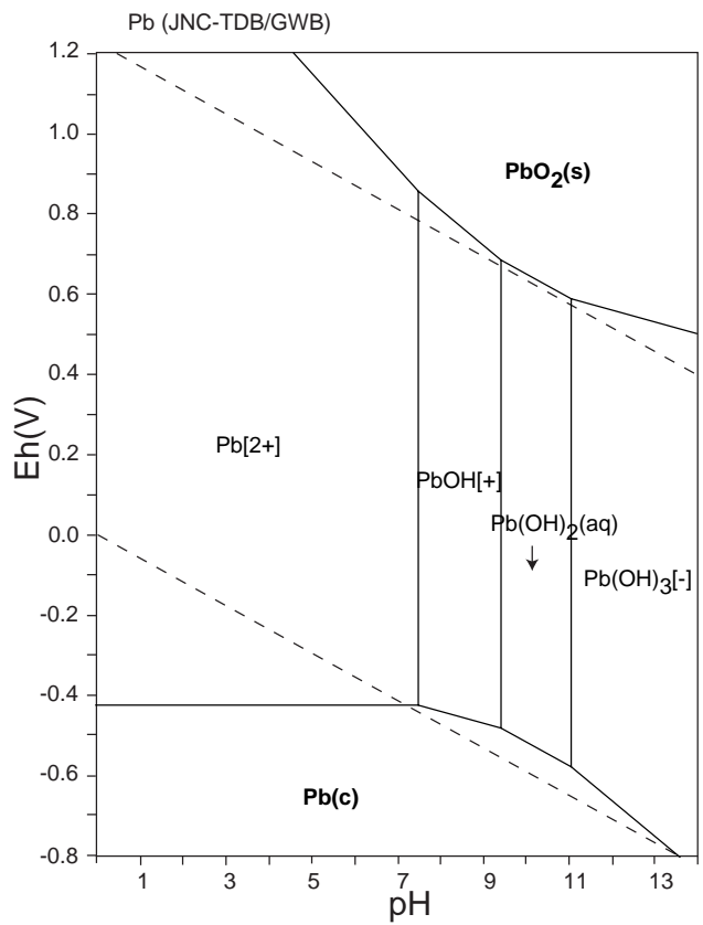
Figure 90: Eh-pH diagrams of the system Pb-O-H (1). \Sigma \text{Pb} = 10^{-10} , 298.15K, 10^5 Pa.
