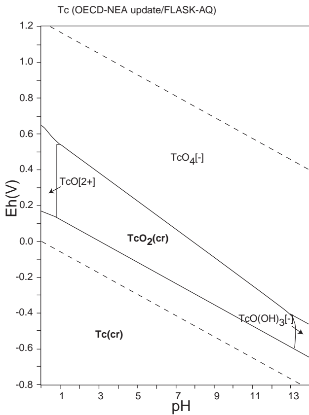
Figure 123: Eh-pH diagrams of the system Tc-O-H (2). \sum \text{Tc} = 10^{-10} , 298.15K, 10^5 Pa.
