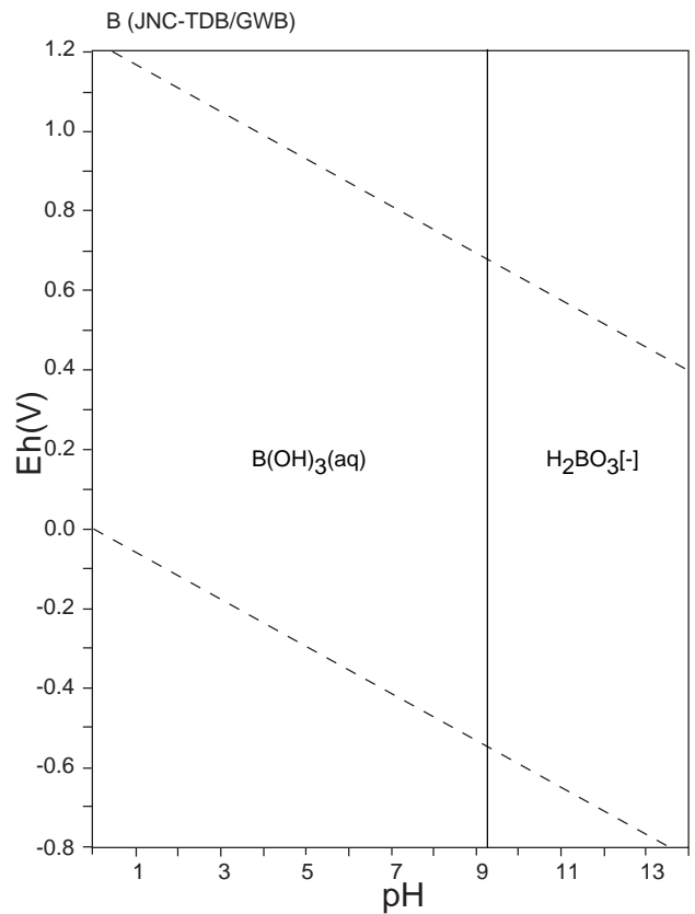
Figure 14: Eh-pH diagrams of the system B-O-H (1). \Sigma \text{B} = 10^{-10} , 298.15K, 10^5 Pa.
