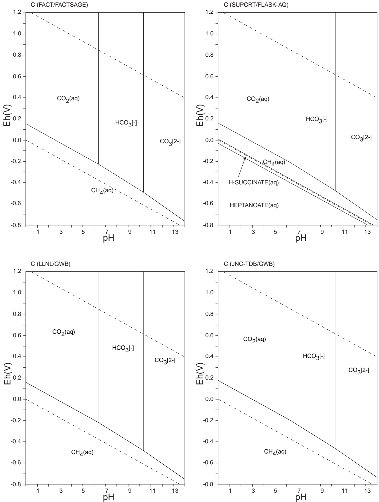
Figure 22: Eh-pH diagrams of the system C-O-H (1). \Sigma \text{C} = 10^{-10} , 298.15K, 10^5 Pa.
