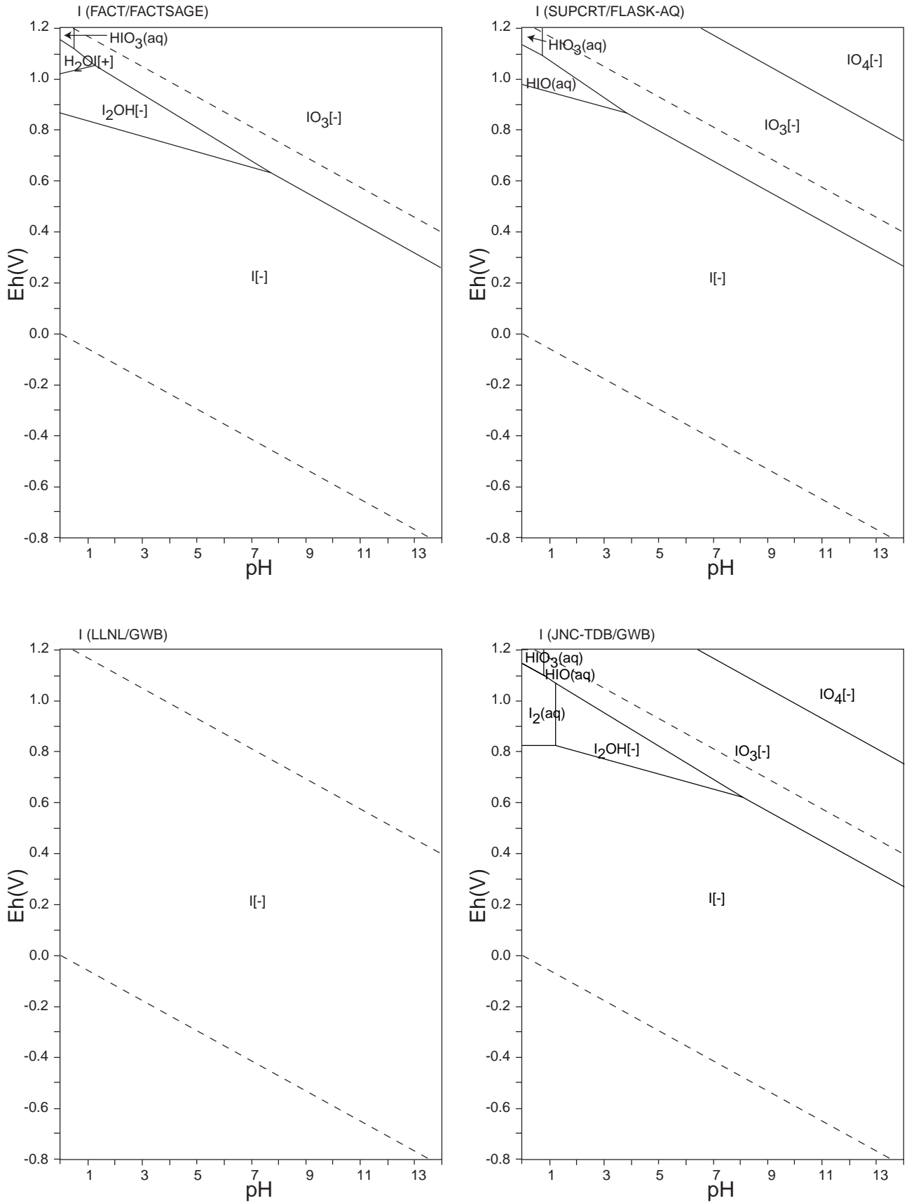
Figure 57: Eh-pH diagrams of the system I-O-H (1). \sum \text{I} = 10^{-10} , 298.15K, 10^5 Pa.
