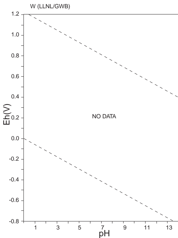
Figure 133: Eh-pH diagrams of the system W-O-H. \Sigma W = 10^{-10} , 298.15K, 10^5 Pa.
