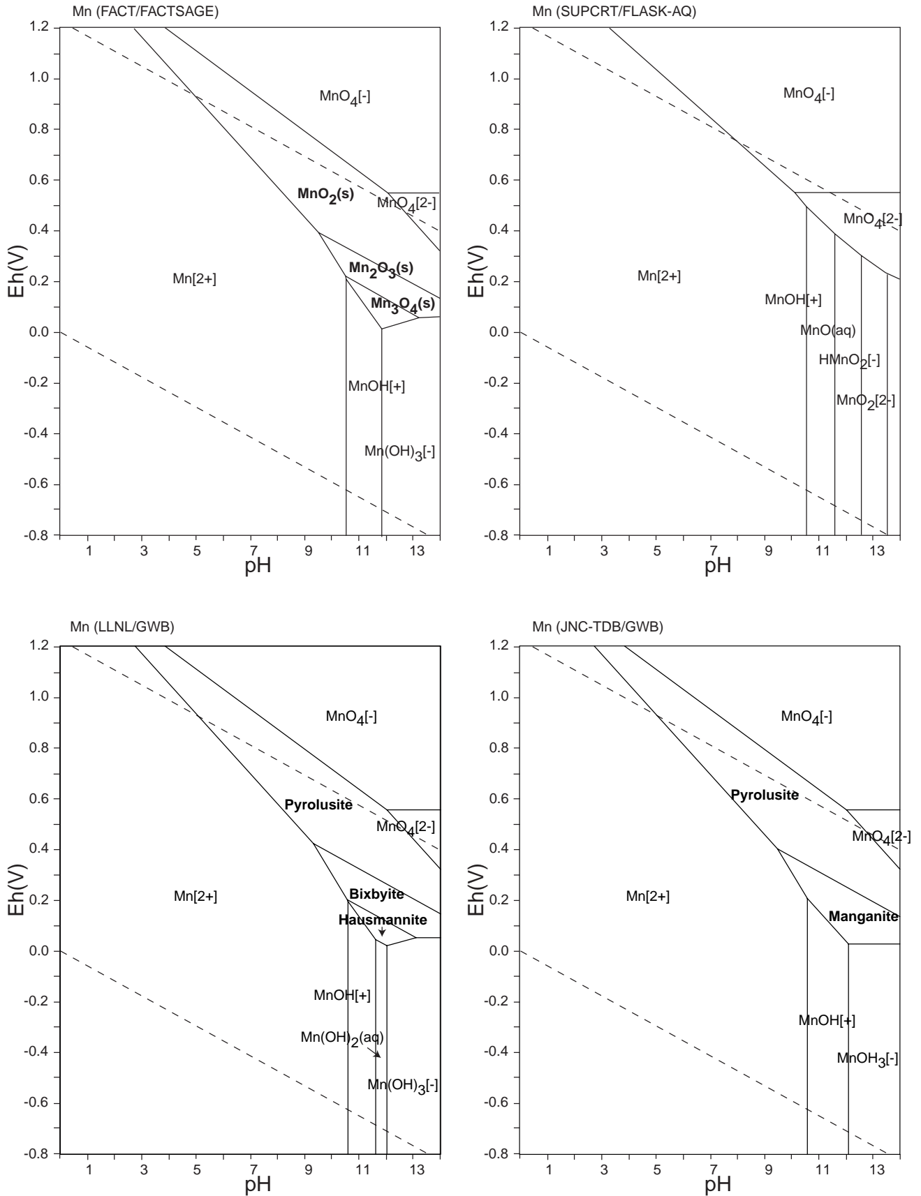
Figure 69: Eh-pH diagrams of the system Mn-O-H (1). \Sigma \text{Mn} = 10^{-10} , 298.15K, 10^5 Pa.
