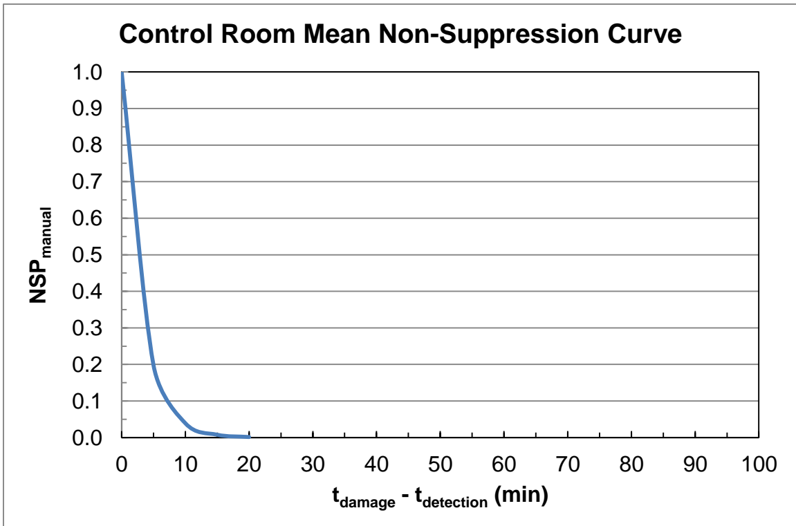
Figure A7.11 Control Room Mean Non-Suppression Curve
