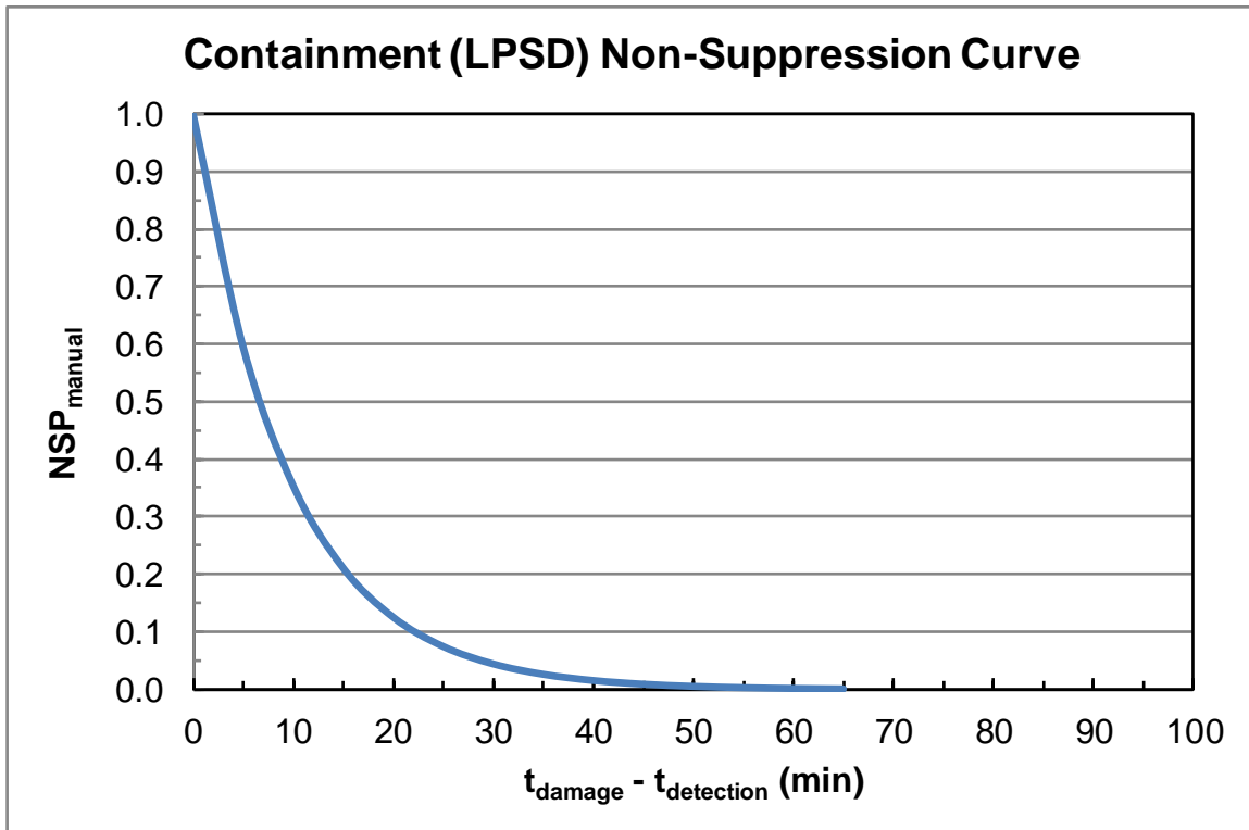
Figure A7.9 Containment (LPSD) Non-Suppression Curve
