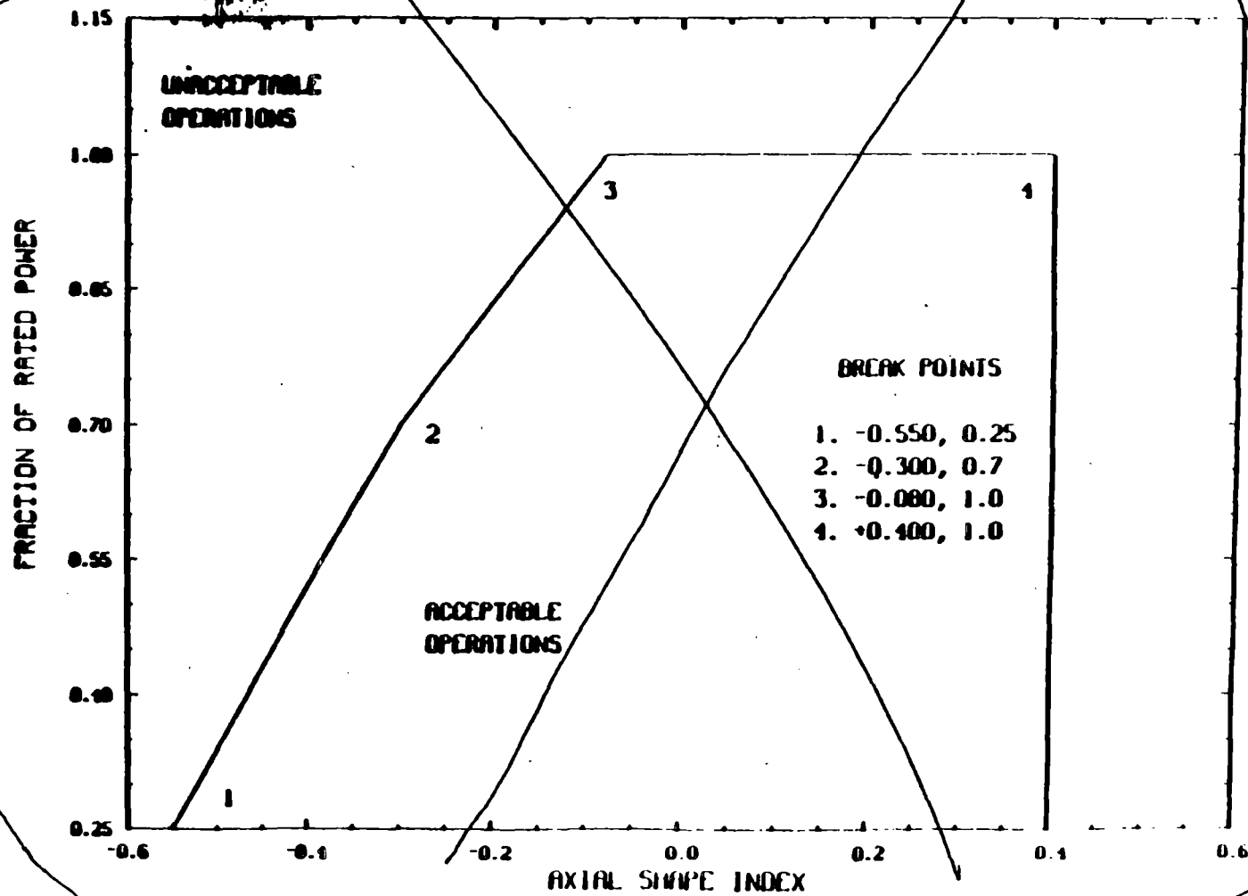
FIGURE 3-0 ASI LCD FOR Tinlet FUNCTION
